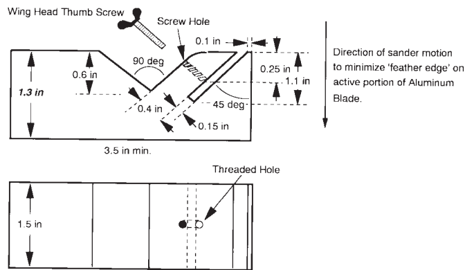
FIG. 27 Aluminum Blade Shaping Fixture
