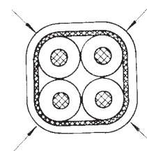
FIG. 11 Shielded and Jacketed Twisted Quad
