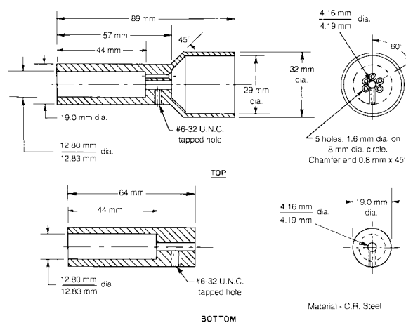
FIG. 1 Test Cell Loading Devices
