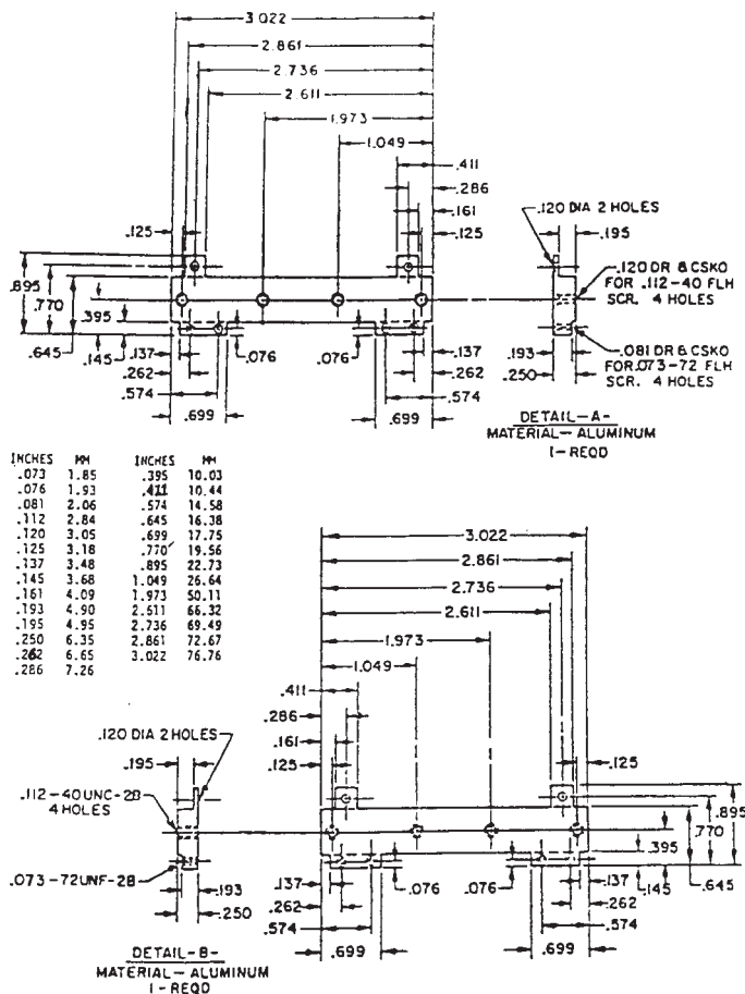
FIG. 6 Test Fixture Construction, Older Design (Fixture B)
