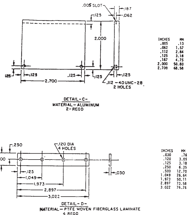
FIG. 7 Test Fixture Construction, Older Design (Fixture B)
