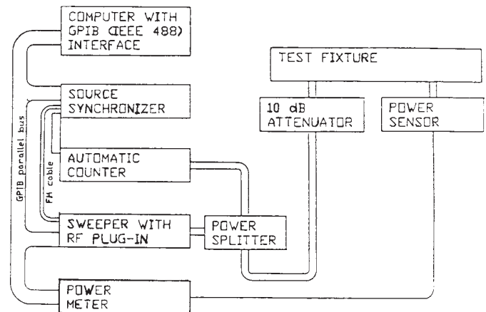
FIG. 17 Automated Permittivity Test Setup
