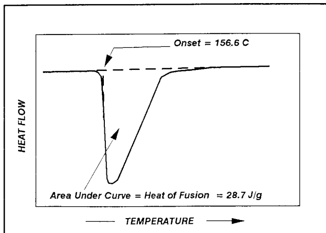
FIG. 1 Indium Calibration
