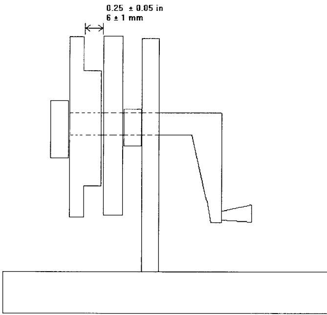
FIG. 1 Coil Winder
