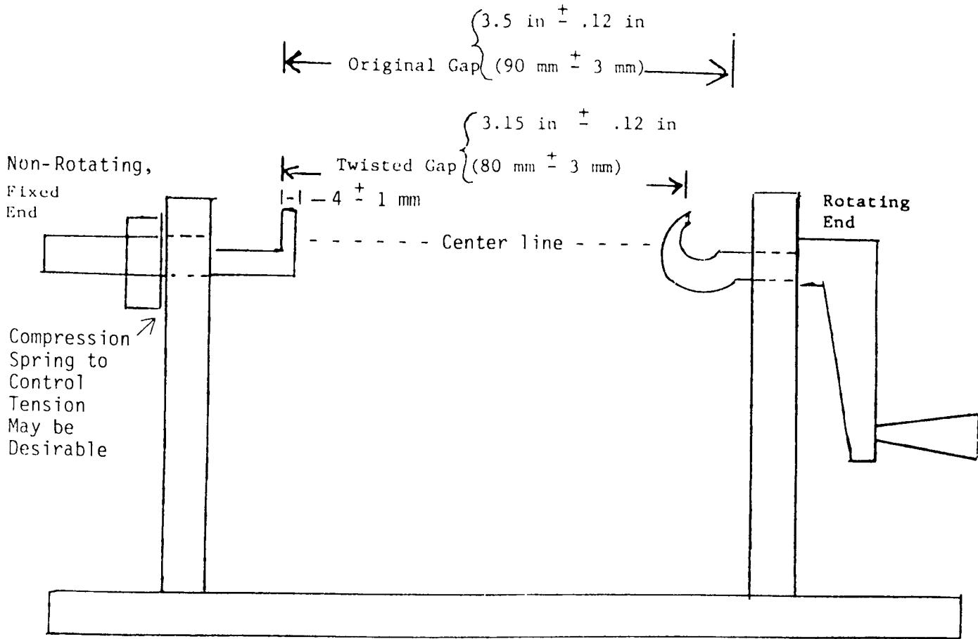
FIG. 3 Coil Twister
