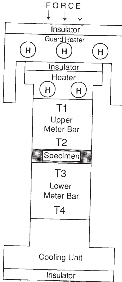
FIG. 2 Guarded Heater
