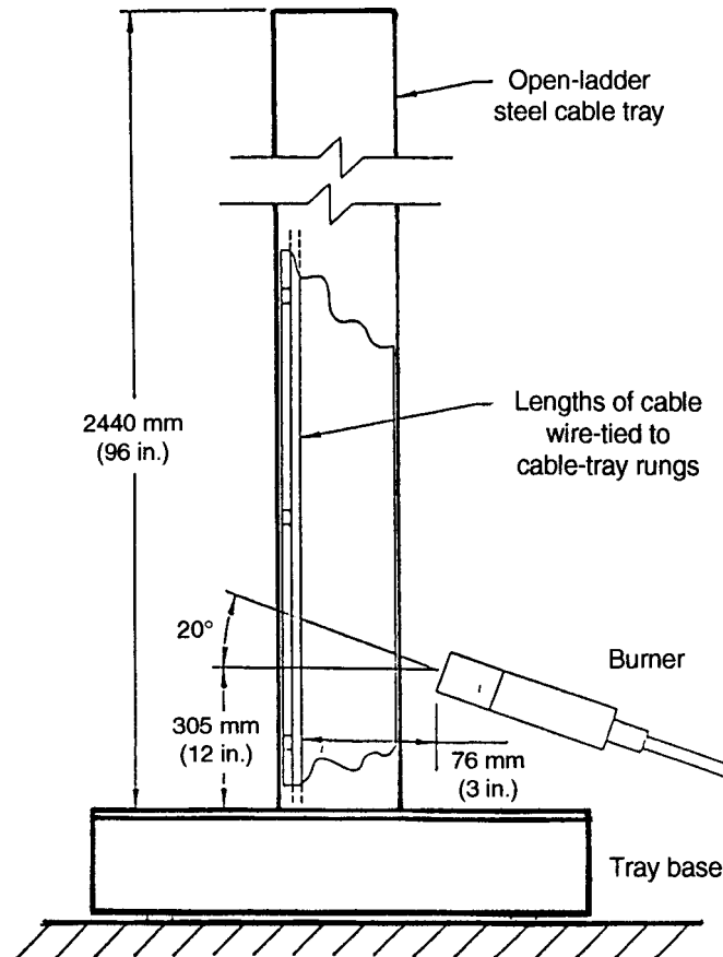
FIG. 6.8 Protocol B Cable Tray
