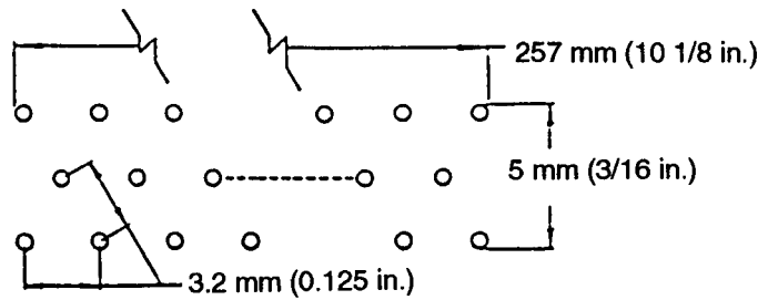
FIG. 5.7 Burner Holes
