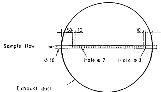
FIG. 4.6 Sampling Probe
