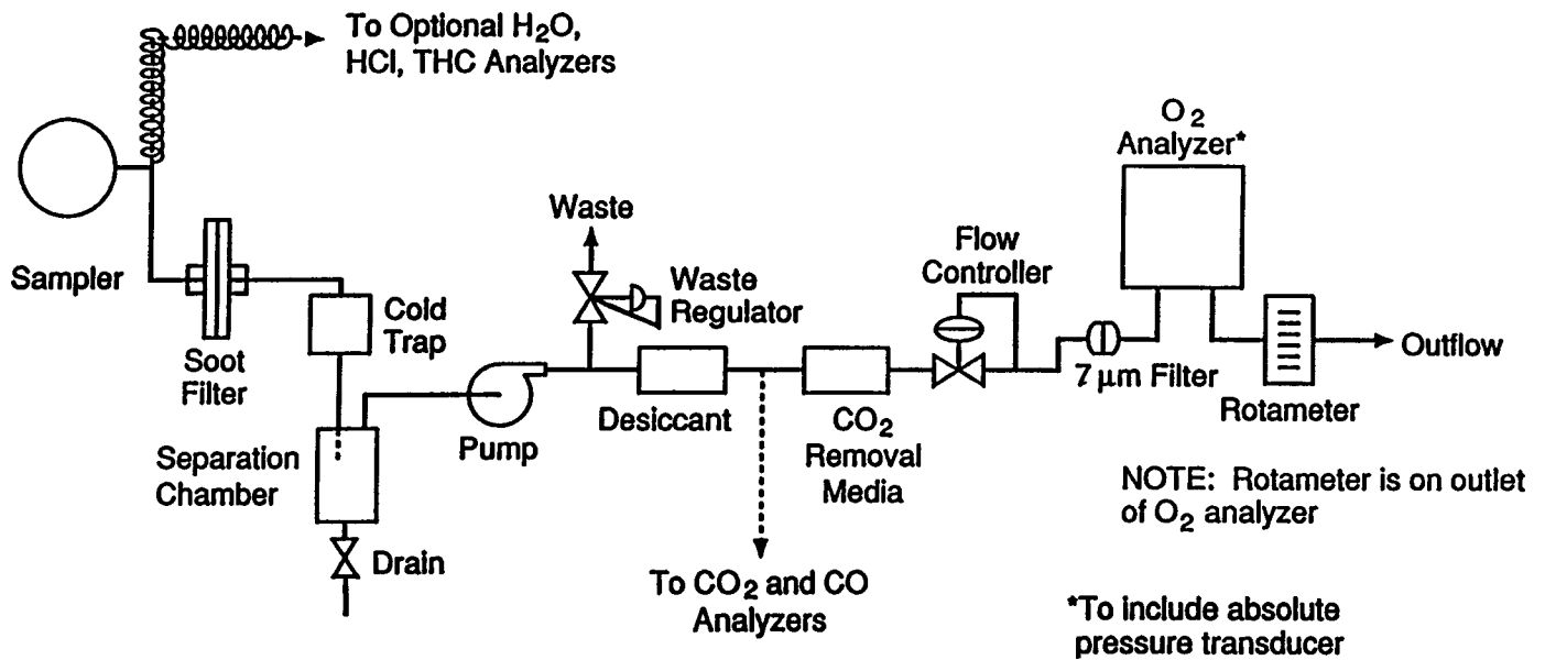
FIG. 3.5 Schematic Diagram of Gas Analysis System
