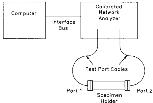
FIG. 1 Block Diagram of Experimental Setup
