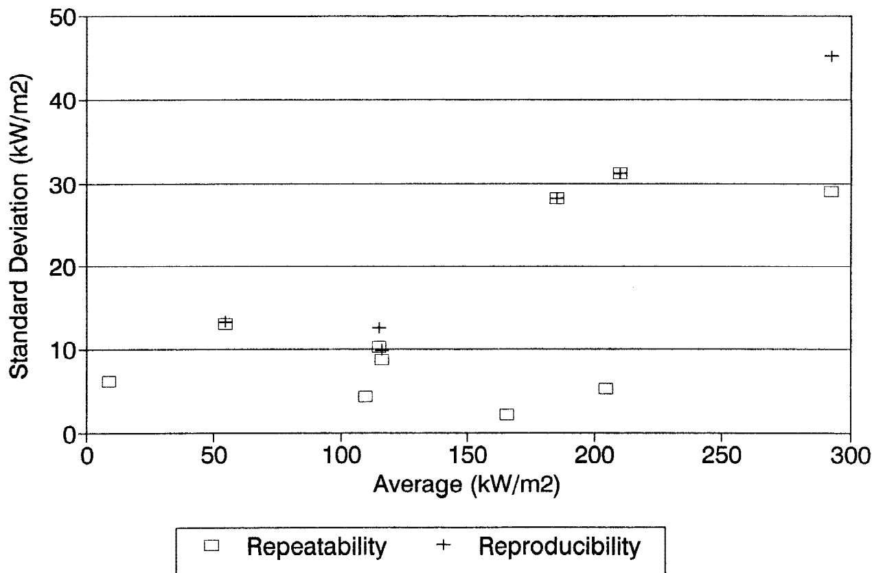
FIG. 3 Peak Heat Release Rate Precision
