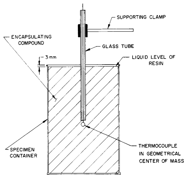
FIG. 1 Test Specimen for Exothermic Temperature
