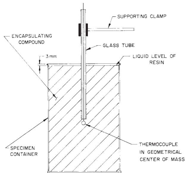
FIG. 1 Test Specimen for Exothermic Temperature
