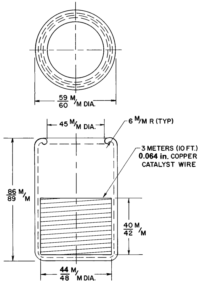
FIG. A1.2 Glass Sample Container with Catalyst
