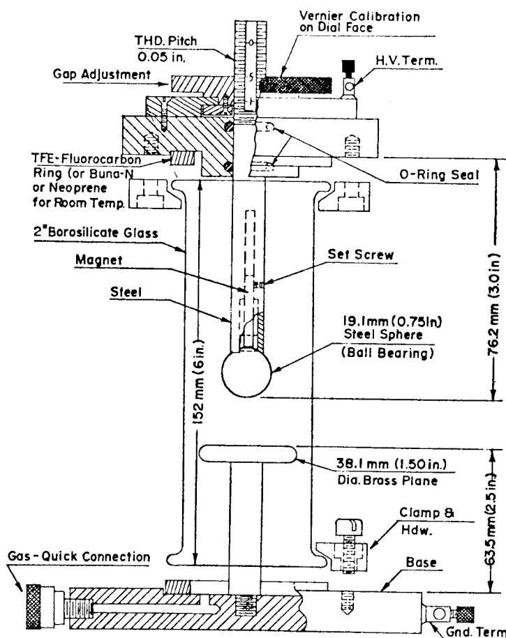
FIG. 1 Test Cell
