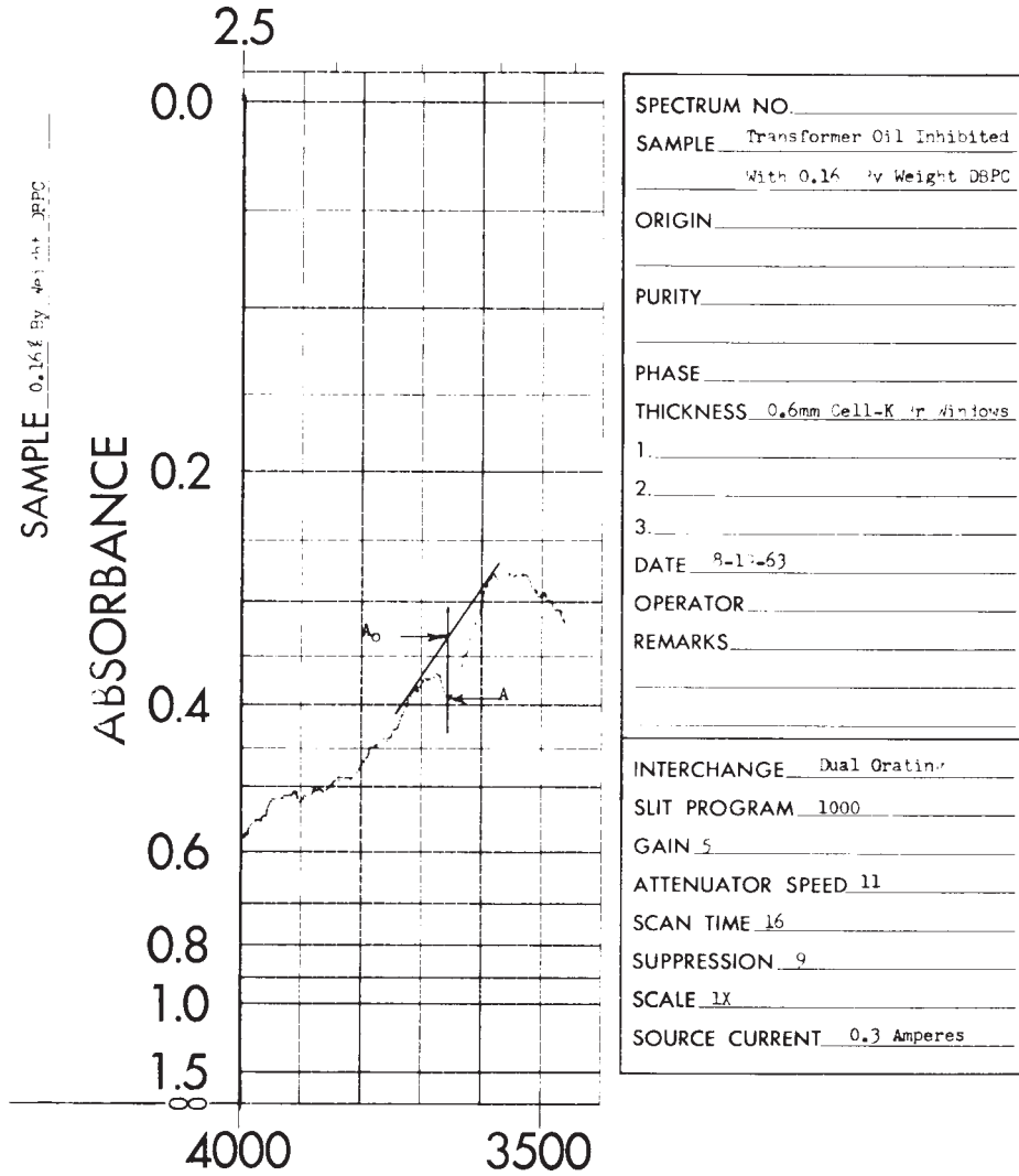
FIG. 1 Spectrum of an Electrical Insulating Oil Inhibited with 2,6-Ditertiary-Butyl Paracresol Showing Location Points A 0 and A
