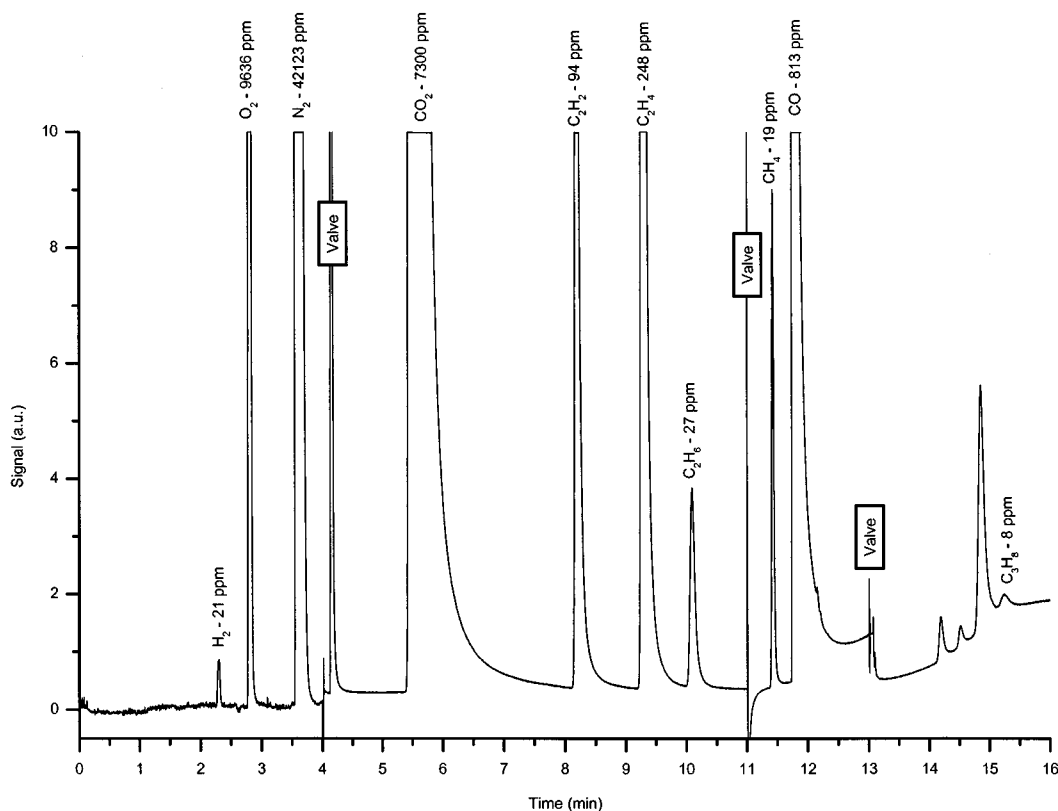
FIG. 8 Typical Chromatogram
