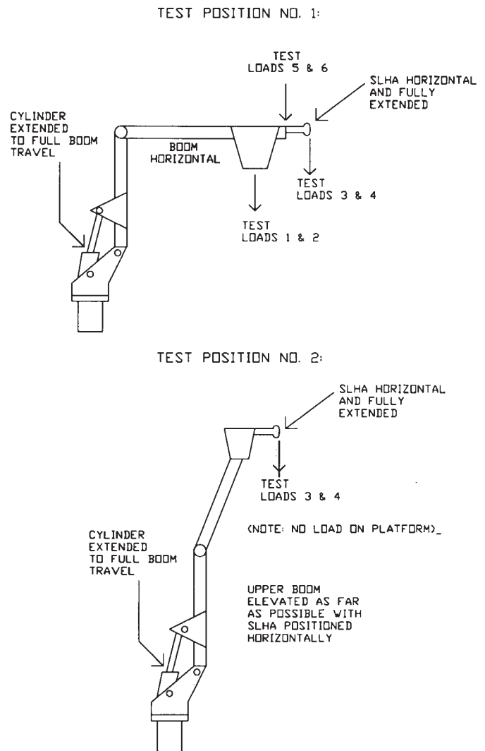
FIG. 4 Non-overcenter Articulating-Boom APD Recommended Test Positions and Test Loads
