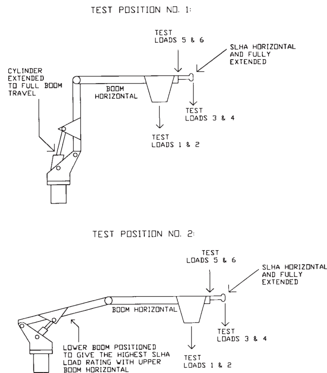
FIG. 4 Non-overcenter Articulating-Boom APD Recommended Test Positions and Test Loads
