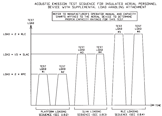
FIG. 6 APD Acoustic Emission Test Sequence
