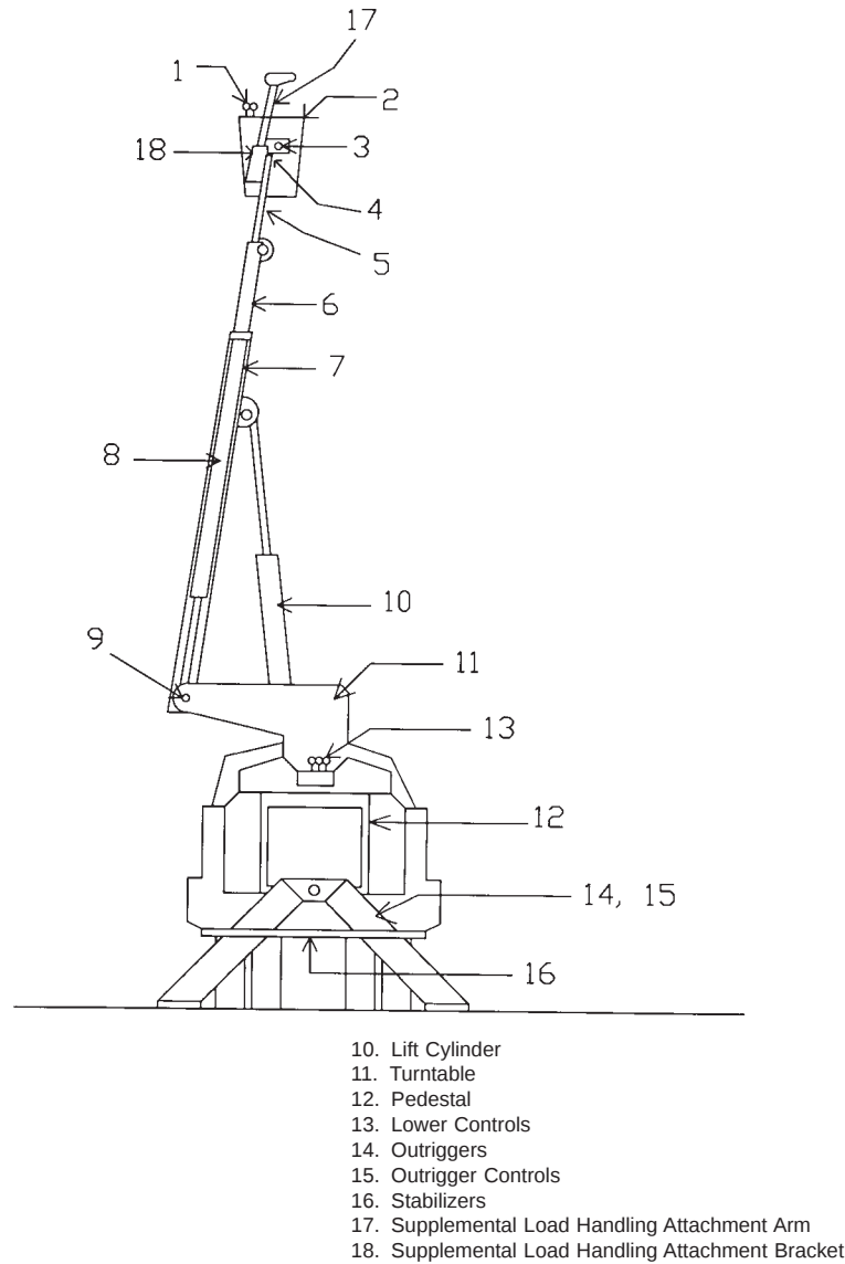
FIG. 2 Extensible-Boom APD Nomenclature Diagram
