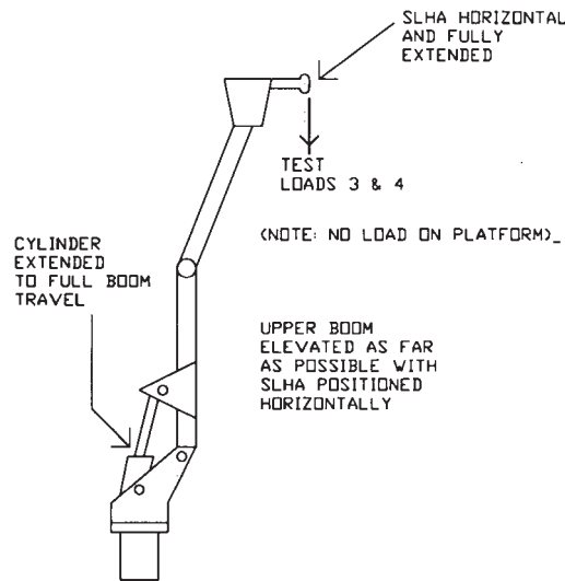
FIG. 4 Non-overcenter Articulating-Boom APD Recommended Test Positions and Test Loads
