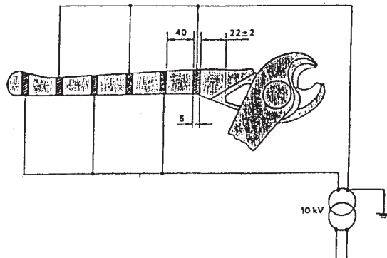
(a) Dielectric Test Between the Working Head and the Handle or the Legs (b) Dielectric Test of the Handle or Legs
