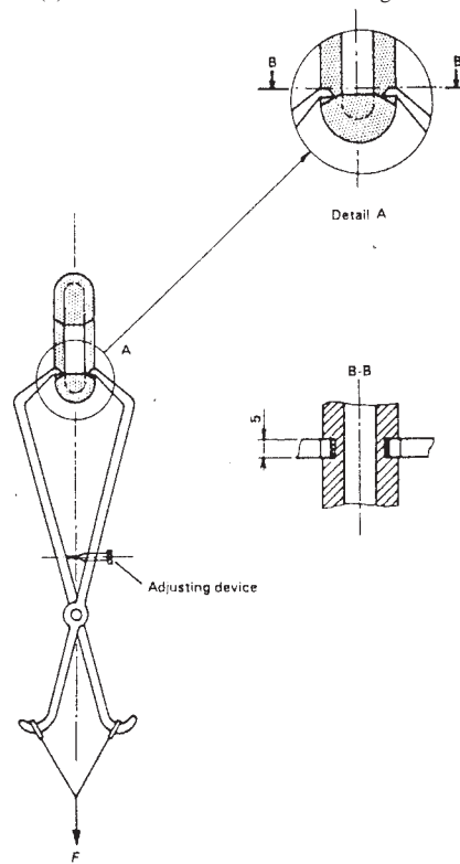
(b) Method B — Test on the Working Head
