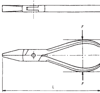
FIG. 113 Insulating Pliers;—Bending Test on Legs
