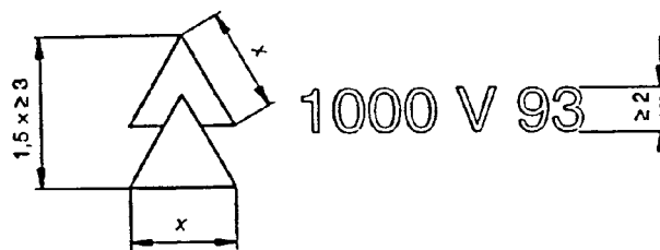
FIG. 4 Marking Symbol
