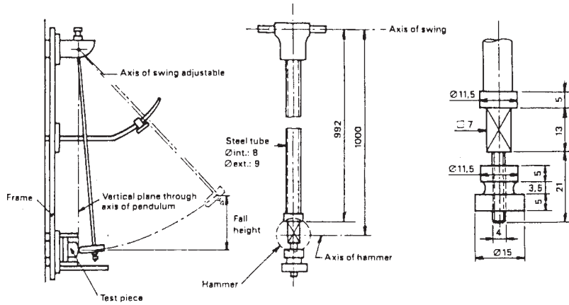
Pendulum for impact test
