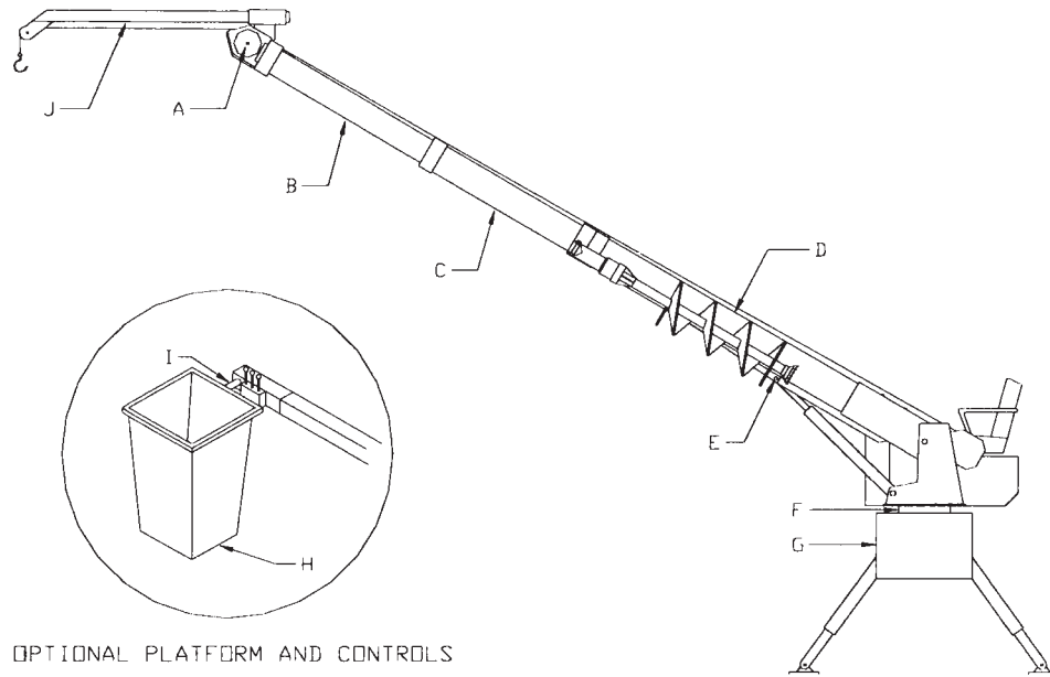
FIG. 1 Insulated Digger Derrick Nomenclature
