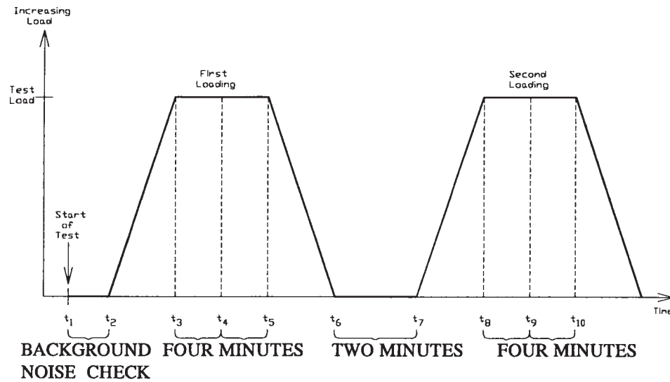
FIG. 3 Acoustic Emission Test Sequence for Insulated Digger Derrick
