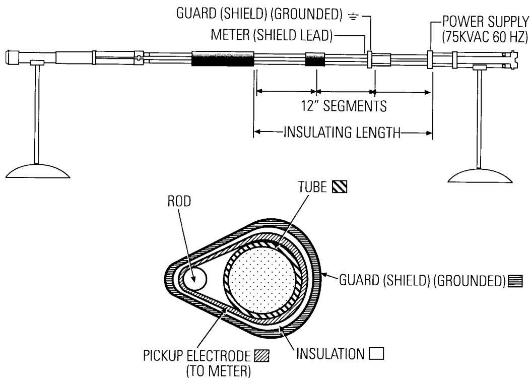
FIG. 1 Test Set-up Example
