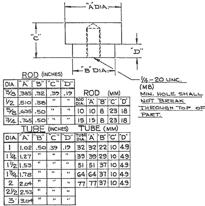
FIG. 8 Brass Electrode Detail
