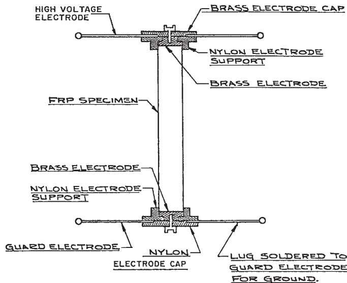
FIG. 5 Assembly Detail
