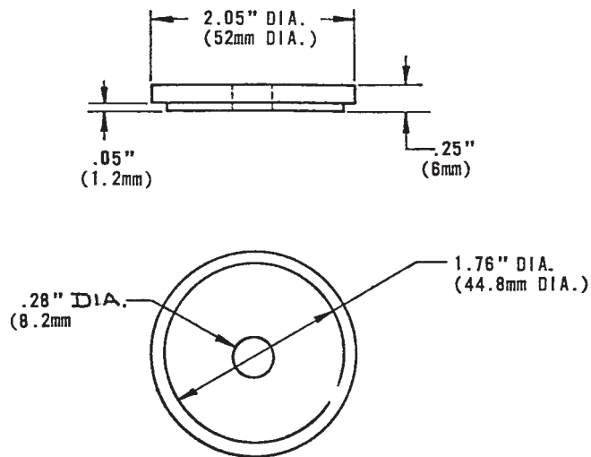
FIG. 6 Electrode Detail
