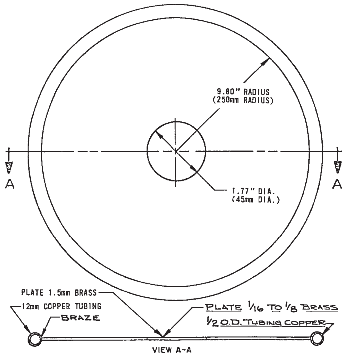
FIG. 6 Electrode Detail
