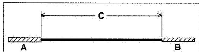
FIG. X1.1 Resistance Areas
