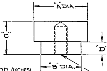
FIG. 6 Electrode Cap Detail
