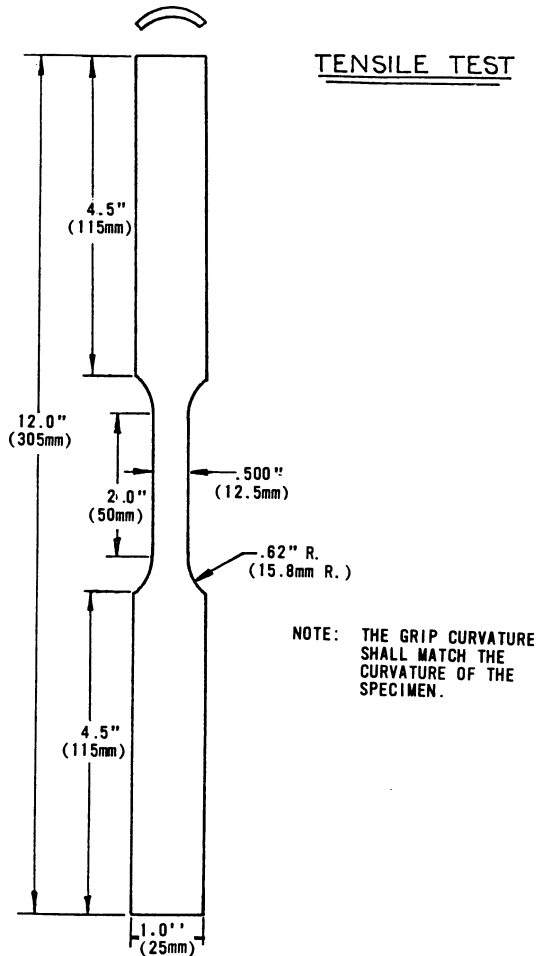
FIG. 1 Tension Test
