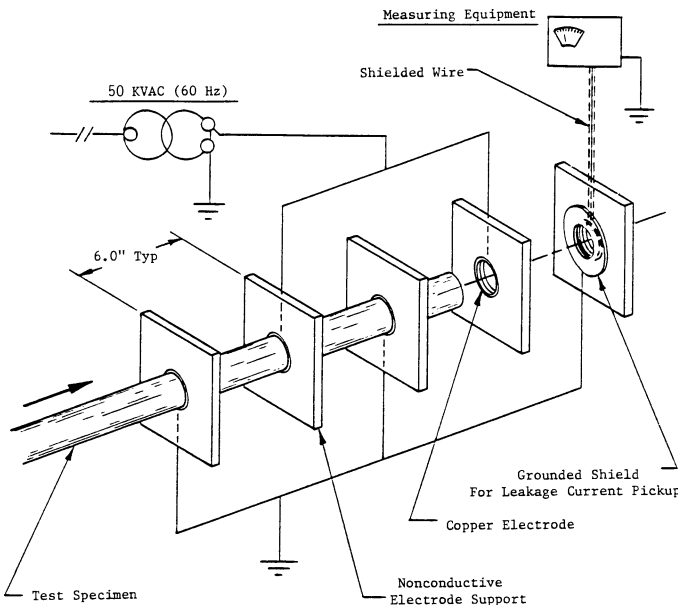
FIG. 11 Typical Test Set-Up
