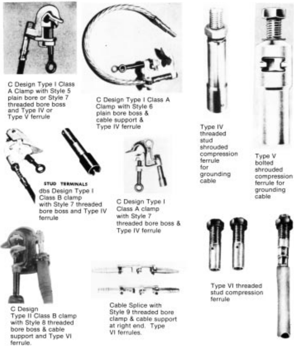
FIG. 11 Cable Terminations and Compatible Cable Ferrules for Grounding Clamps
