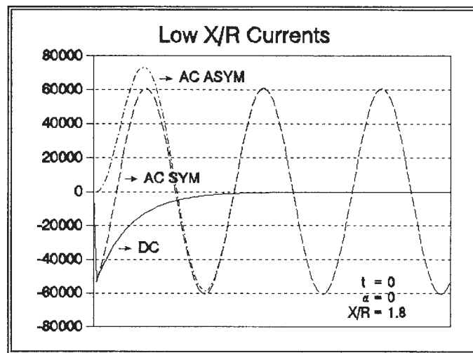
FIG. X4.3 Low X/R Currents
