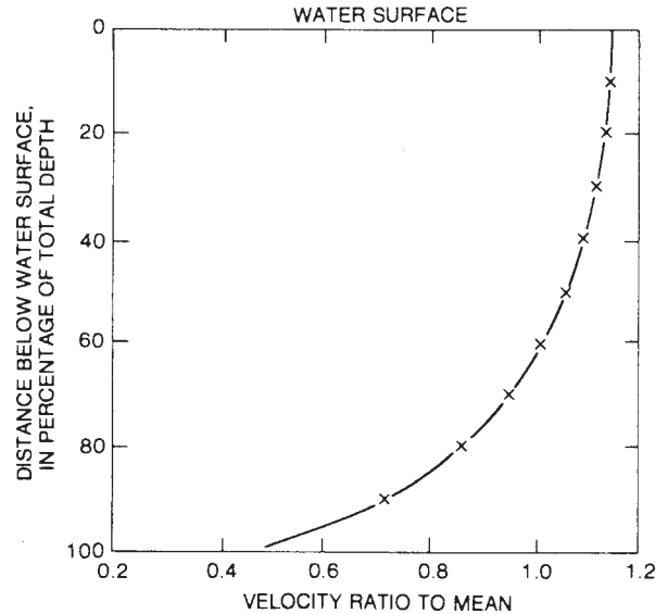
FIG. 8 Theoretical Vertical Velocity Distribution 6
