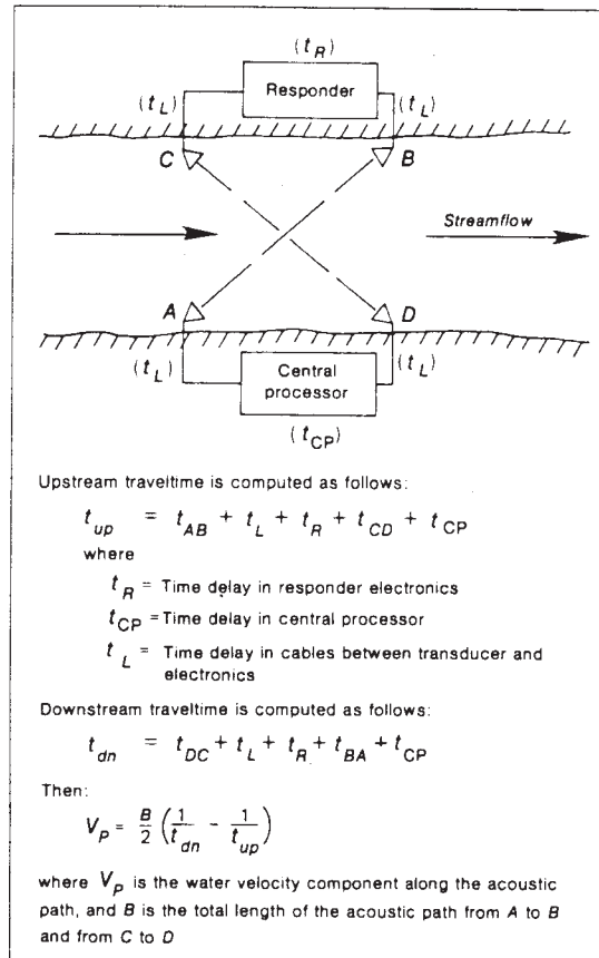
FIG. 7 Responder System
