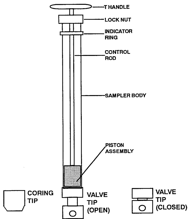
FIG. 14 Syringe Sampler
