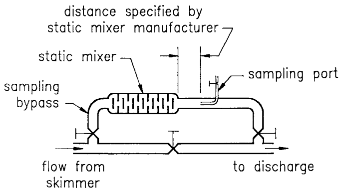
FIG. 2 Sampling Bypass
