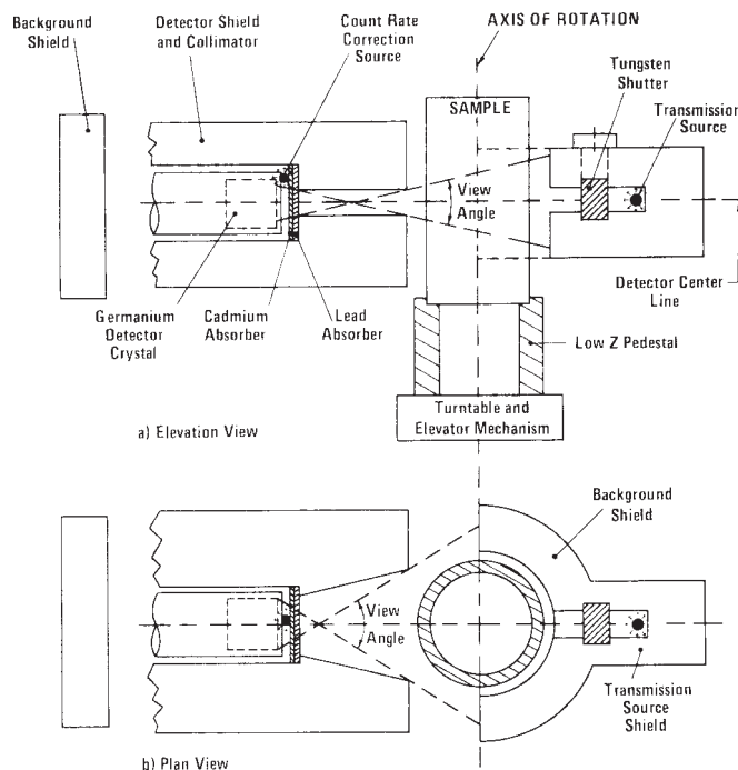
FIG. 1 Gener Typical Arrangement for Segmented Gamma-Ray Scanning
