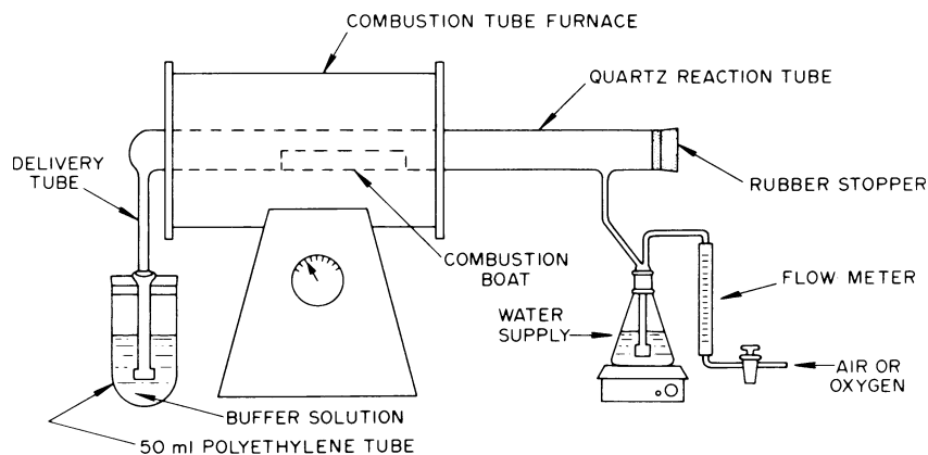
FIG. 3 Pyrohydrolysis Apparatus
