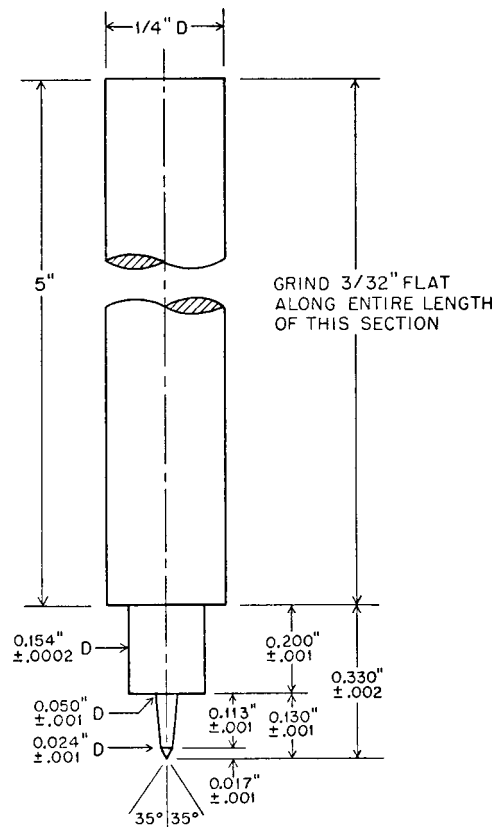
FIG. 2 Venting Tool
