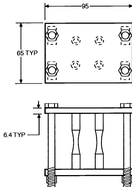
FIG. X2.1 Dimensions of Specimen Master Holder
