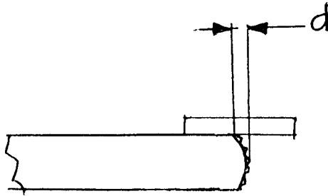
FIG. 5 Depth Measurement of Beveled Region
