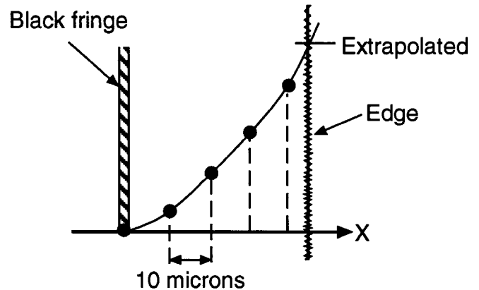
FIG. 3 Extrapolation Procedure Plotting Birefringence Versus Position
