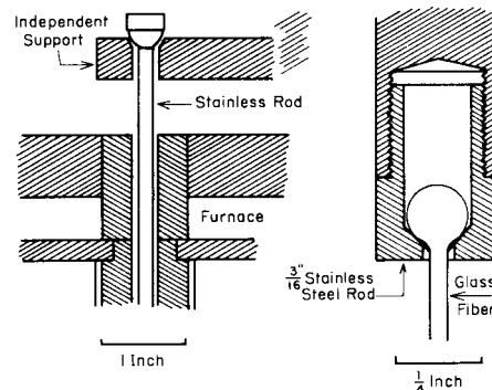
(a) Independent Support for Steel Rod (b) Method of Attaching Sample Fiber to Steel Rod. FIG. 4 Apparatus Assembly for Suspension of Sample Fiber Between Metal Rod
