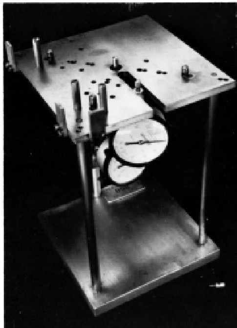
FIG. 1 Apparatus for Square Tile, Set Up for Measurement of 4¼- by 4¼-in. (108- by 108-mm) Tile
