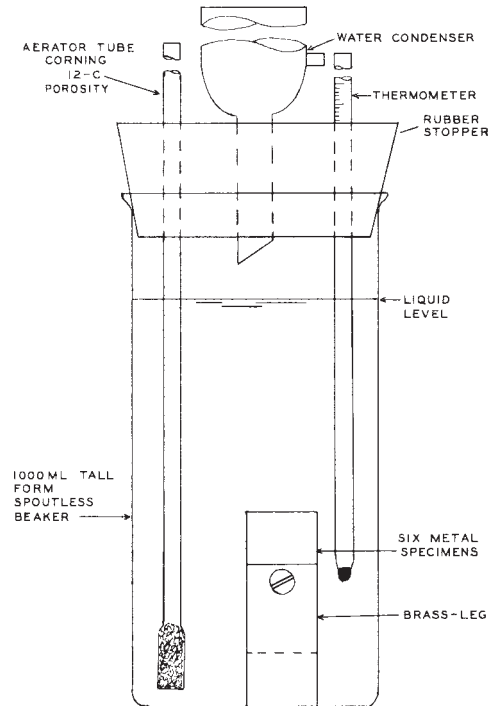
FIG. 1 Metal Specimens and Equipment for the 336-h Corrosion Test
