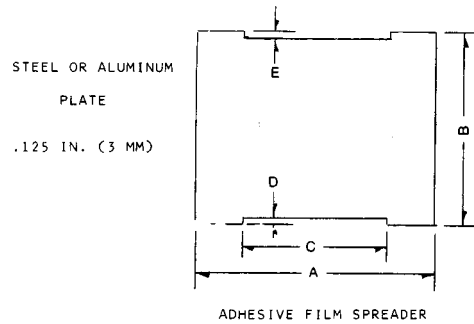
FIG. 6 Specimen for Test of Durability (Moisture Resistance)
