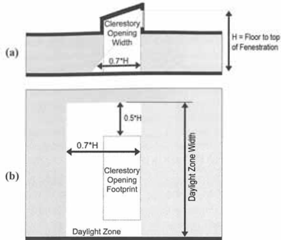
(a) Elevation view and (b) plan view of daylight zone under clerestory roof monitor.
