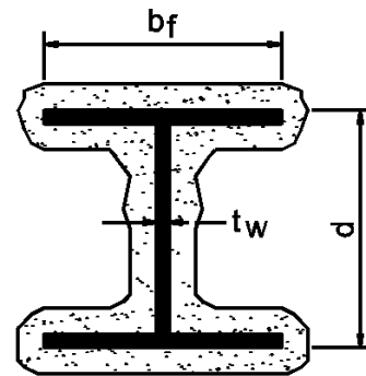
FIGURE 722.5.1(5) WIDE FLANGE STRUCTURE STEEL COLUMNS WITH SPRAYED FIRE-RESISTANT MATERIALS
