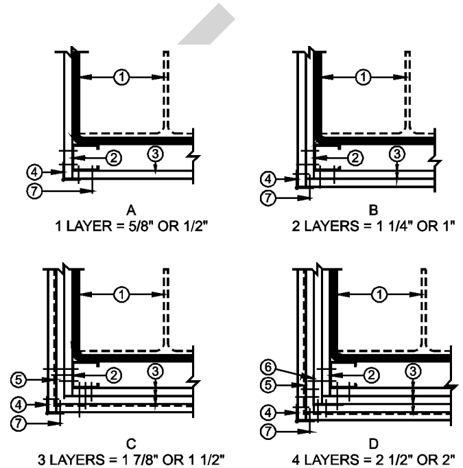
FIGURE 722.5.1(3) GYPSUM WALLBOARD PROTECTED STRUCTURAL STEEL COLUMNS WITH STEEL STUD/SCREW ATTACHMENT SYSTEM
