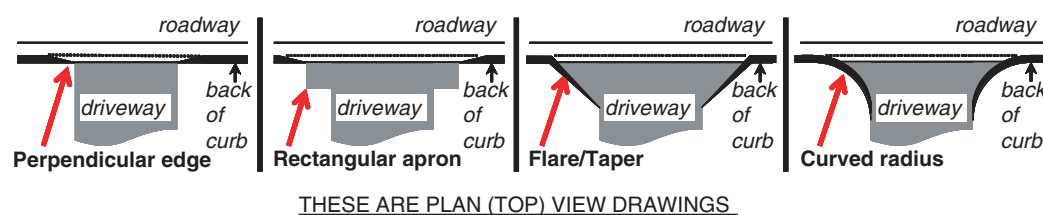
Exhibit 5-19. Types of driveway connection transition geometry.
