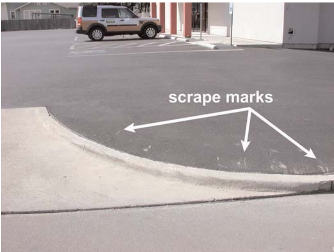
Exhibit 5-5. Poorly defined edge leads to scrapes.
