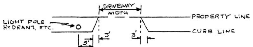
Exhibit 5-49. Driveway edge clearance from fixed objects.
