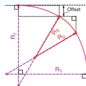
Exhibit 5-26. Geometry of a symmetrical 3-centered curve.
