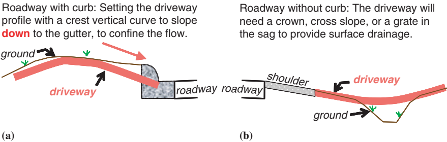
Exhibit 5-70. Confining surface runoff flow.
