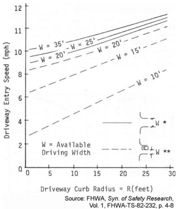
Exhibit 3-10. Driveway entry speed related to driveway radius and width.
