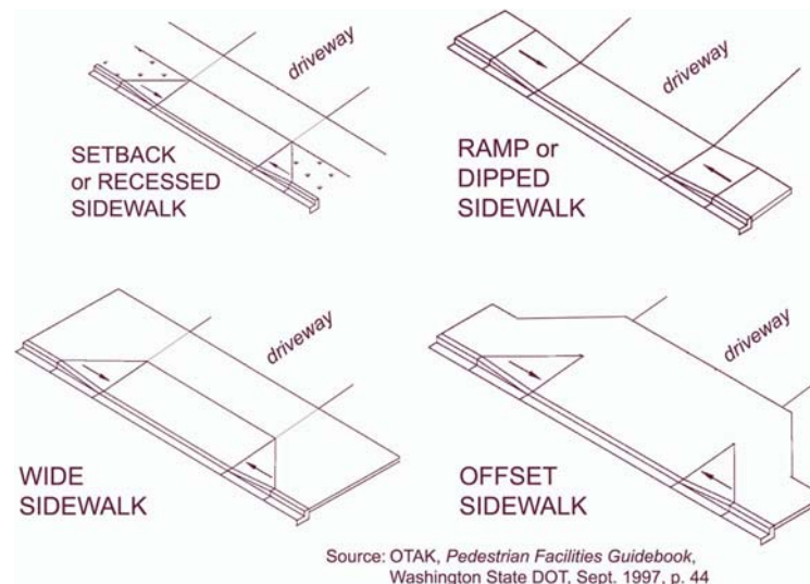
Exhibit 5-9. Sidewalk-driveway treatments.
