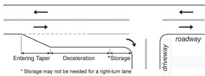
Exhibit 5-78. Parts of a deceleration lane.
