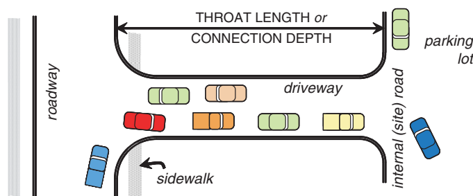
Exhibit 5-52. Driveway throat.
