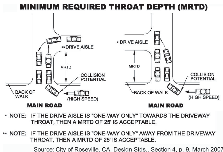
Exhibit 5-56. Roseville explanatory drawing.
