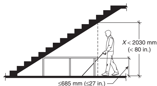
Figure J.4 Vertical Clearance.
