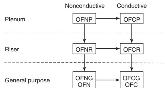
Figure 770.154 Cable Substitution Hierarchy.
