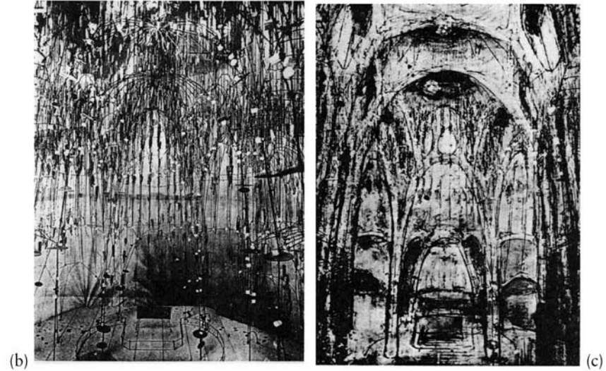
Figure 14.78 (b) Photograph of the inside of the model, rotated through 180^\circ . The upside-down cables change into arches. (c) Interior sketch by Gaudi on the basis of the model.
