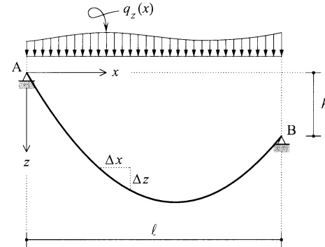
Figure 14.18 Cable with distributed load (force per horizontally measured length).
