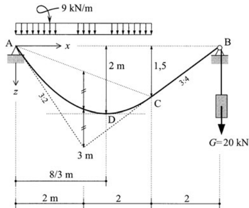
Figure 14.15 The cable is parabolic over AC. To sketch the shape of the cable, we can use the same auxiliary lines when drawing a parabolic bending moment diagram.
