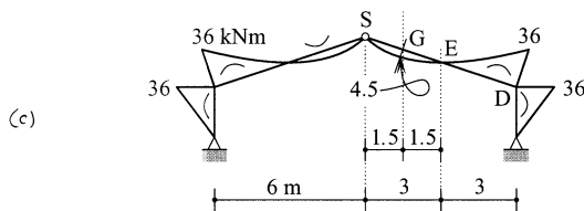
Figure 14.67 (c) Bending moment diagram.
