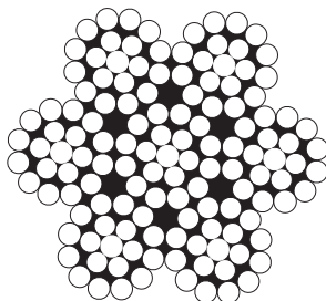
7 X 19
