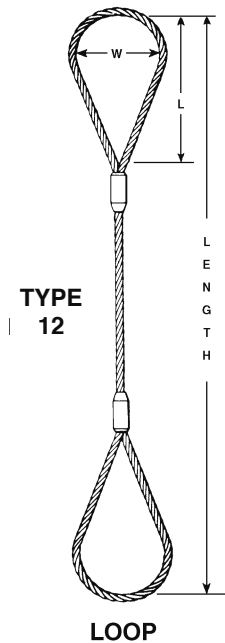
SINGLE LEG
