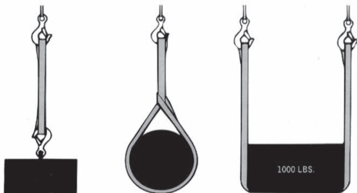
Vertical Hitch
