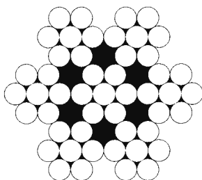
7 X 7
