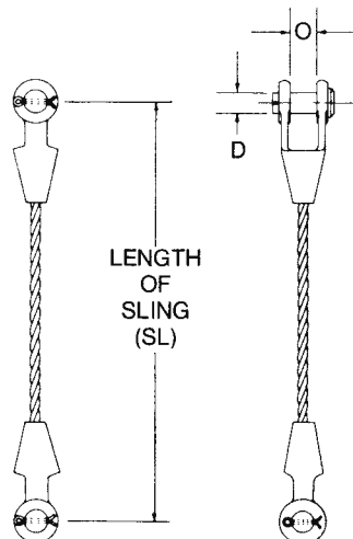
PINS PARALLEL PINS AT RIGHT ANGLES
