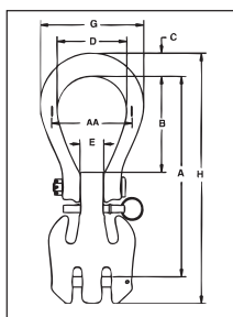
A-1362 Crosby ELIMINATOR® Double Hook
