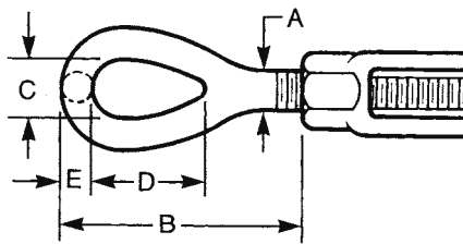
EYE
