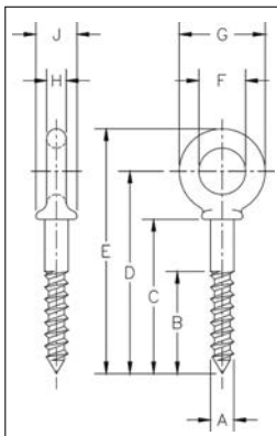
G-275 Screw Eye Bolts
