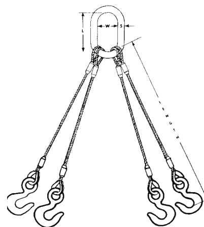
TYPE 41
