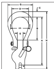
A-1361 Crosby ELIMINATOR® Single Hook
