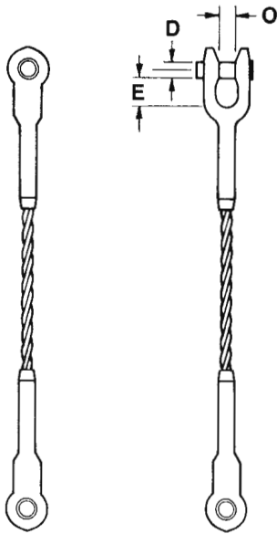
PINS PARALLEL
