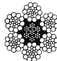
6 x 26 WARRINGTON-SEALE
