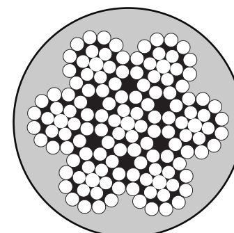
7 X 19
