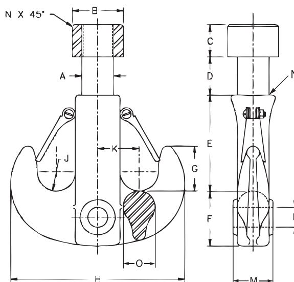
Duplex Hook with Nut and Latches Dimensions (in.)
