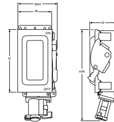
Crouse-Hinds Receptacle
