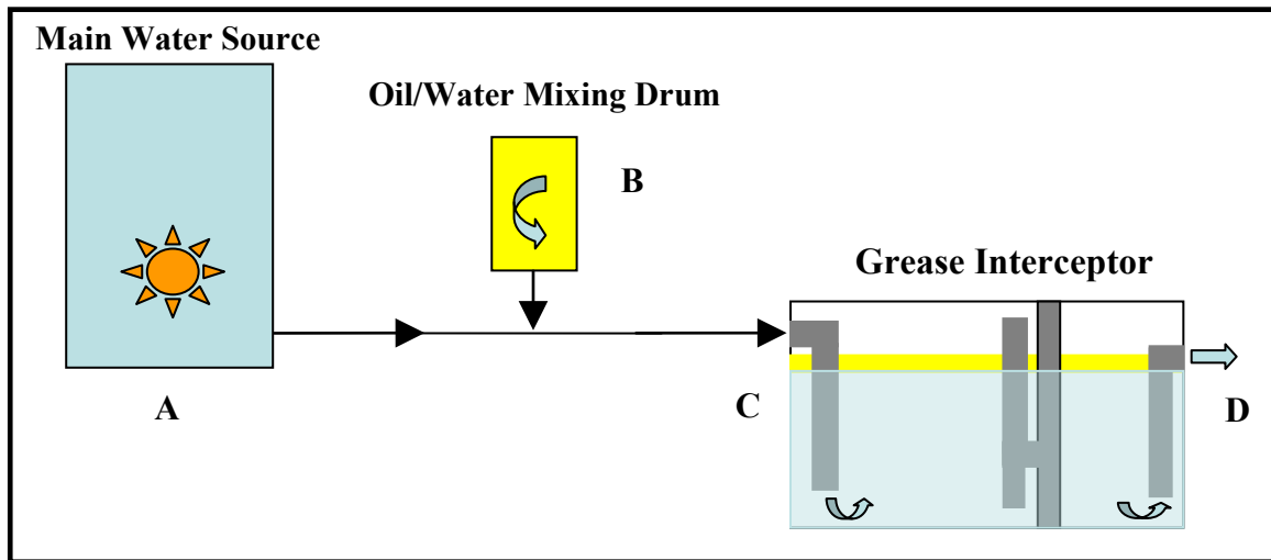
Figure 2-4. Conceptual Schematic for Lab Grease Interceptor: a) How Water Source, b) Oil/Water Mixing Tank, c) Influent Sample Location of GI, d) Effluent Sample Location of GI.
