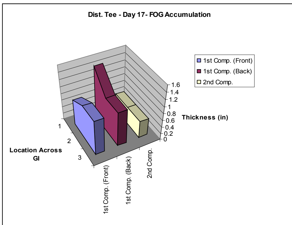
Figure 4-19. Day 13 and 17 FOG Thickness Profile in Distributive Tee-inlet GI.
