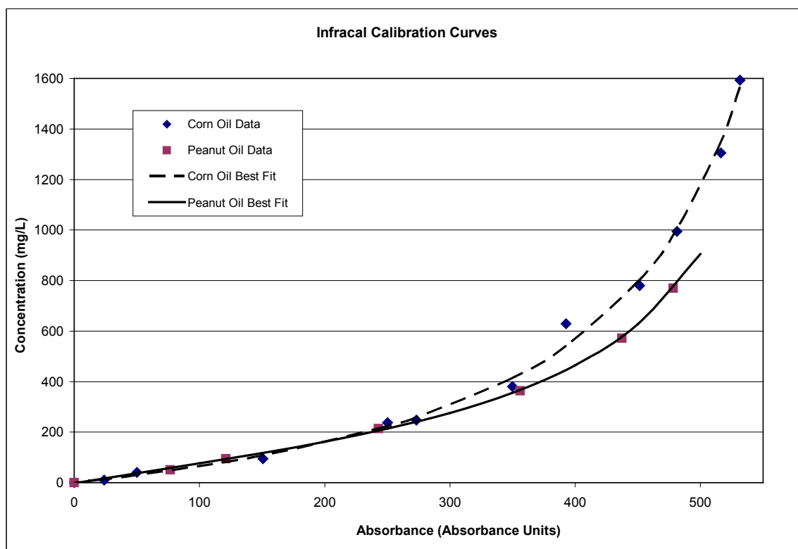
Figure 5-2. Infracal ® Calibration of Corn Oil and Peanut Oil.
