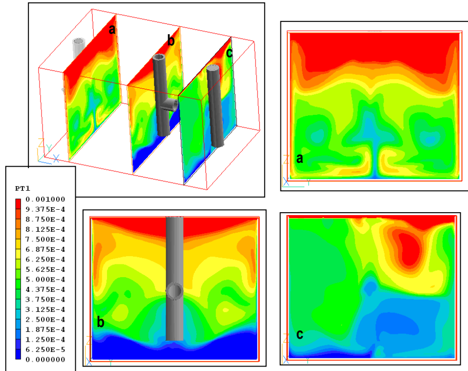
Figure 5-30. 15gpm Distributive Inlet/Standard Baffle Configuration Image Showing Volume Fraction of Oil (Contours) for ASM Simulation.
