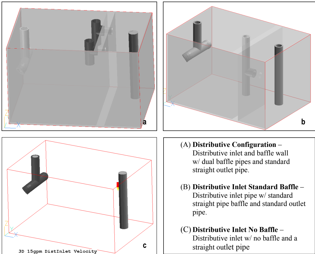
Figure 5-16. Simulated 3D GI Configurations (Distributive Configurations).
