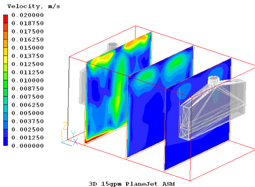
Figure 5-21. Velocity Contours in the Flow Direction for DPJ Configuration.
