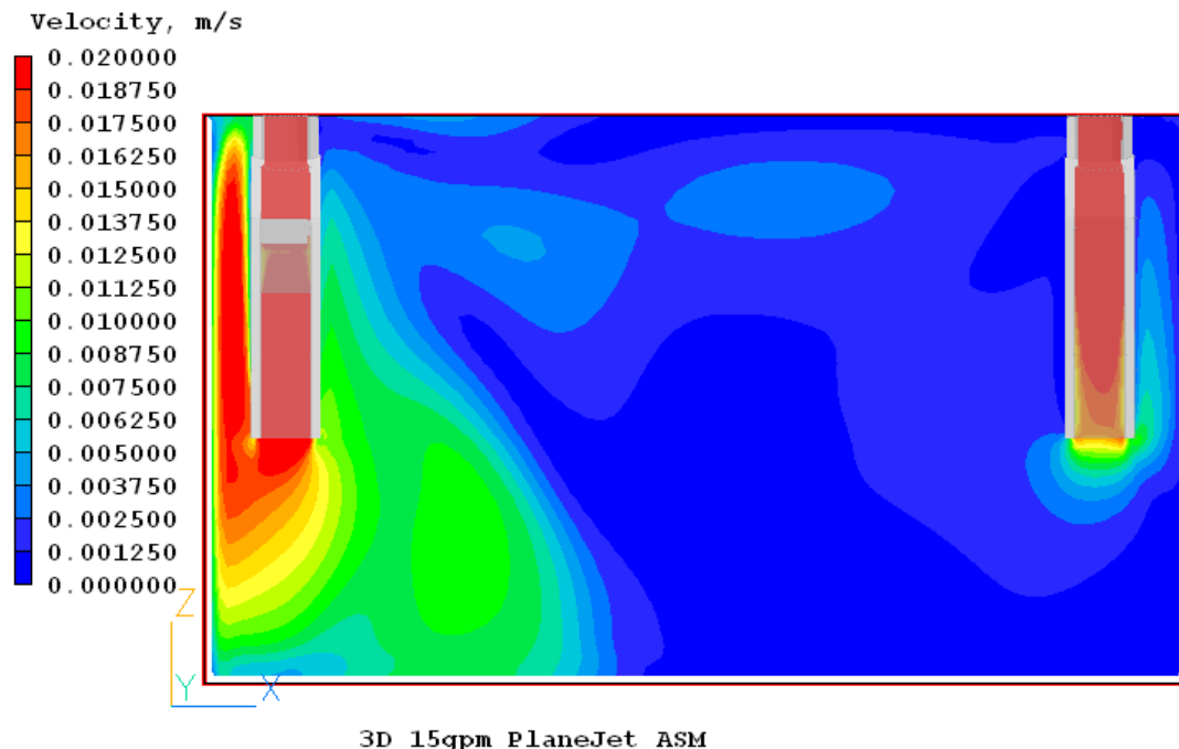
Figure 5-20. Velocity Contours Along the Center of the DPJ 15gpm Simulation.
