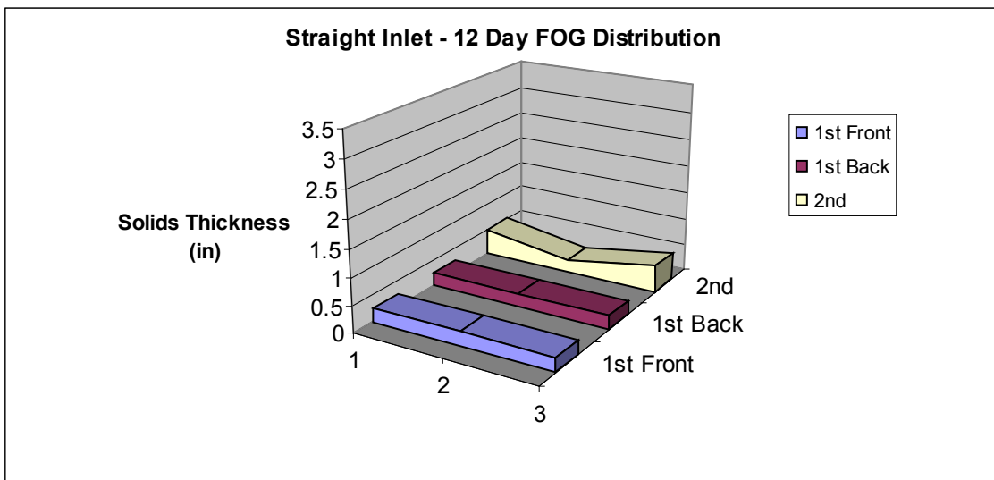
Figure 4-23. Day 9 and 12 FOG Thickness Profile in Straight Inlet GI.
