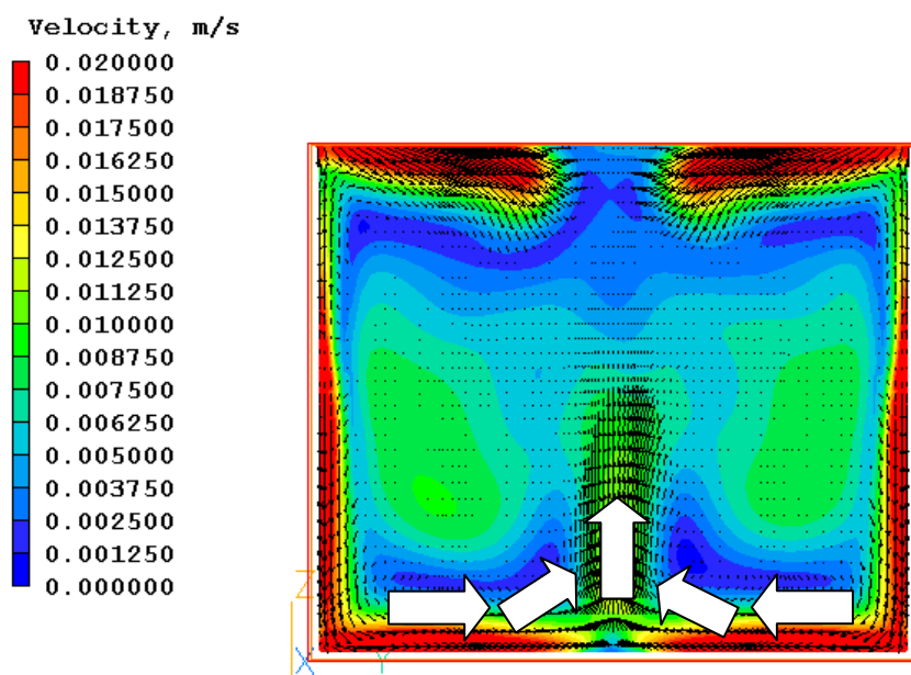
Figure 5-24. Velocity Contours for Distributive Inlet/No Baffle.
