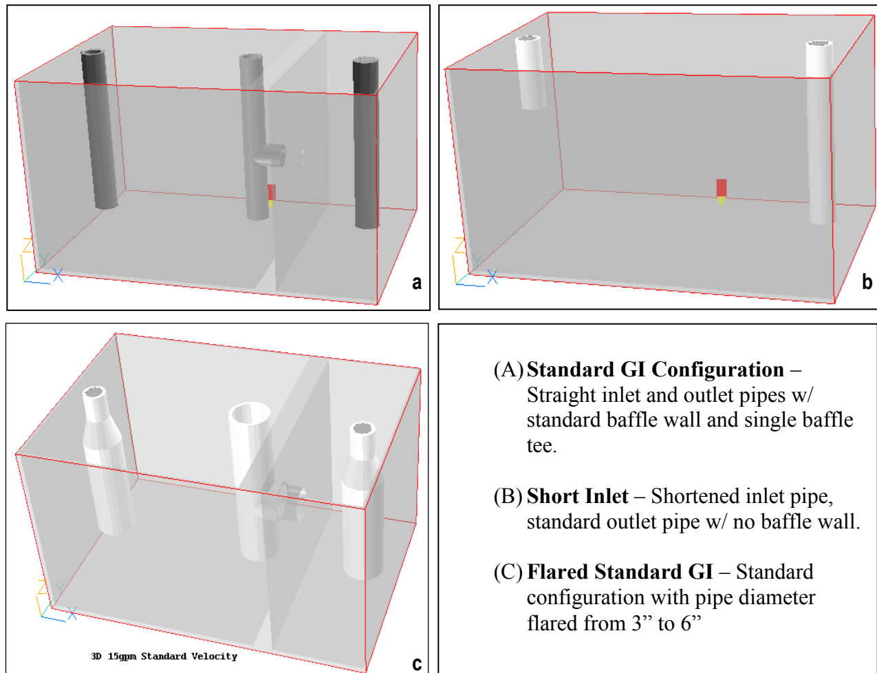
Figure 5-15. Simulated 3D GI Configurations (Straight Pipe Configurations).
