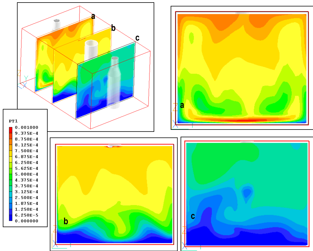
Figure 5-27. 15gpm Flared Configuration Image Showing Volume Fraction of Oil (Contours) for ASM Simulation.
