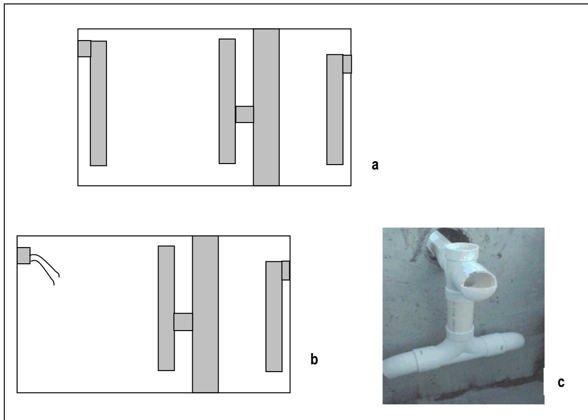
Figure 4-6. Field Grease Interceptors Observed: a) Standard Inlet Tee, b) No Inlet Tee, c) Distributive Inlet Tee.
