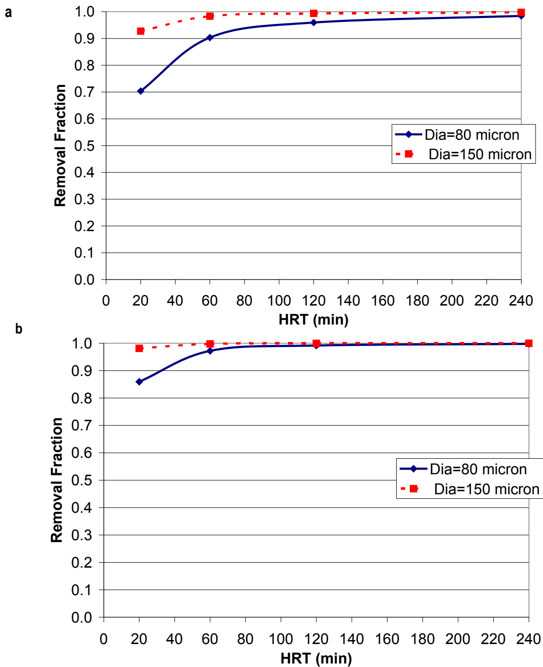
Figure 5-36. Fraction of Removal for 80 and 150 Micron FOG Globule Sizes: a) N = 1.5 for N Tanks in Series RTD Model, b) N = 2.0 for N Tanks in Series RTD Model.
