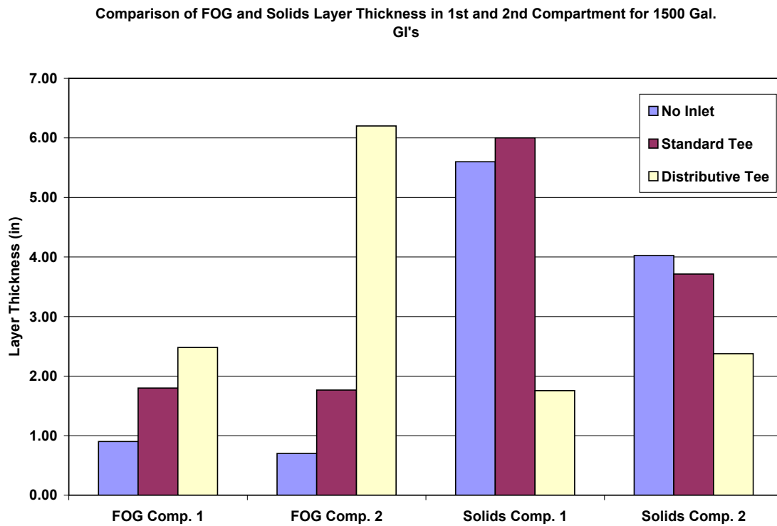
Figure 4-8. Graphical Representation of Table 4-10.
