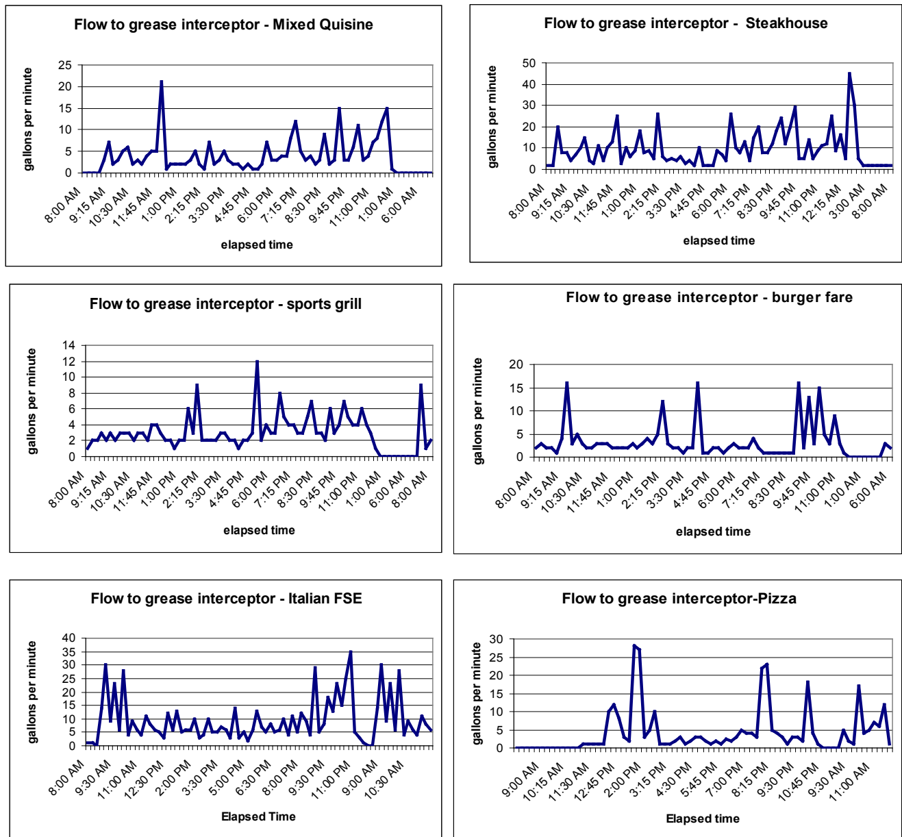
Figure 4-3a. Analysis of Flow Data from Sampled Grease Interceptor Influent from Several Restaurants.
