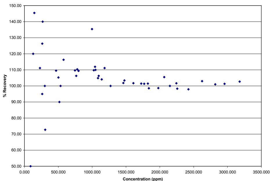
Figure 5-1. Data from Evaporative Testing at Various Concentrations.
