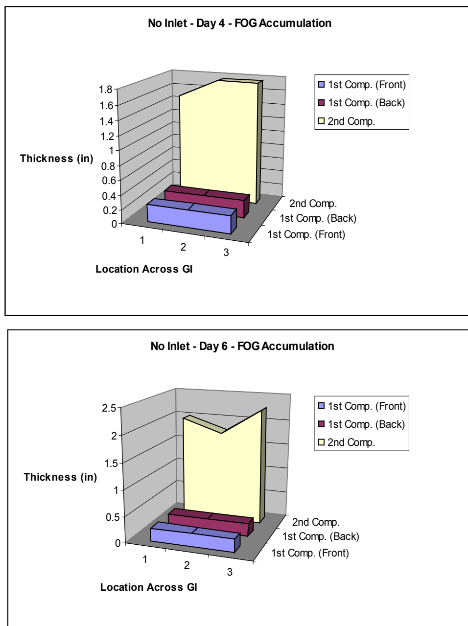
Figure 4-14. Day 4 and 6 FOG Thickness Profile in No-inlet GI.
