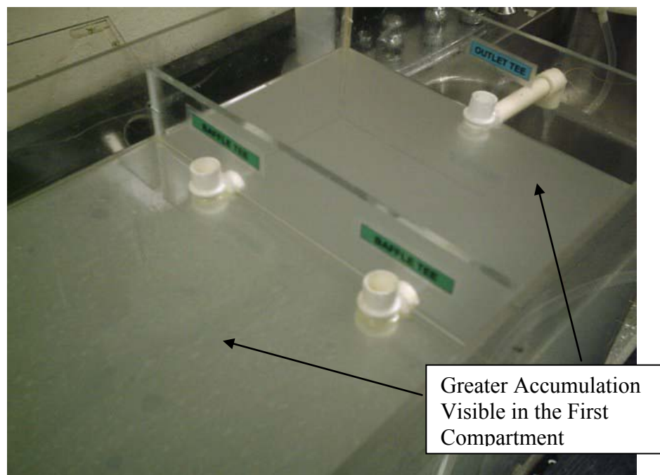
Figure 5-8. Top View of 1hr Residence Time Bench Scale Experiment.
