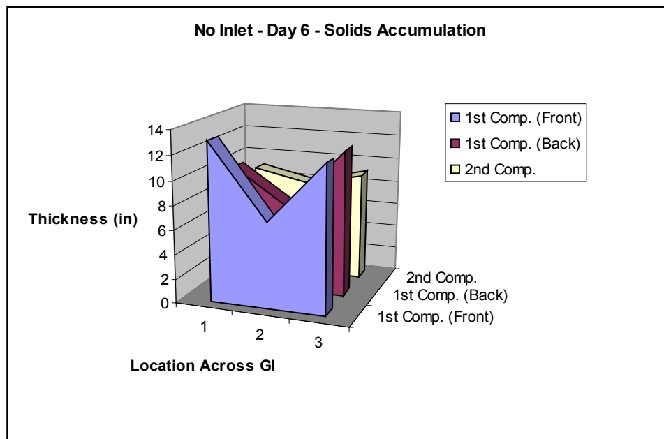
Figure 4-16. Day 4 and 6 Solids Thickness Profile in No-inlet GI.
