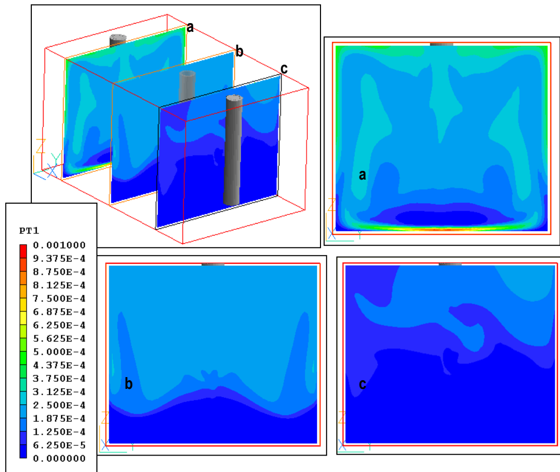
Figure 5-28. 5gpm Standard Configuration Image Showing Volume Fraction of Oil (Contours) for ASM Simulation.
