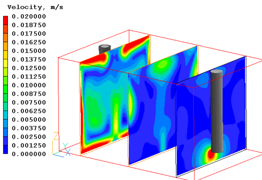
Figure 5-23. Velocity Contours for Distributive Inlet/No Baffle.
