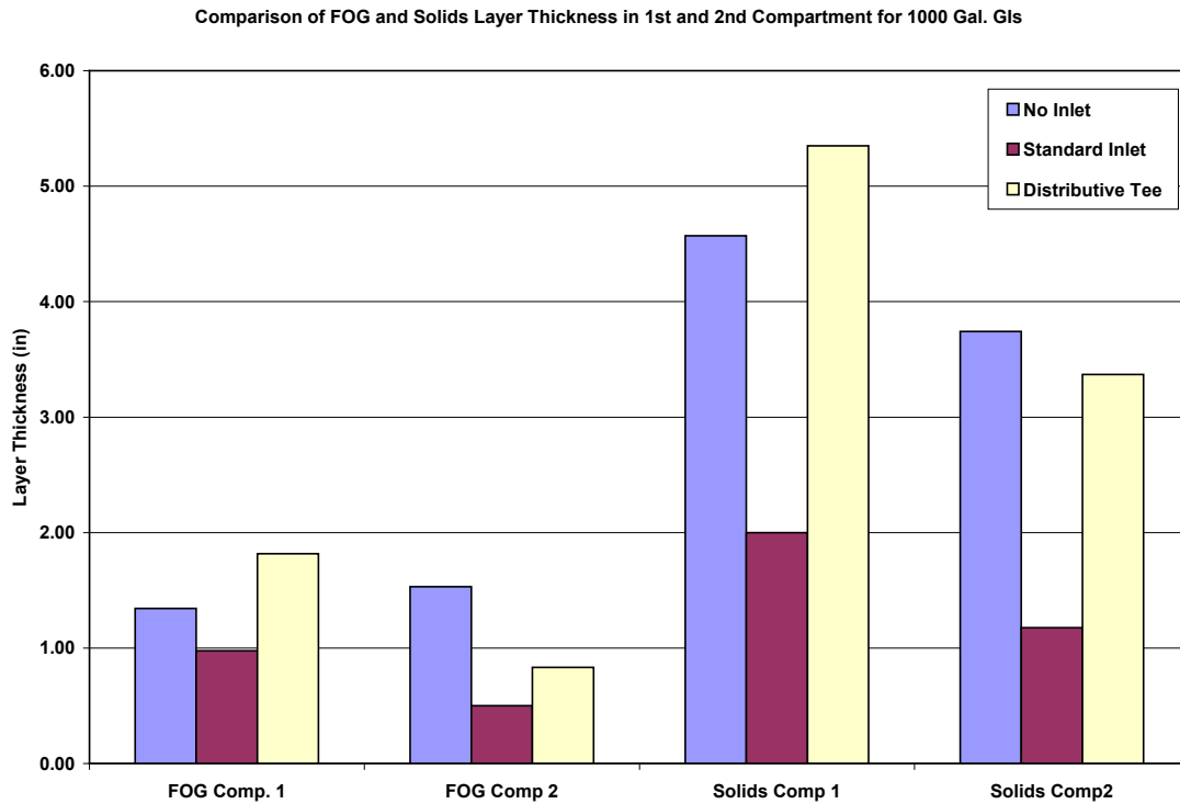
Figure 4-7. Graphical Representation of Table 4-9.
