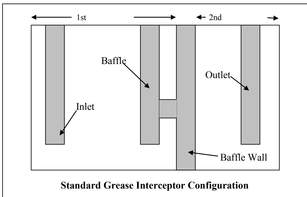
Figure 2-7. Definition of Grease Interceptor Terms.
