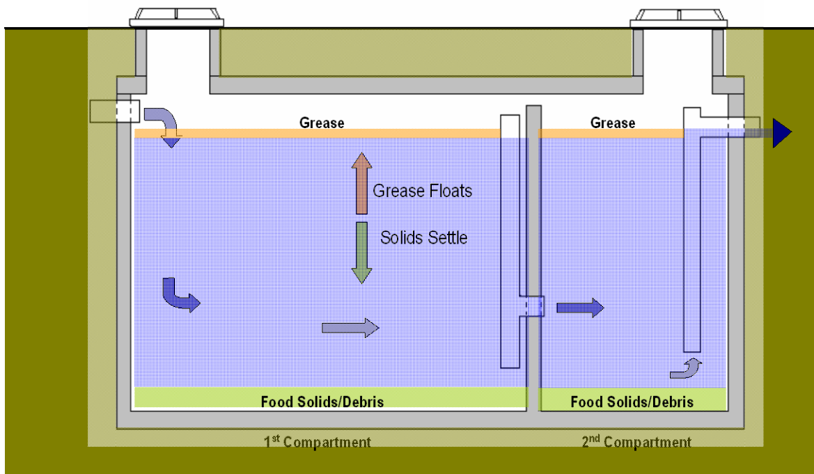
Figure 1-1. Standard Configuration of Grease Interceptor.
