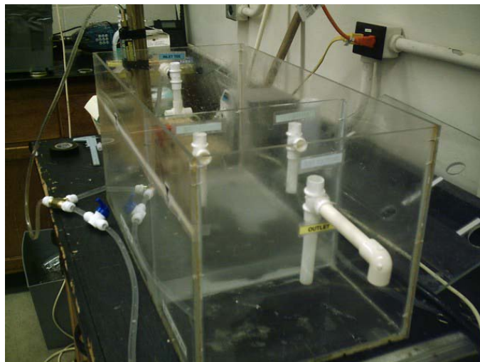
Figure 2-9. Bench Scale Reactor with Distributive Tee Configuration.
