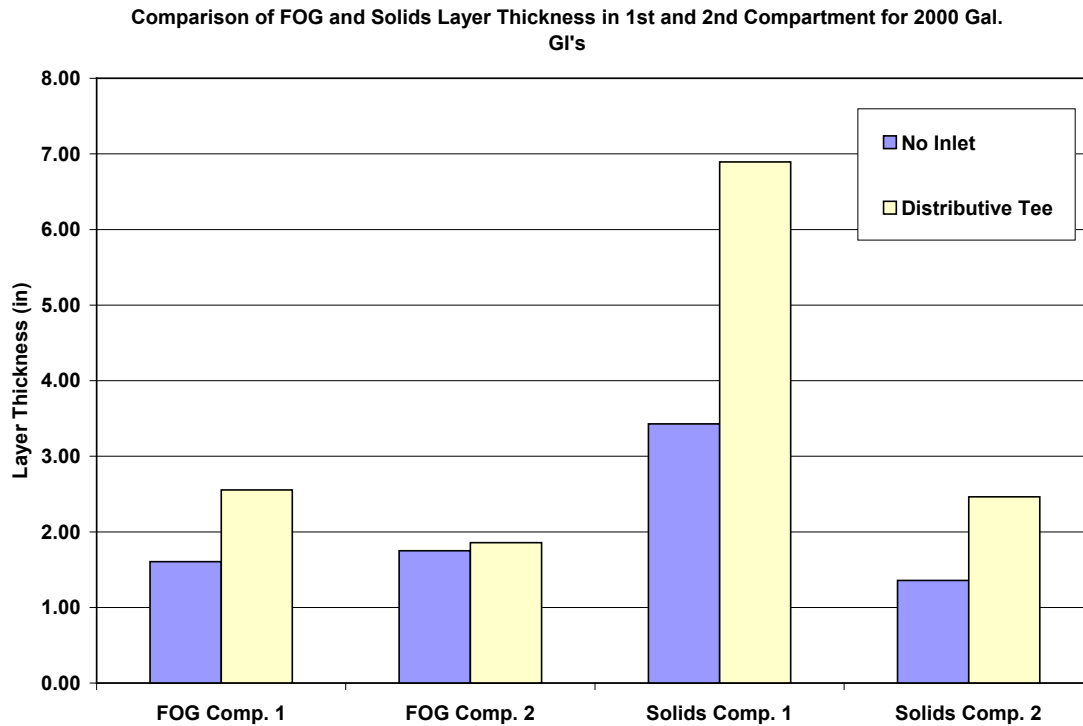
Figure 4-9. Graphical Representation of Table 4-11.
