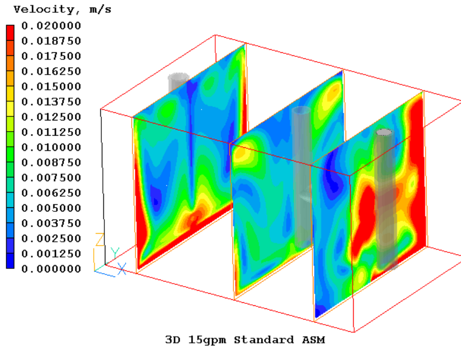
Figure 5-19. Velocity Contours in the Flow Direction for Standard Configuration.
