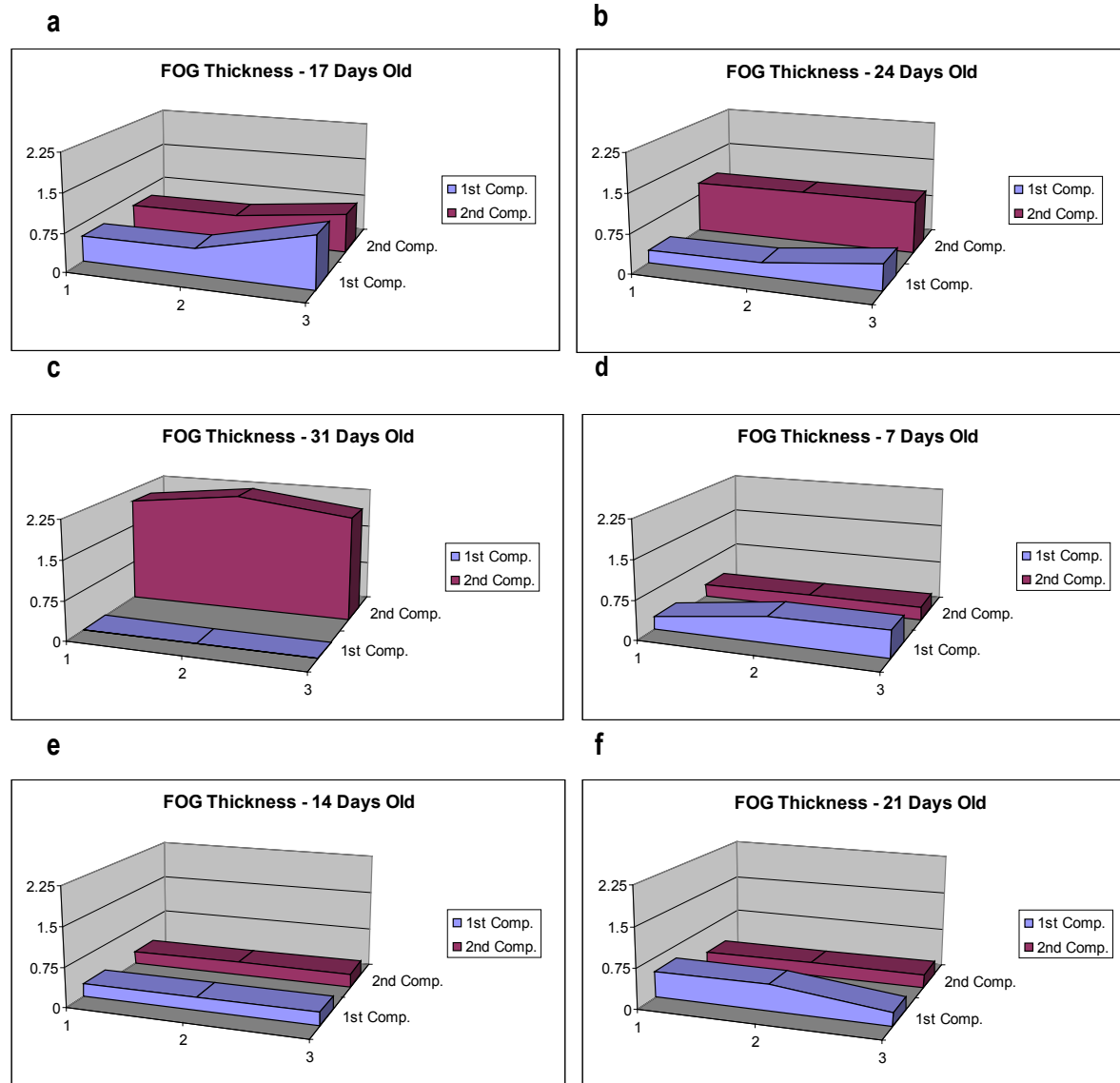
Figure 4-11. FOG Thickness in First and Second Compartment for GI with No Food Grinder.
