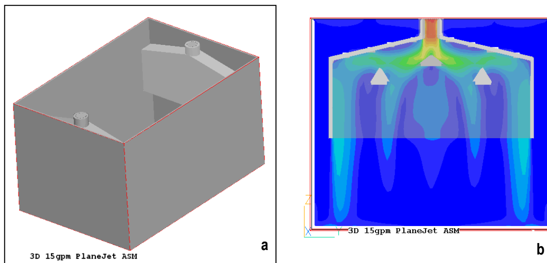
Figure 5-17. a) Simulated 3D GI Configurations (Distributive Plane Jet Configuration), b) Velocity Contours Depicting the Flow Distribution in the Inlet.
