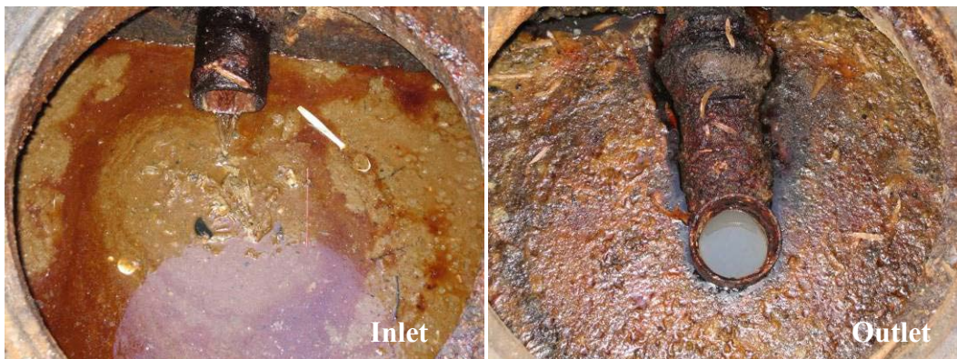
Figure 4-4. Inlet and Outlet of On-Campus Dining Facility GI.
