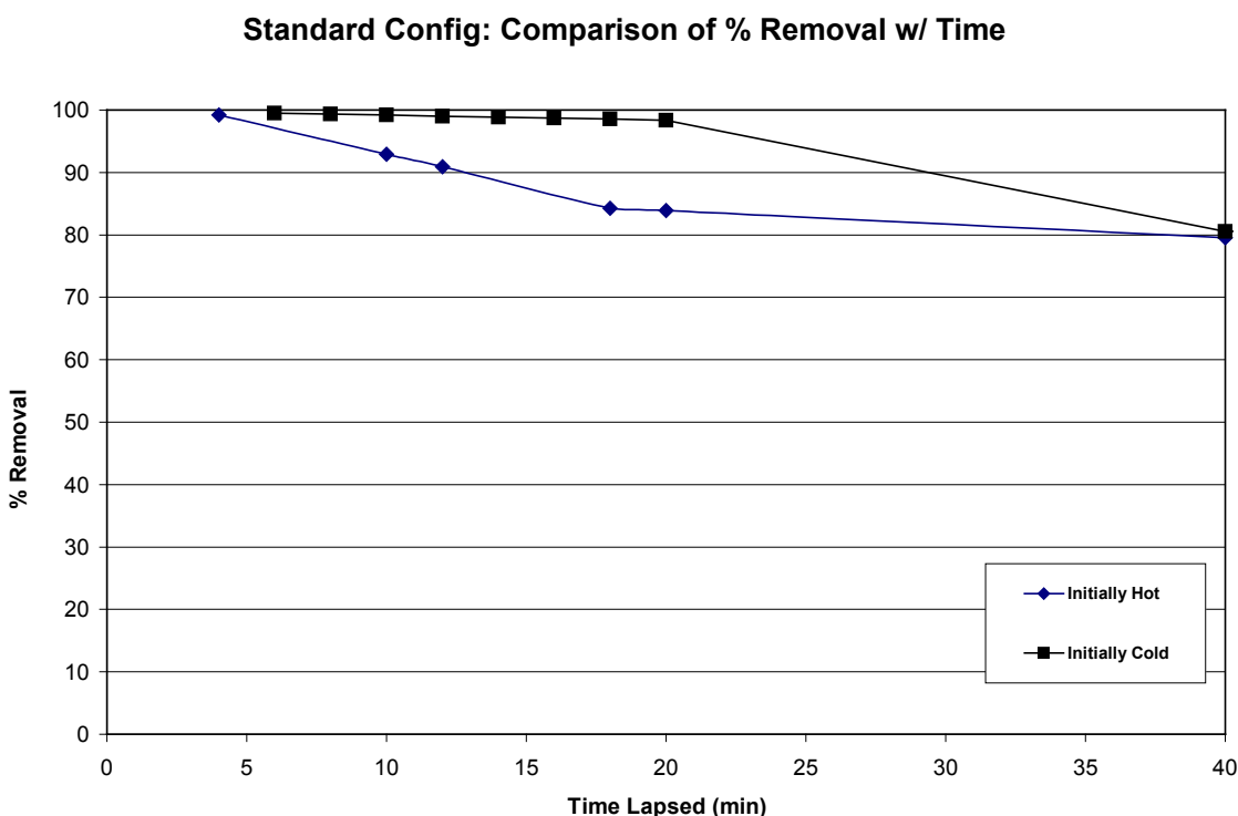
Figure 5-9. % Removal Over Time for Standard Configuration with Initially Cold or Initially Hot Water.
