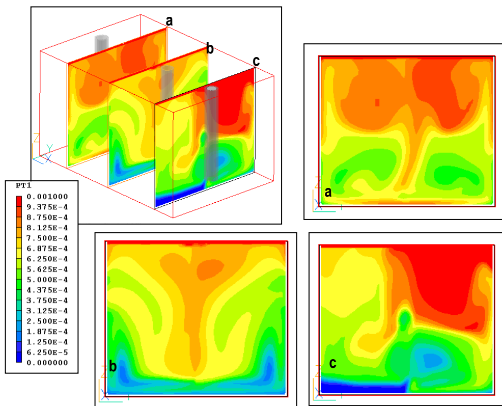
Figure 5-25. 15gpm Standard Configuration Image Showing Volume Fraction of Oil (Contours) for ASM Simulation.
