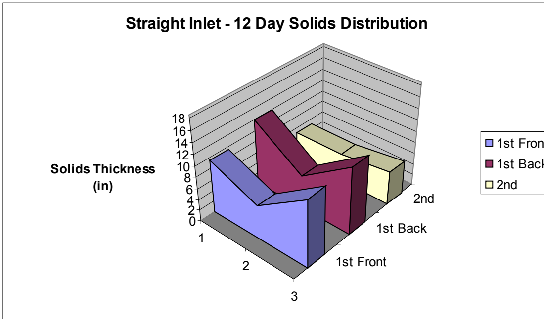
Figure 4-25. Day 9 and 12 Solids Thickness Profile in Straight Inlet GI.
