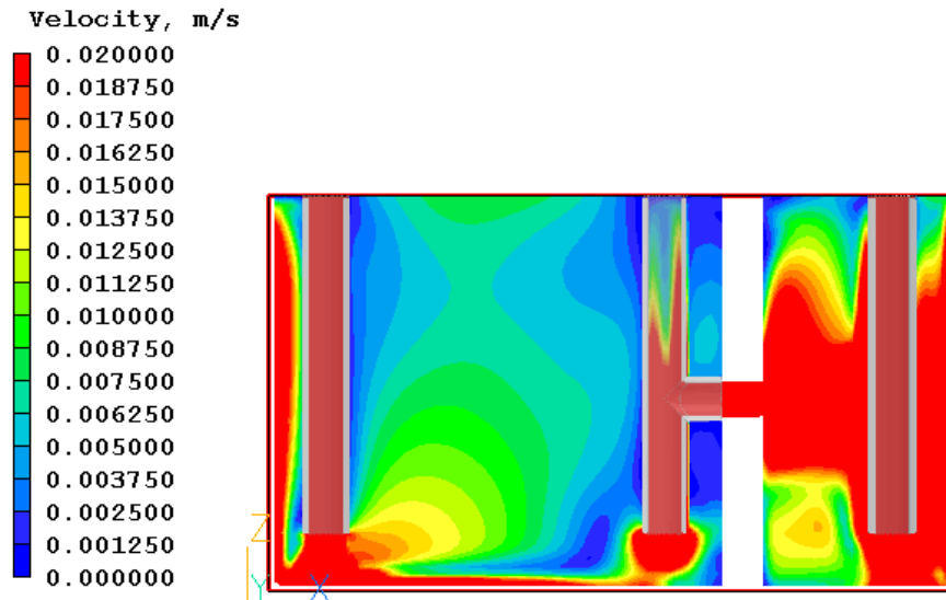
Figure 5-18. Velocity Contours Along the Center of the Standard 15gpm Simulation.
