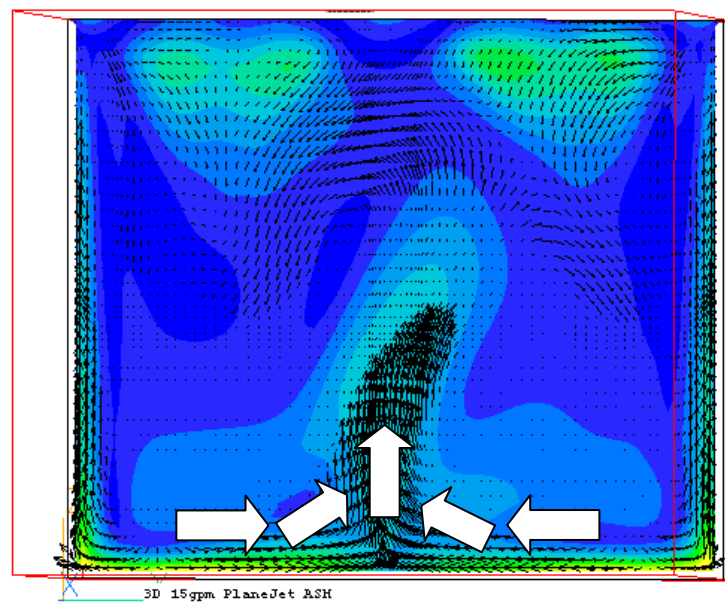
Figure 5-22. Velocity Contour Near the Inlet, Showing the Upward Flow Motion.
