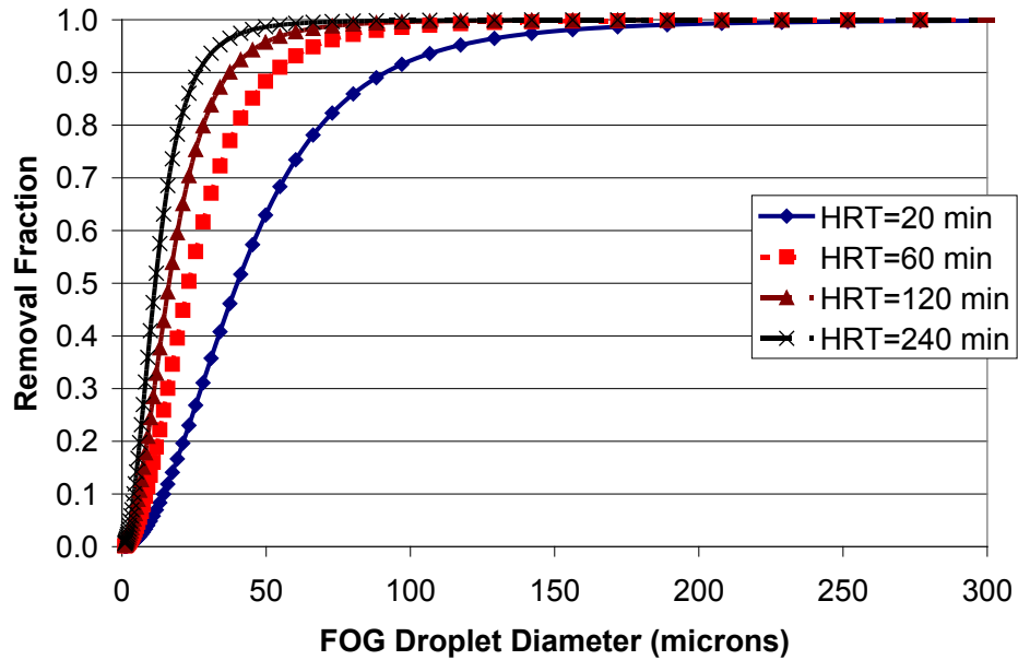
Figure 5-35. Fraction of Removal for Different FOG Globule Sizes: a) N=1.5 for N Tanks in Series RTD Model, b) N=2.0 for N Tanks in Series RTD Model.
