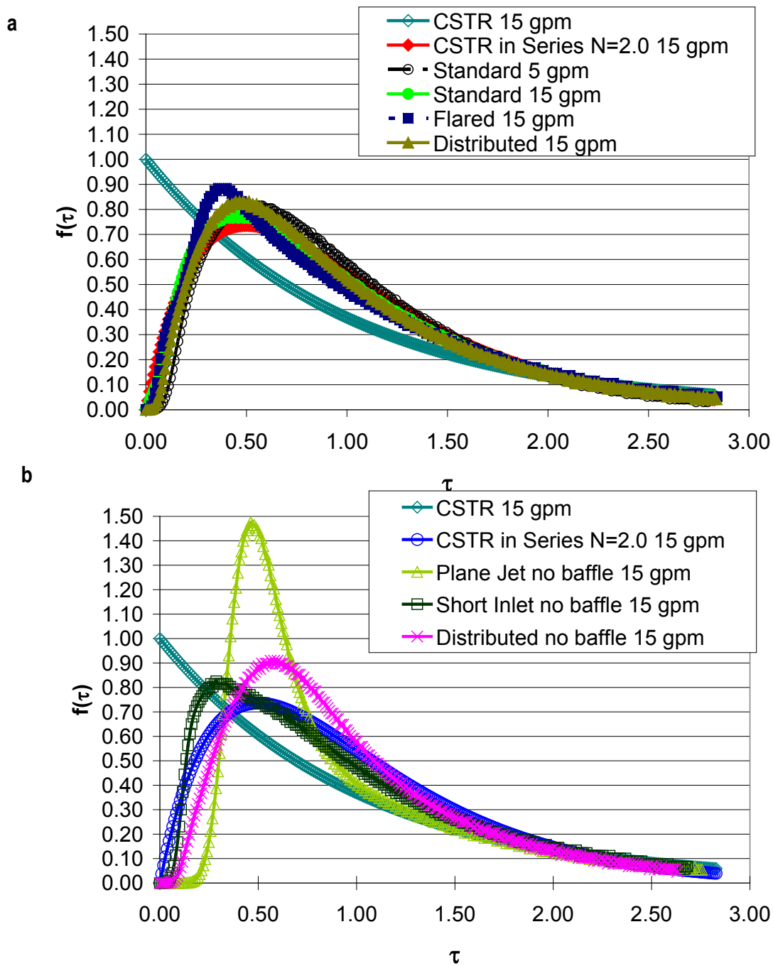
Figure 5-34. Tracer Test Simulations for the Different Configurations: a) Designs that Include a Mid-baffle Wall, b) Designs that Exclude a Mid-baffle Wall.
