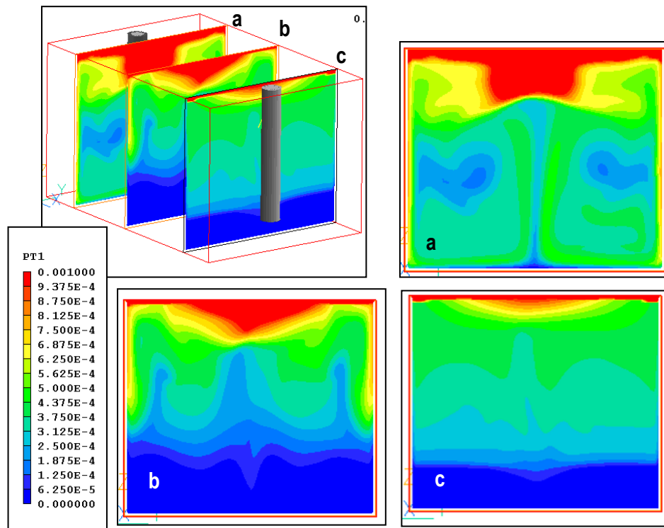
Figure 5-31. 15gpm Distributive Inlet/No Baffle Configuration Image Showing Volume Fraction of Oil (Contours) for ASM Simulation.
