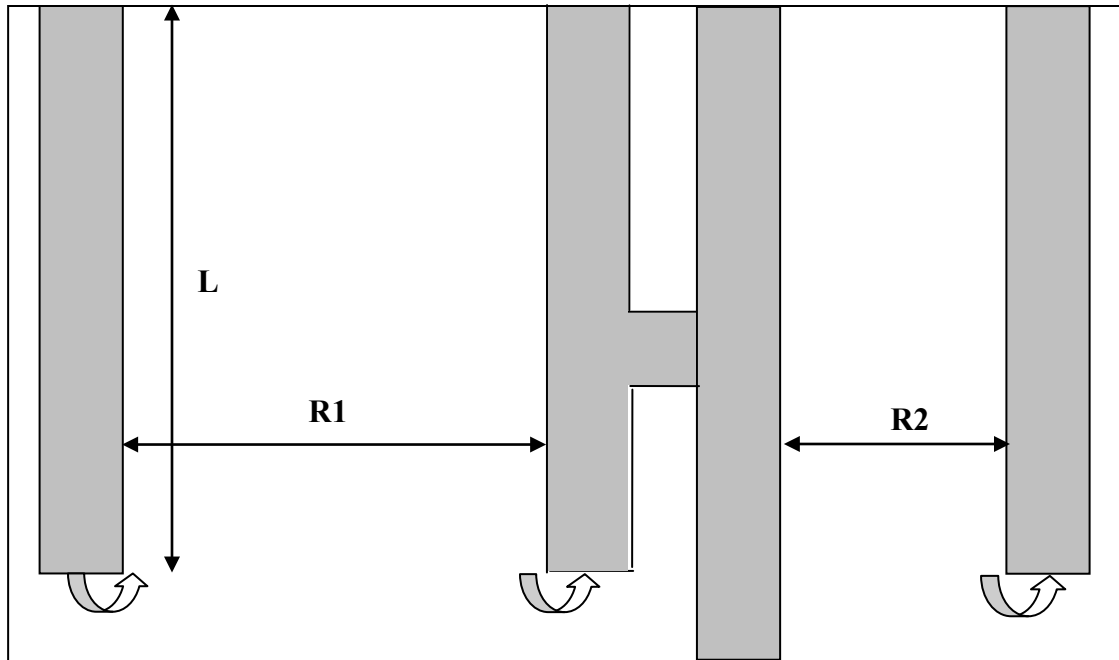
Figure 5-14. Layout of 2D GI Simulations with Variable Descriptions.
