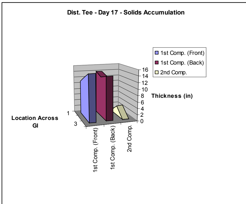
Figure 4-21. Day 13 and 17 Solids Thickness Profile in Distributive Tee-inlet GI.
