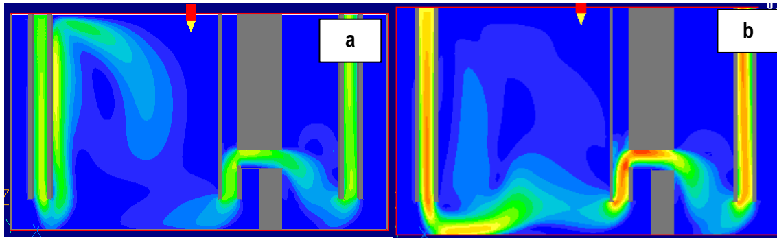
Figure 5-12. Comparison of Standard GI Simulation with 150 Micron a) and 80 Micron, b) Mean Droplet Distributions.
