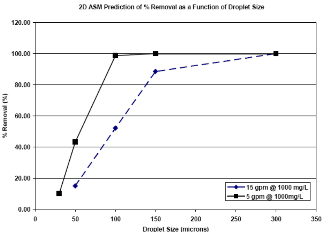
Figure 5-11. 2D Summary of Simulations Comparing % Removal w/ Droplet Size.
