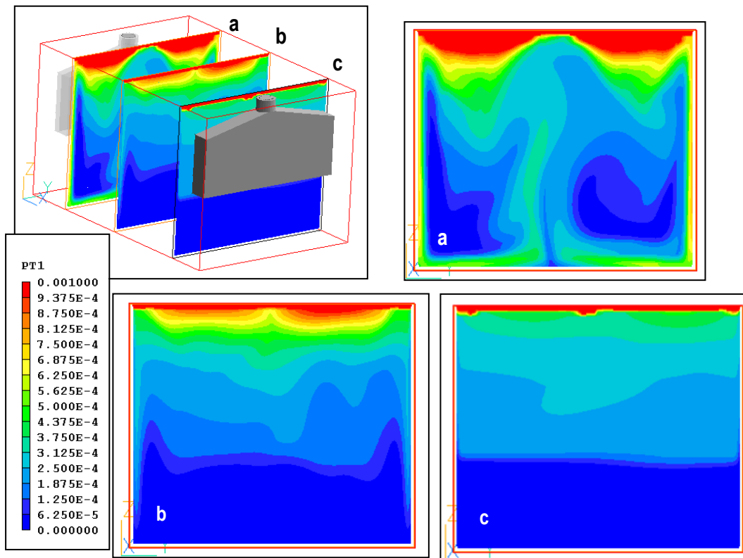
Figure 5-32. 15gpm Plane Jet Configuration Image Showing Volume Fraction of Oil (Contours) for ASM Simulation.
