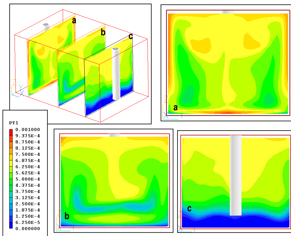
Figure 5-26. 15gpm Short Inlet/No Baffle Configuration Image Showing Volume Fraction of Oil (Contours) for ASM Simulation.
