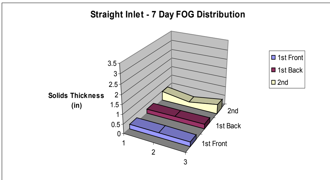
Figure 4-22. Day 5 and 7 FOG Thickness Profile in Straight Inlet GI.
