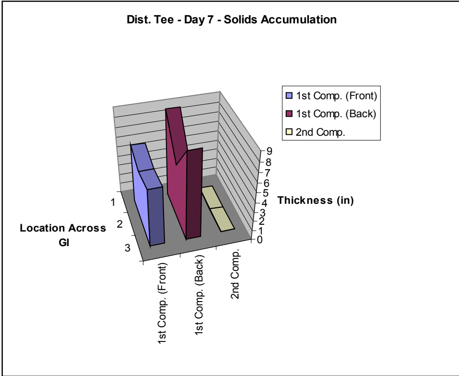
Figure 4-20. Day 3 and 7 Solids Thickness Profile in Distributive Tee-inlet GI.
