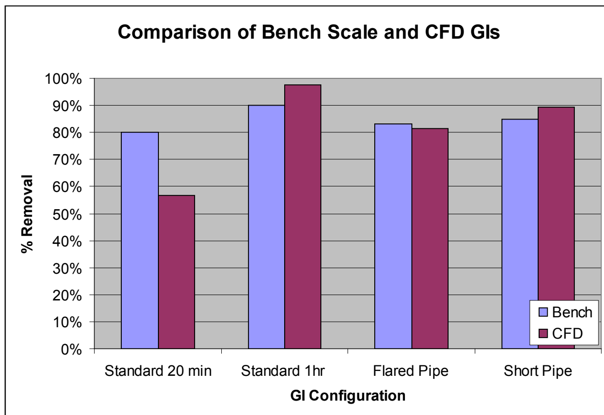
Figure 5-33. Comparison of Bench and CFD GIs.
