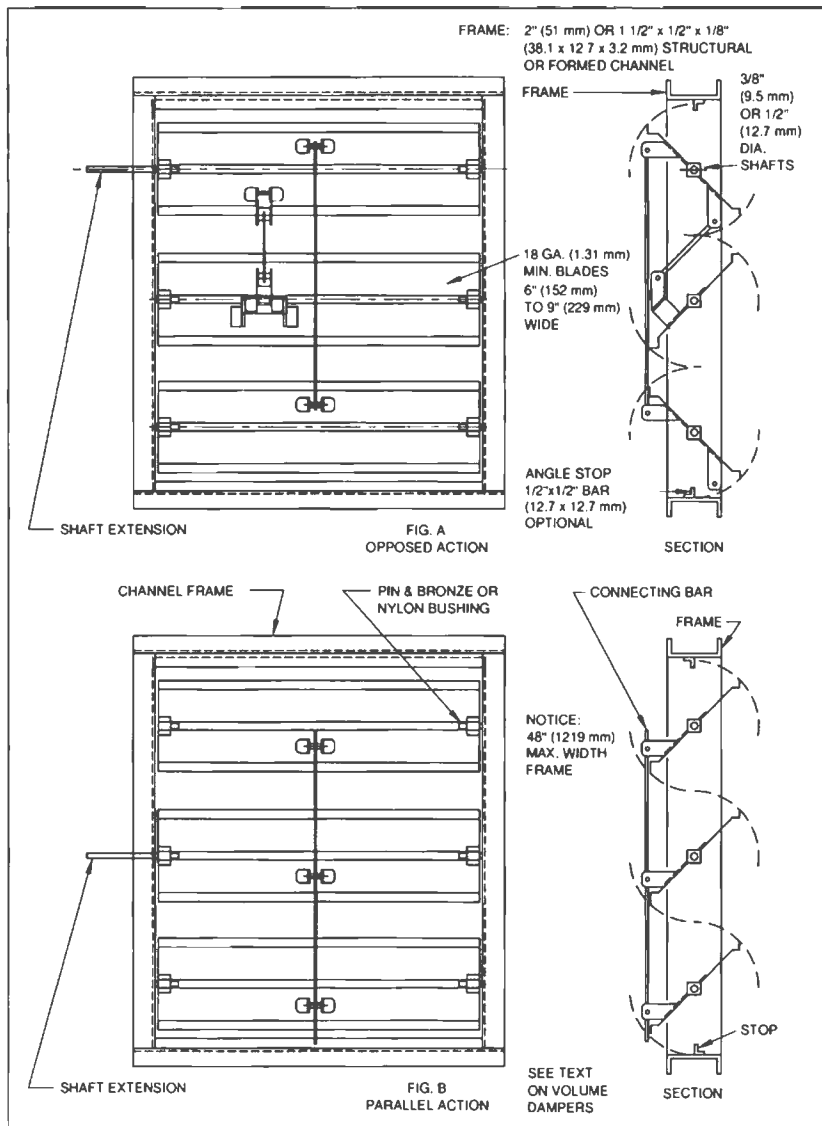
FIG. 2-13 MULTIBLADE VOLUME DAMPERS
