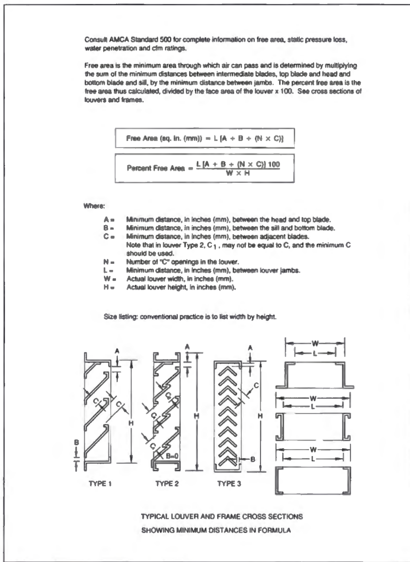
FIG. 5-2 LOUVER FREE AREA CALCULATION
