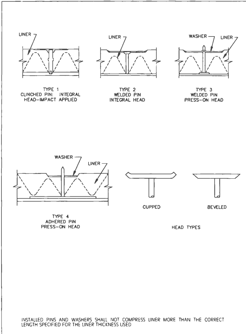
FIG. 2-20 LINER FASTENERS
