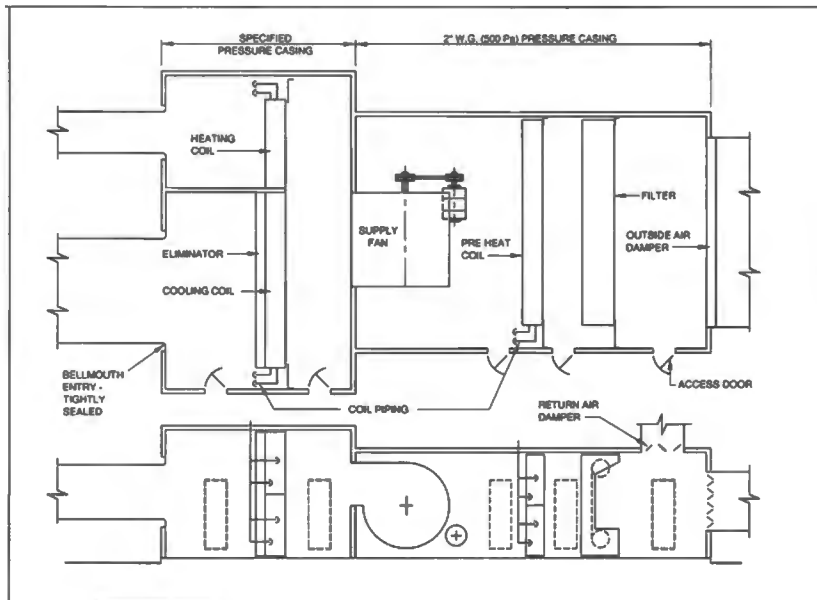
FIG. 6-4 OVER 2" W.G. CASING ARRANGEMENT
