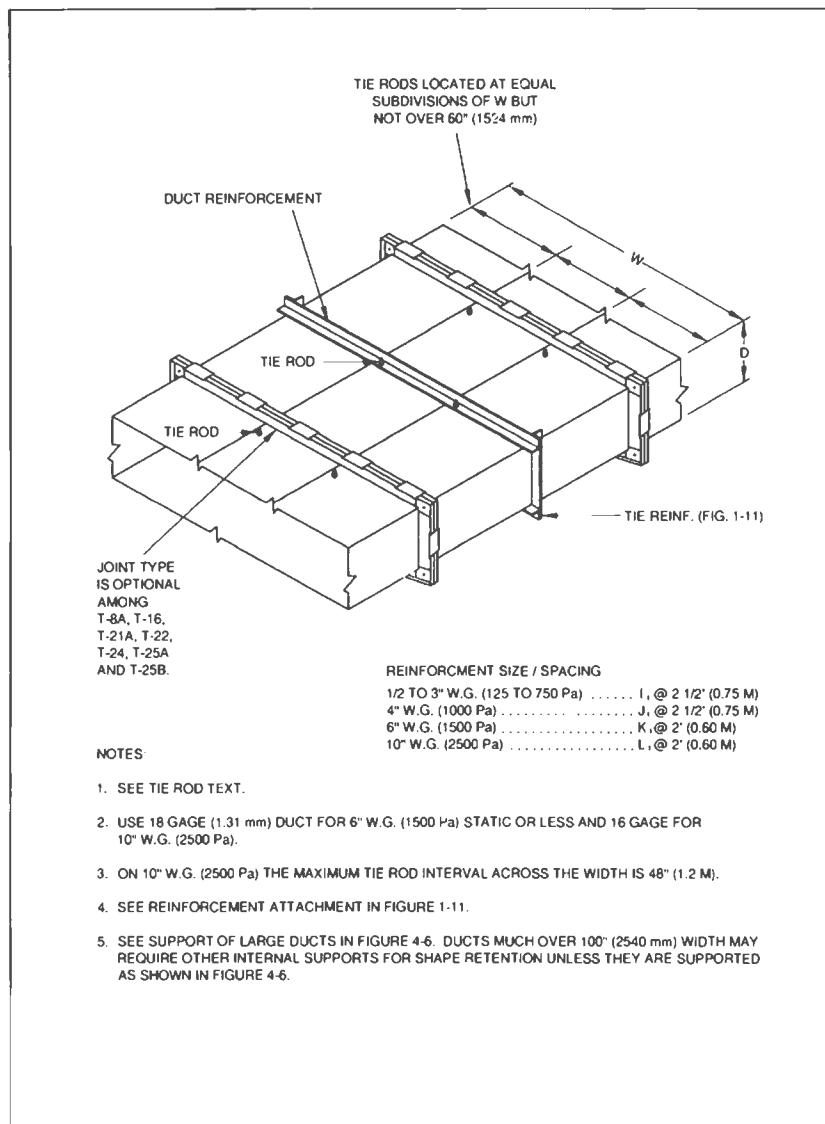
FIG. 1-12 DUCT OVER 120" (3048 mm) WIDE
