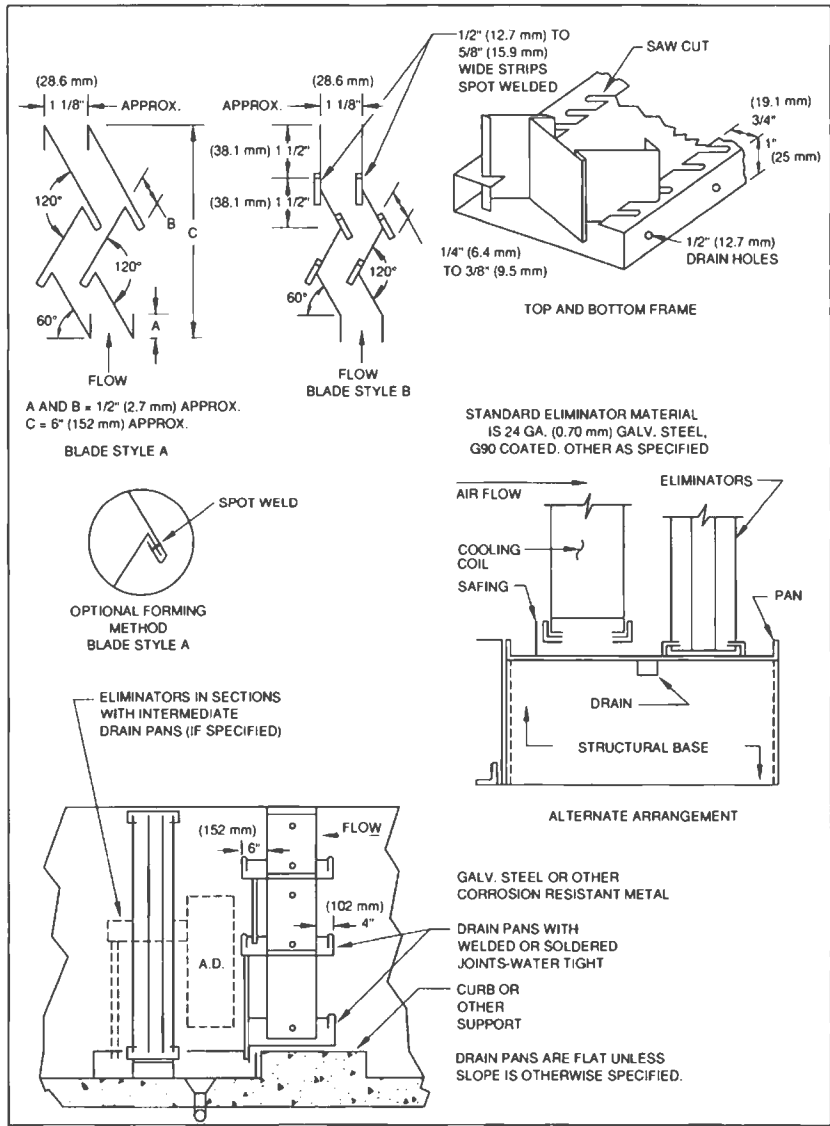
FIG. 6-9 ELIMINATORS AND DRAIN PANS
