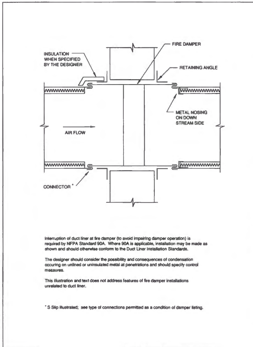
FIG. 2-22 DUCT LINER INTERRUPTION
