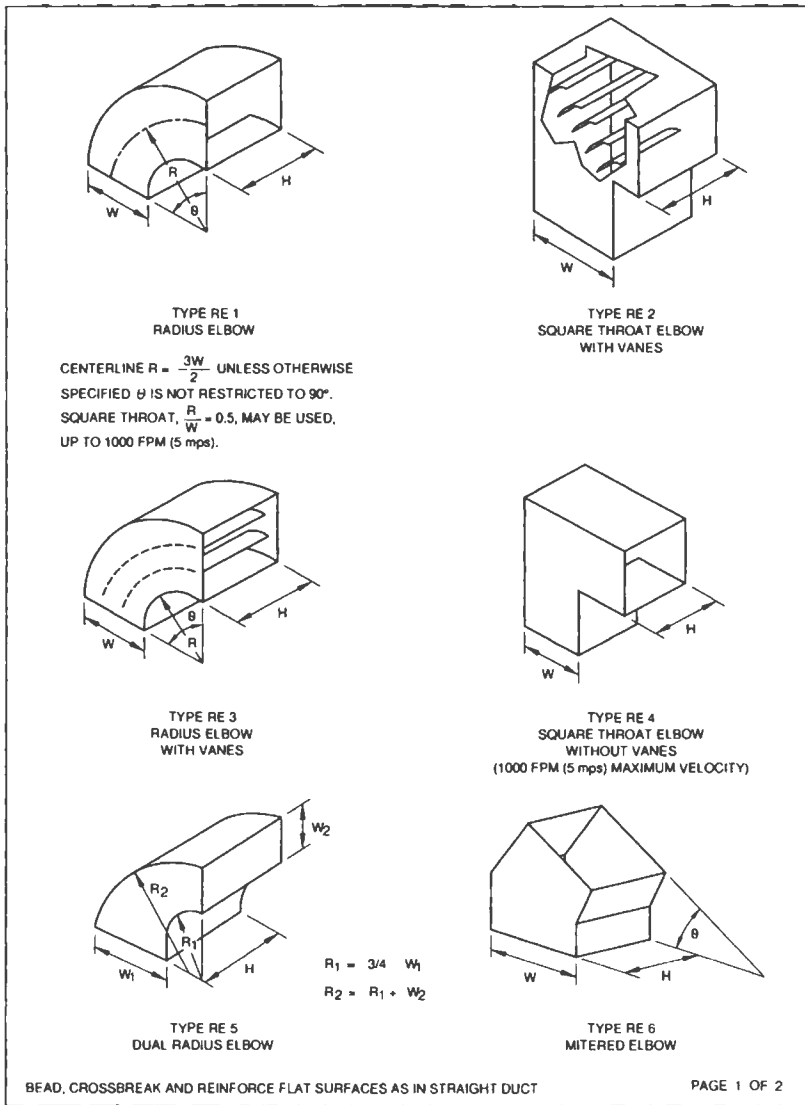
FIG. 2-2 RECTANGULAR ELBOWS
