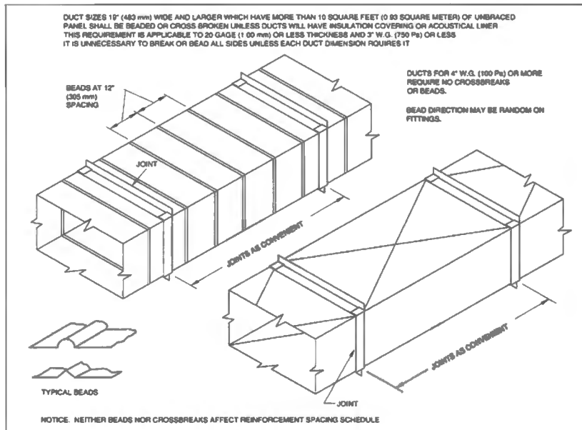
FIG. 1-8 CROSSBROKEN AND BEADED DUCT
