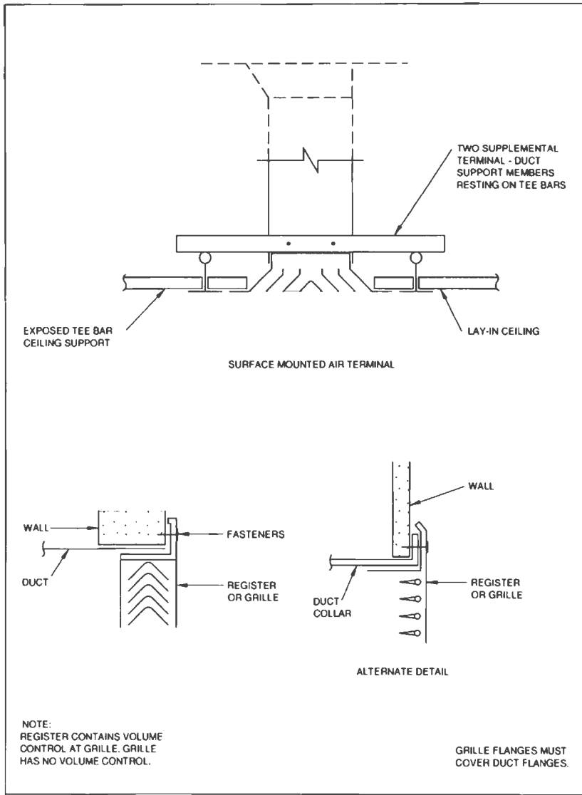
FIG. 2-14 GRILLE AND REGISTER CONNECTIONS
