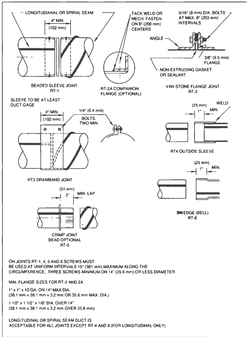
FIG. 3-2 TRANSVERSE JOINTS - ROUND DUCT
