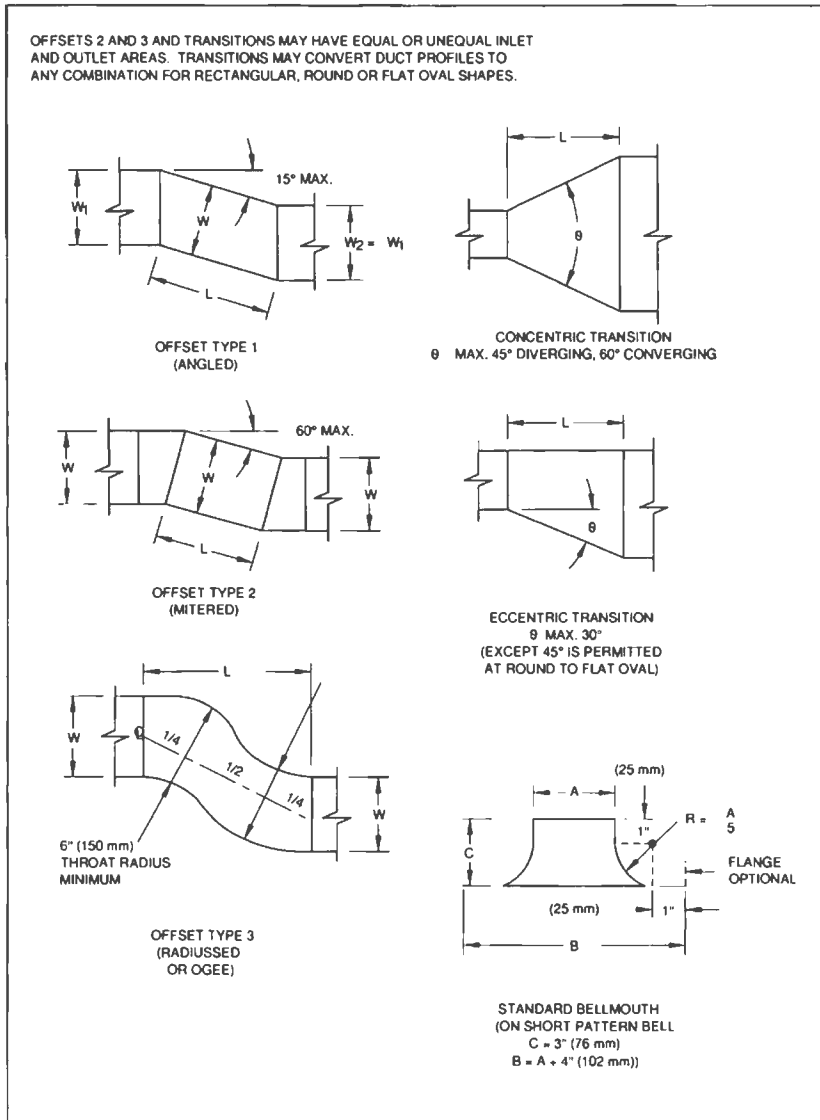
FIG. 2-7 OFFSETS AND TRANSITIONS
