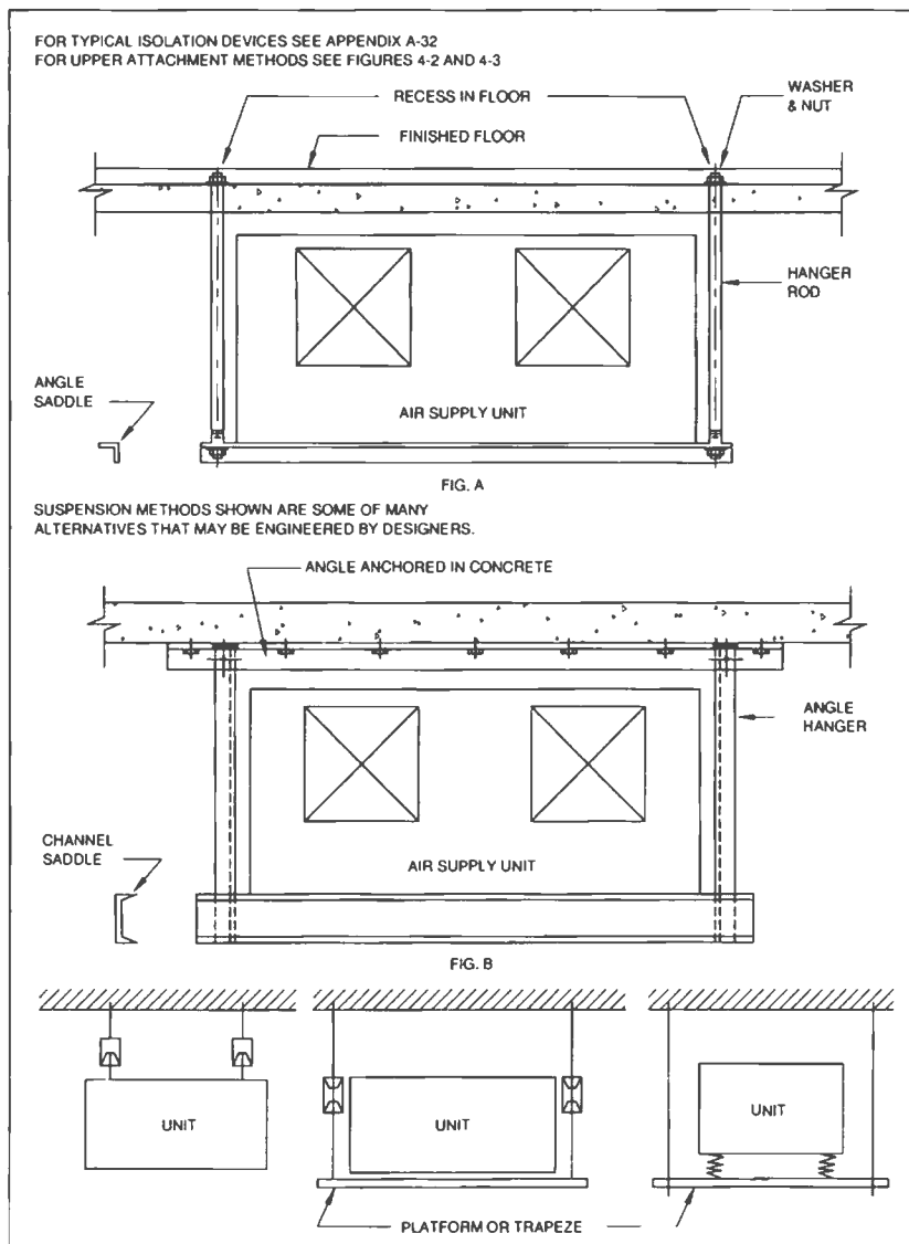
FIG. 4-10 HVAC UNIT SUSPENSION
