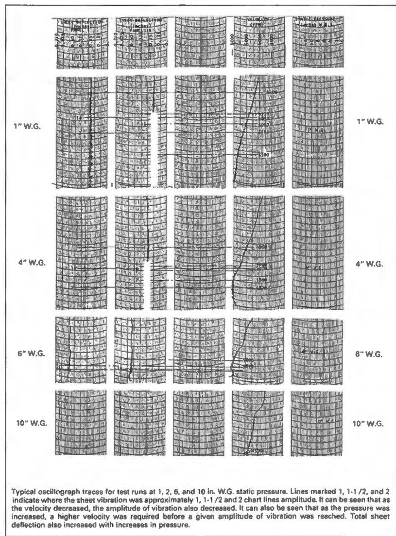
FIG. 7-5 OSCILLOGRAPH TRACES
