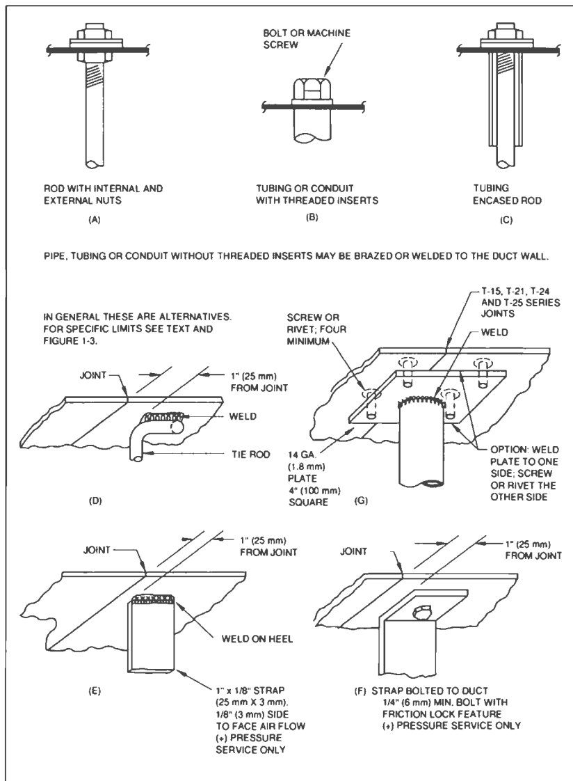
FIG. 1-2 TIE ROD ATTACHMENTS
