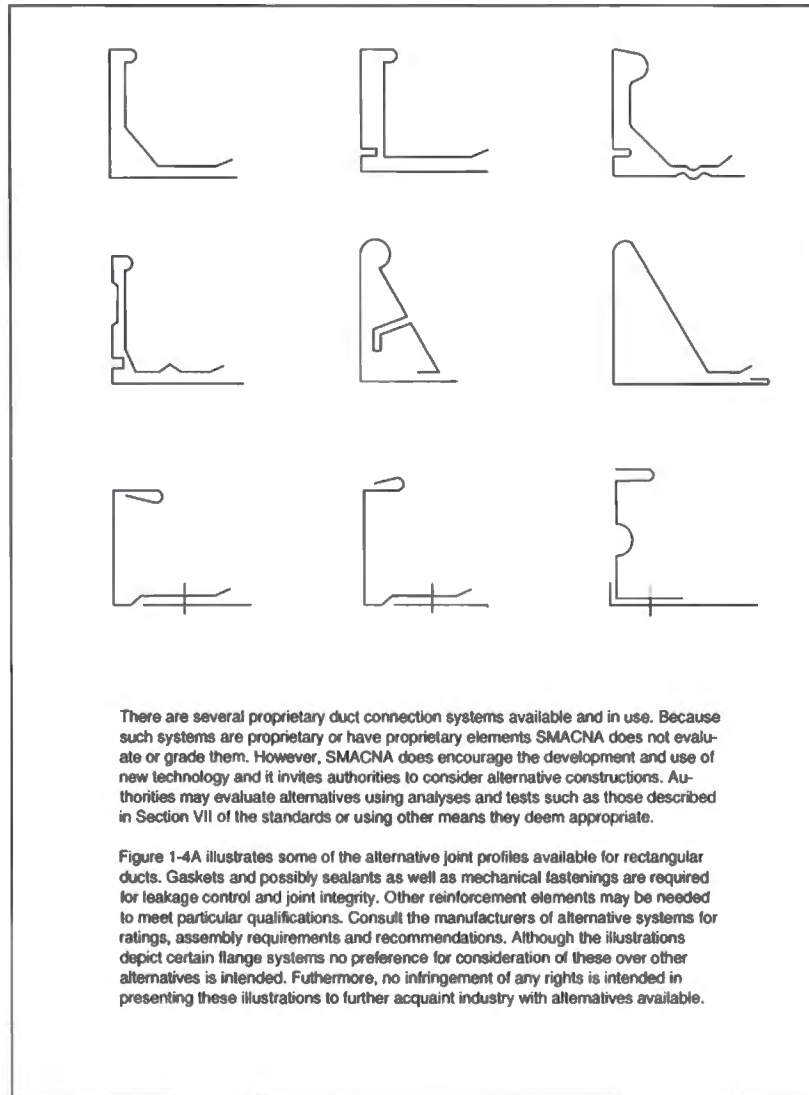
FIG. 1-4A SPECIAL JOINT PROFILES
