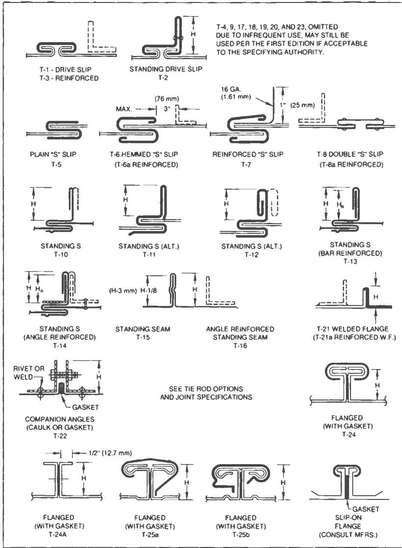
FIG. 1-4 TRANSVERSE (GIRTH) JOINTS
