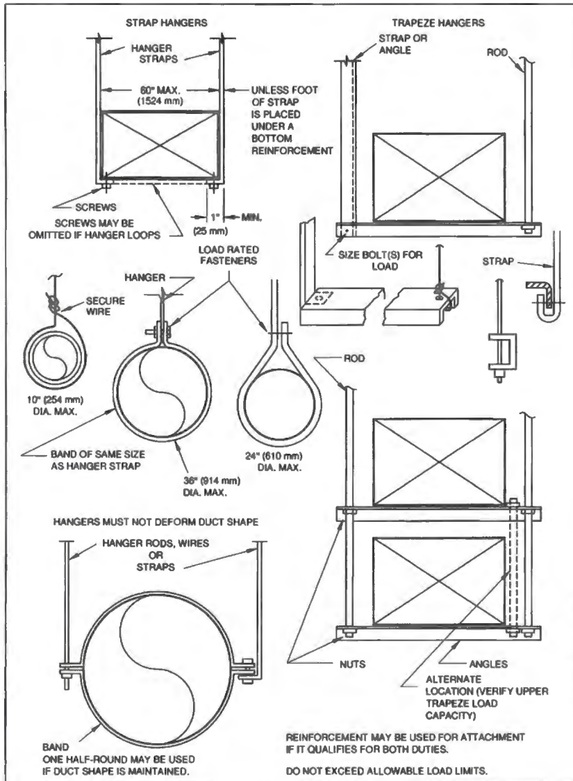
FIG. 4-4 LOWER HANGER ATTACHMENTS
