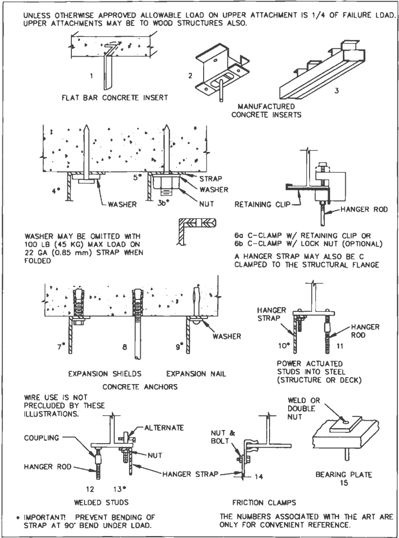
FIG. 4-2 UPPER ATTACHMENT DEVICES - TYPICAL
