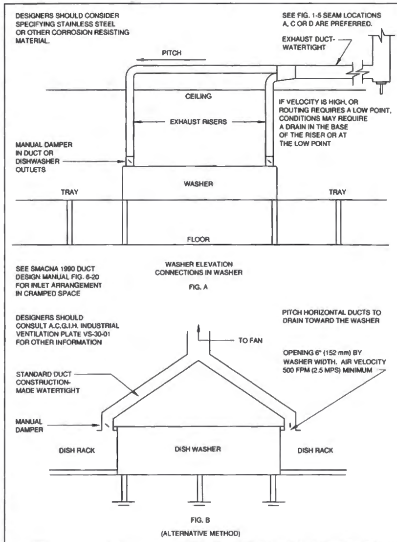
FIG. 2-18 DISH WASHER VAPOR EXHAUST
