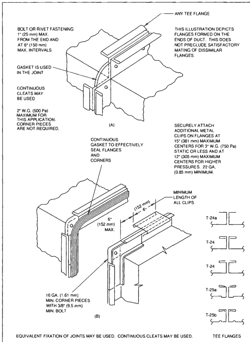
FIG. 1-15 CORNER CLOSURES - FLANGES
