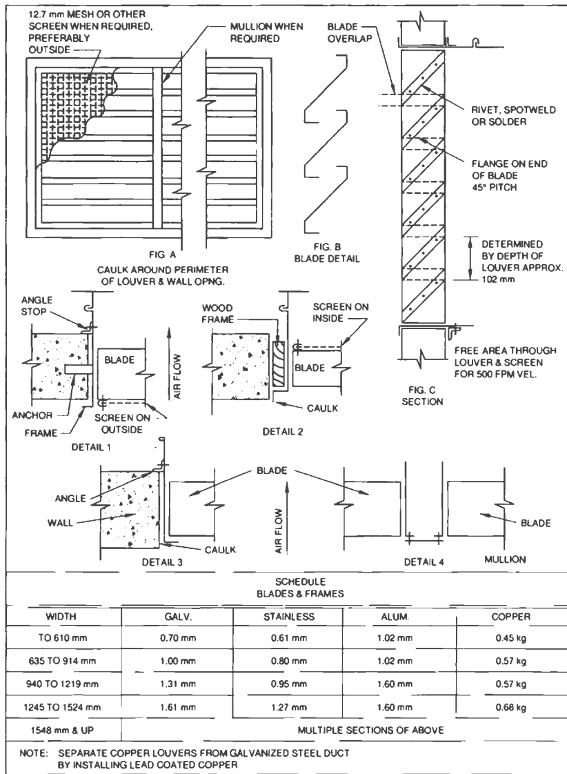
FIG. 5-1M LOUVERS AND SCREENS
