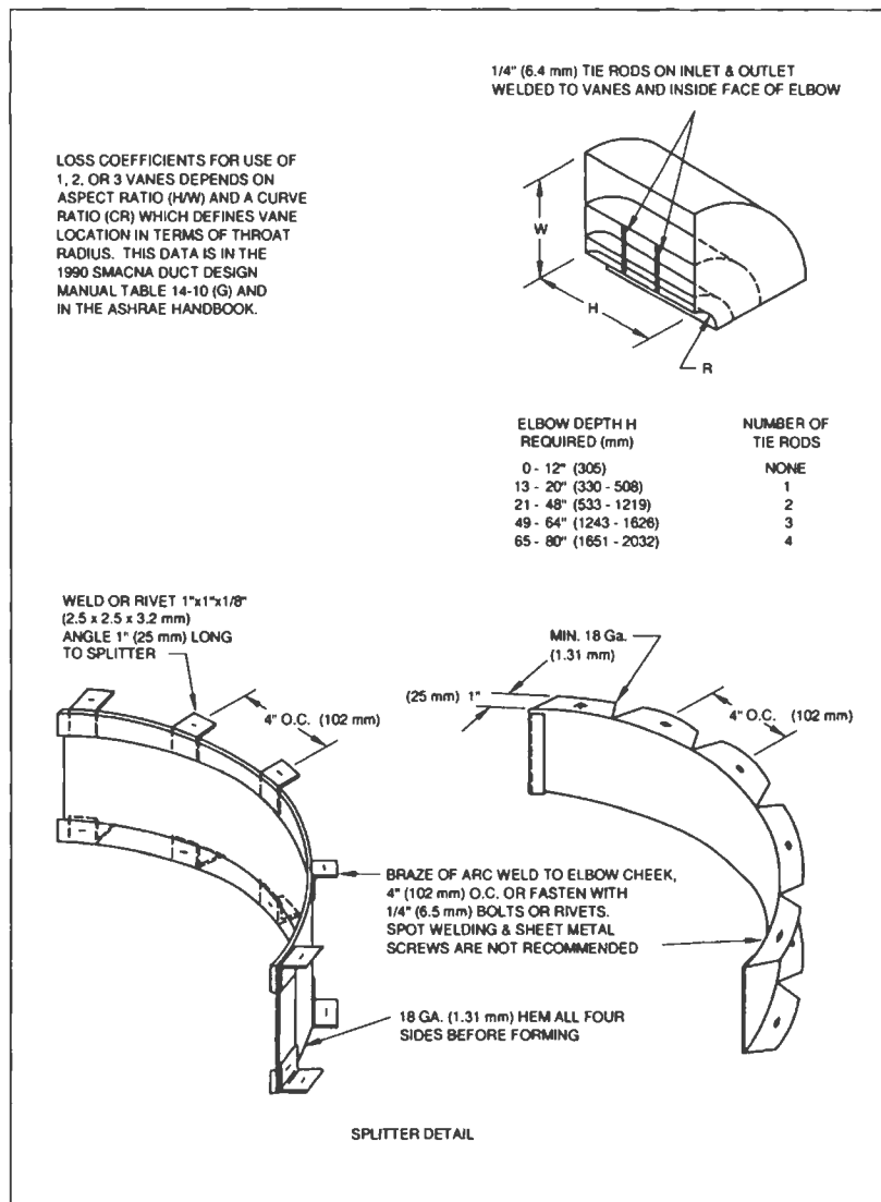
CONSTRUCTION OF SHORT RADIUS VANES
