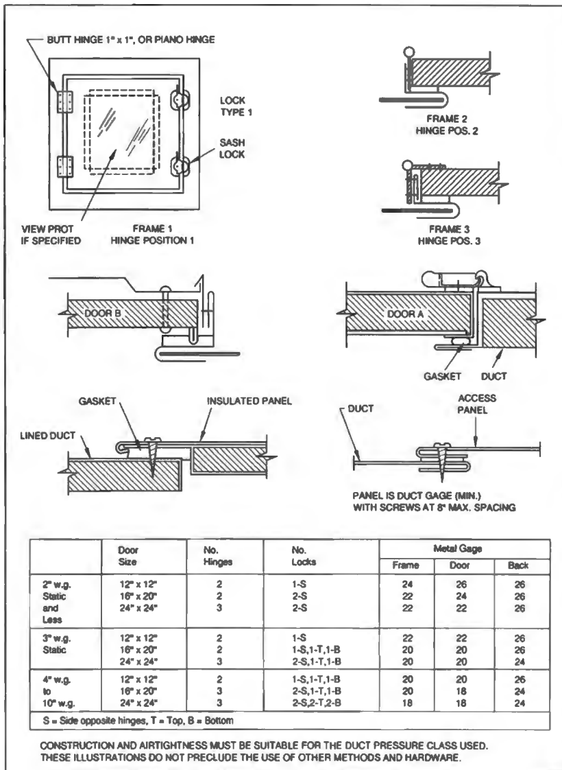
FIG. 2-10 DUCT ACCESS DOORS AND PANELS
