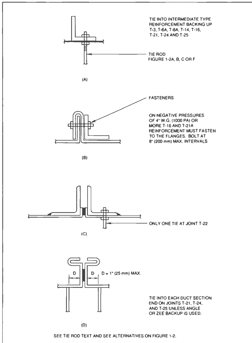
FIG. 1-3 TIE ROD ATTACHMENTS
