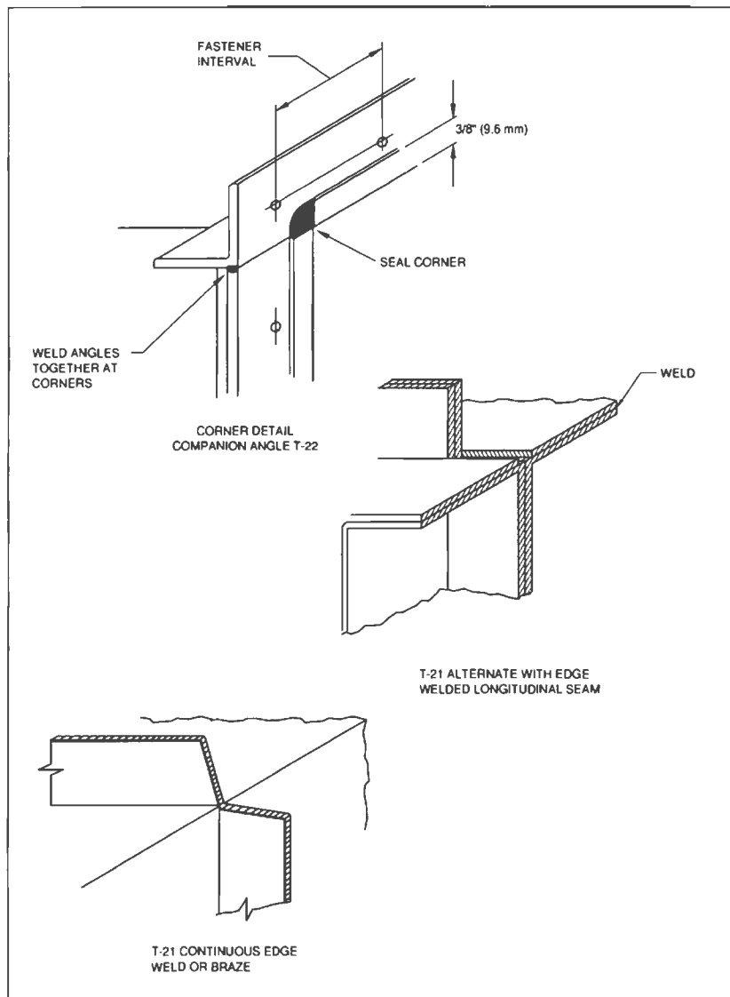
FIG. 1-14 CORNER CLOSURES - FLANGES
