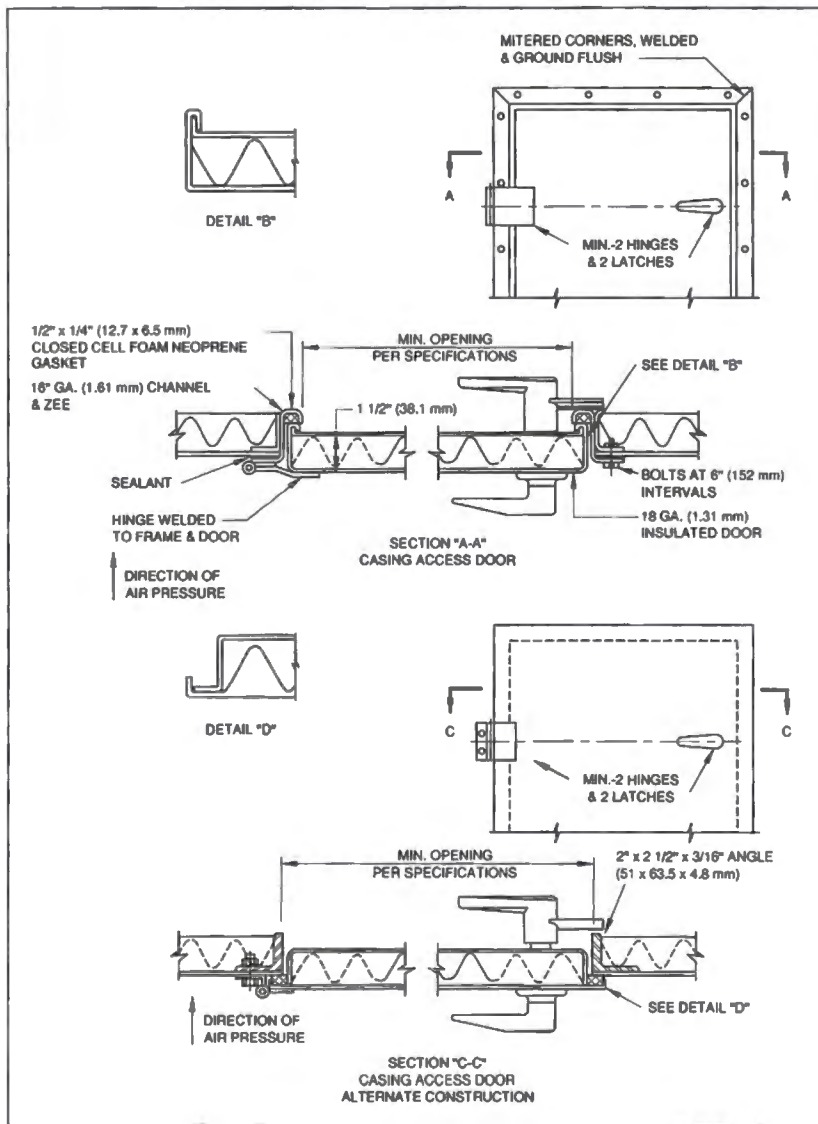
FIG. 6-12 CASING ACCESS DOORS - 3-10" W.G. (750-2500 Pa)
