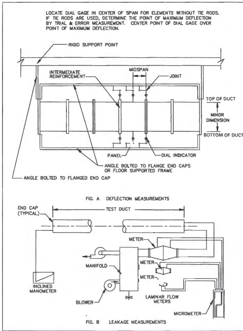
FIG. 7-3 DEFLECTION AND LEAKAGE MEASUREMENT
