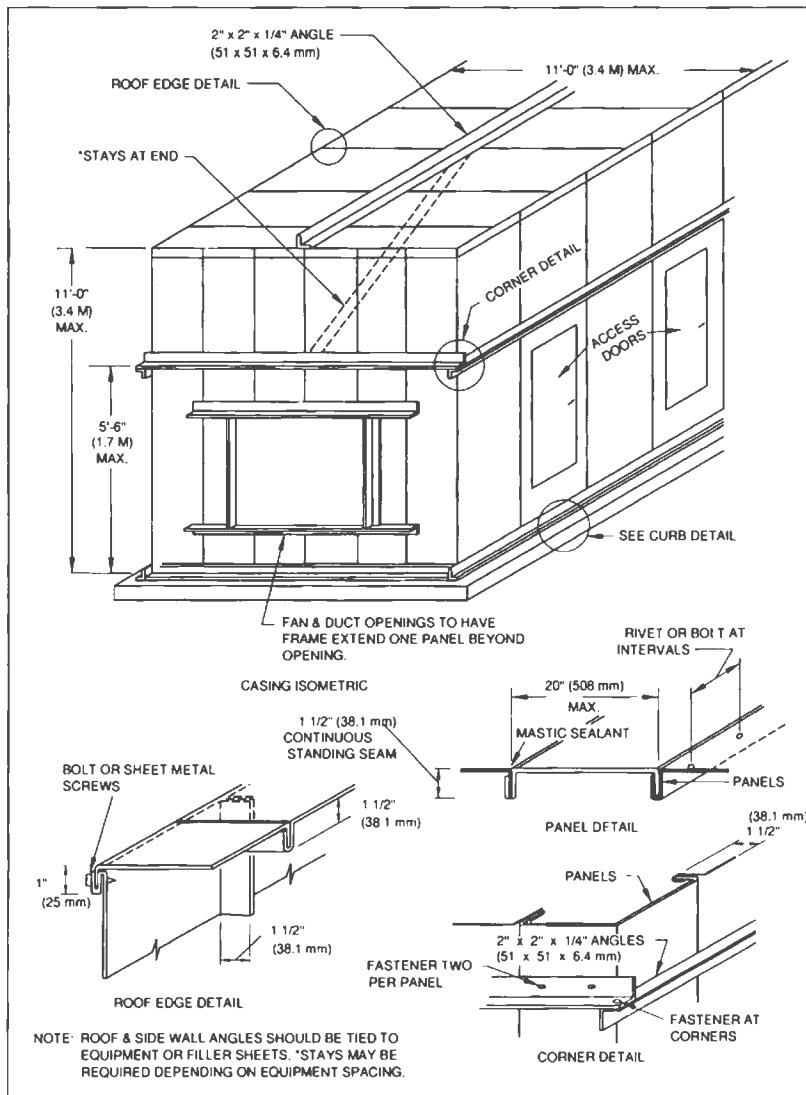
FIG. 6-6 INSIDE SEAM CASING - 6" W.G. (1500 Pa) MAX.
