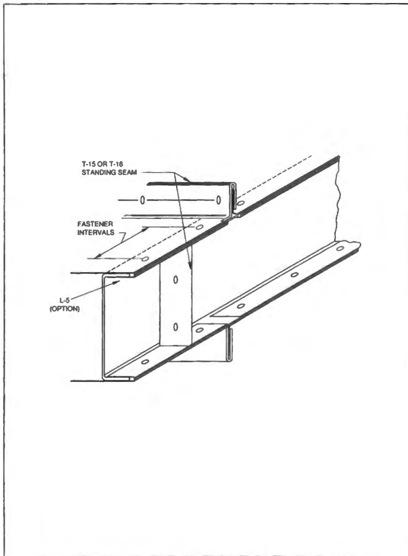
FIG. 1-16 CORNER CLOSURES - STANDING SEAMS
