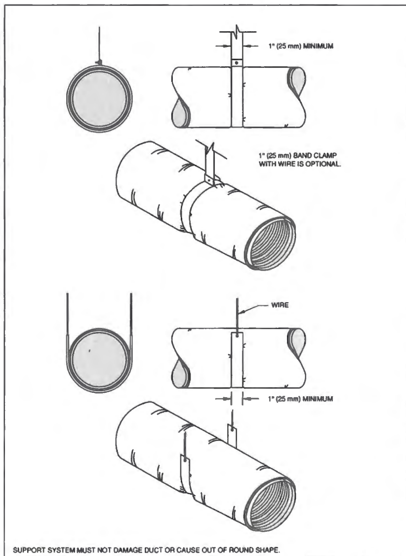
FIG. 3-10 FLEXIBLE DUCT SUPPORTS
