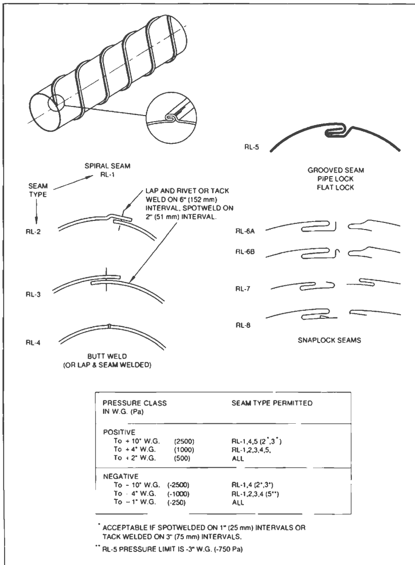
FIG. 3-1 SEAMS - ROUND DUCT AND FITTINGS
