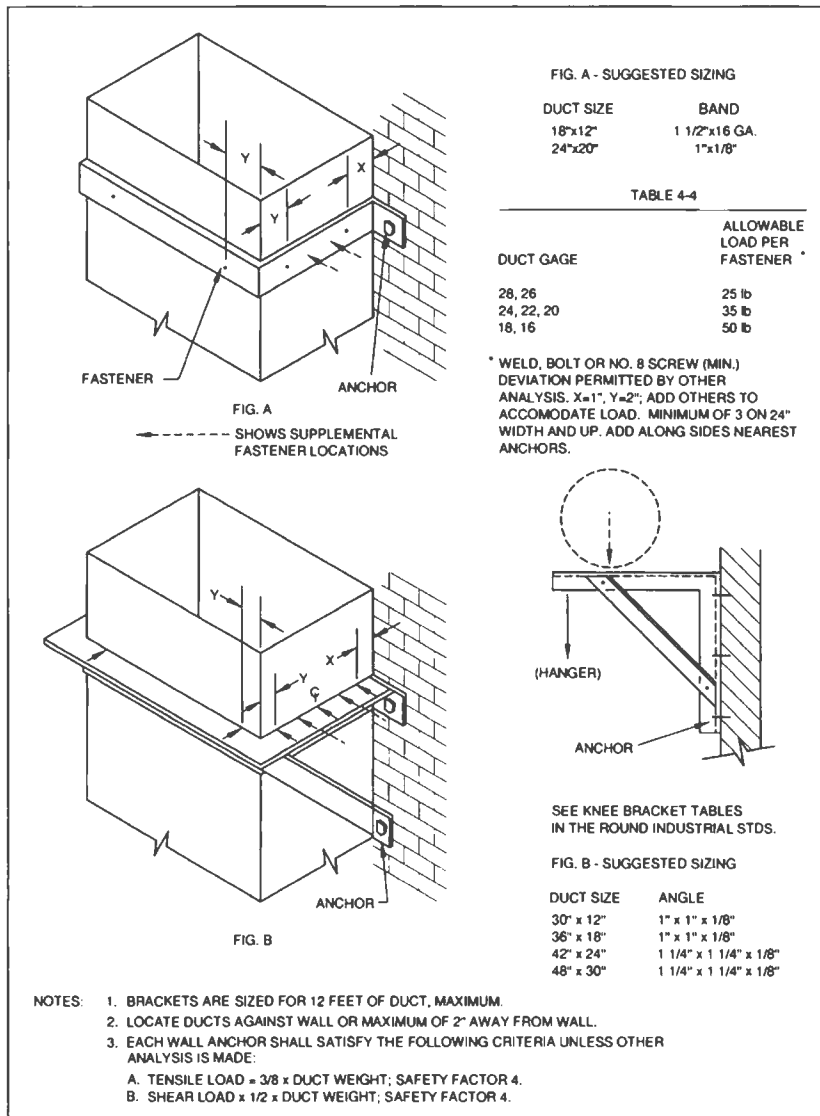
FIG. 4-8 SUPPORTS FROM WALL
