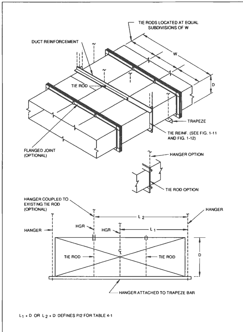
FIG. 4-6 LARGE DUCT SUPPORT
