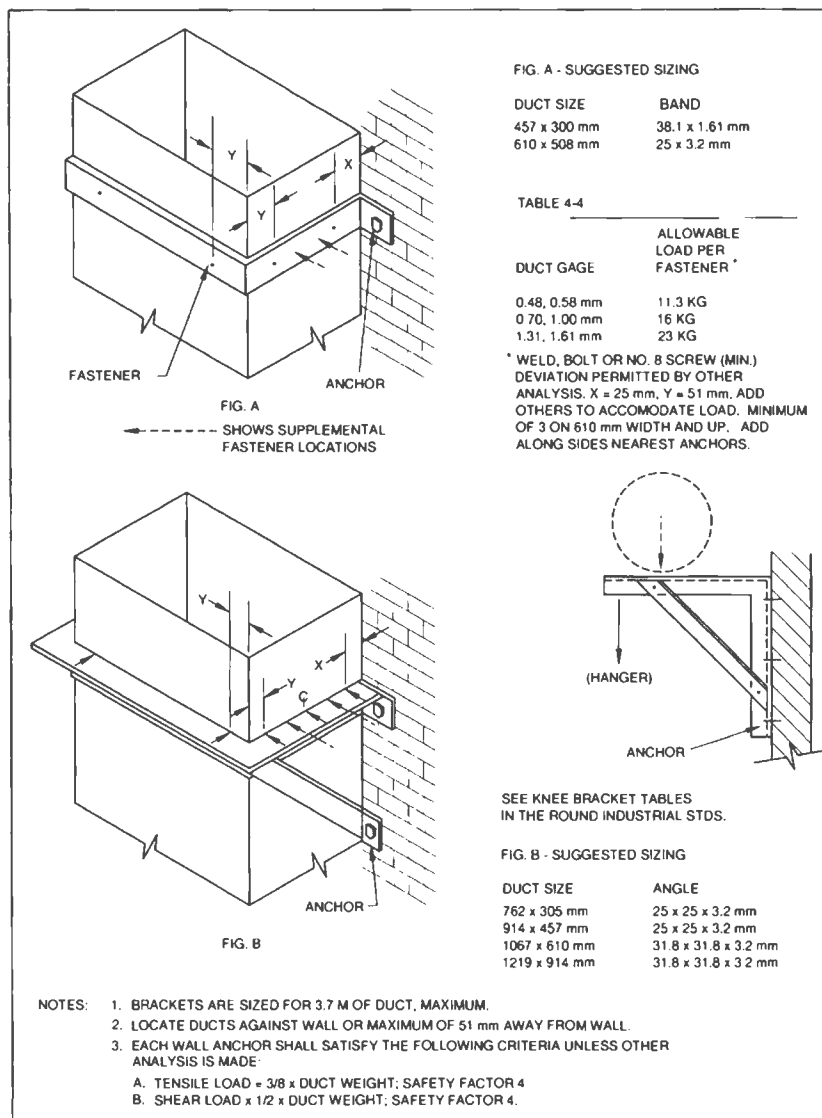
FIG. 4-8M SUPPORTS FROM WALL
