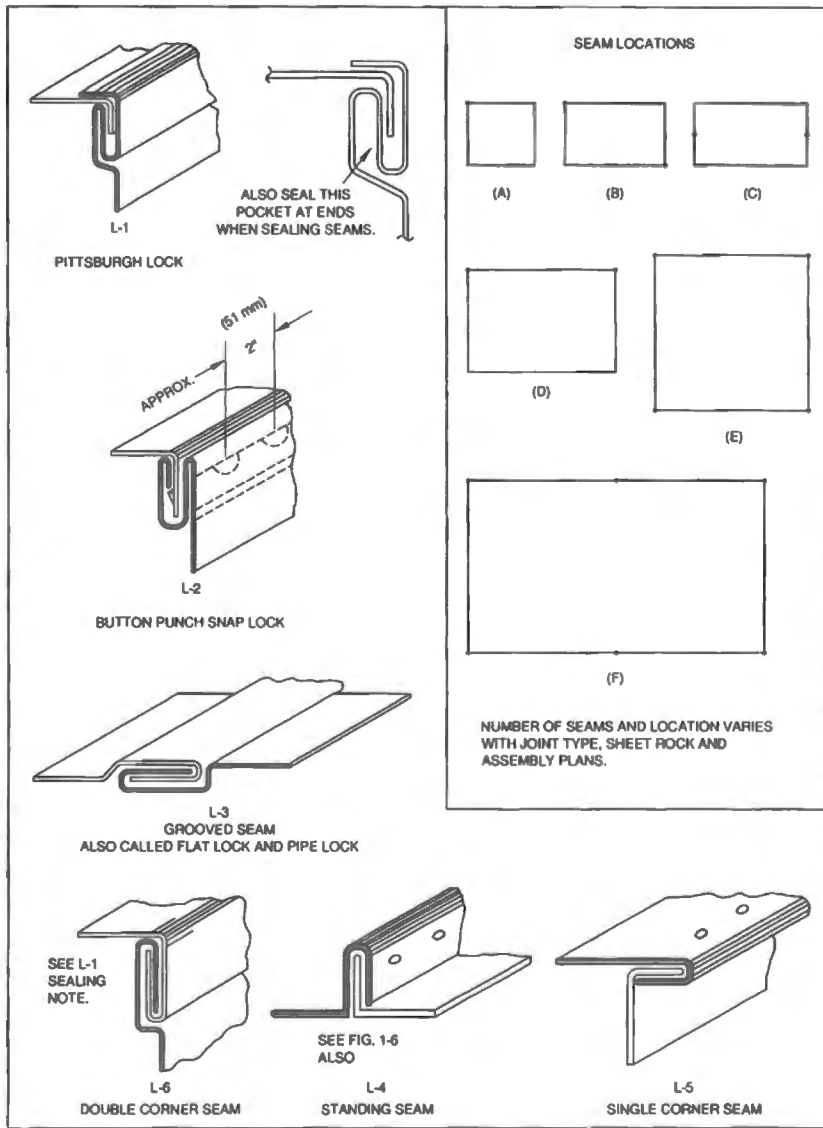
FIG. 1-5 LONGITUDINAL SEAMS - RECT. DUCT
