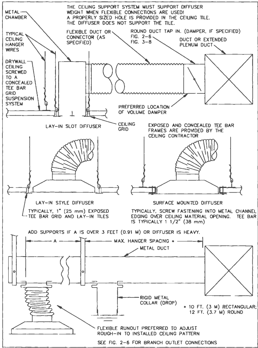
FIG. 2-15 CEILING DIFFUSER BRANCH DUCTS
