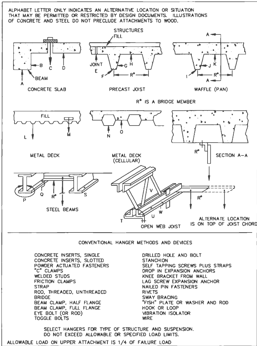
FIG. 4-1 HANGER ATTACHMENTS TO STRUCTURES
