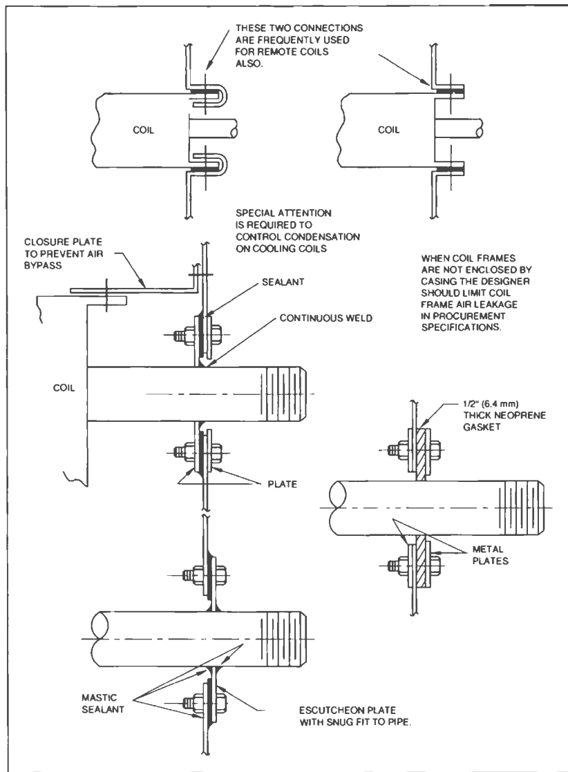
FIG. 6-10 PIPE PENETRATIONS OF CASINGS
