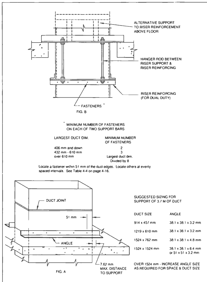
FIG. 4-7M RISER SUPPORTS - FROM FLOOR
