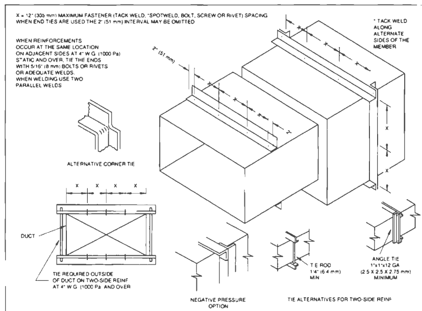
FIG. 1-11 REINFORCEMENT ATTACHMENT
