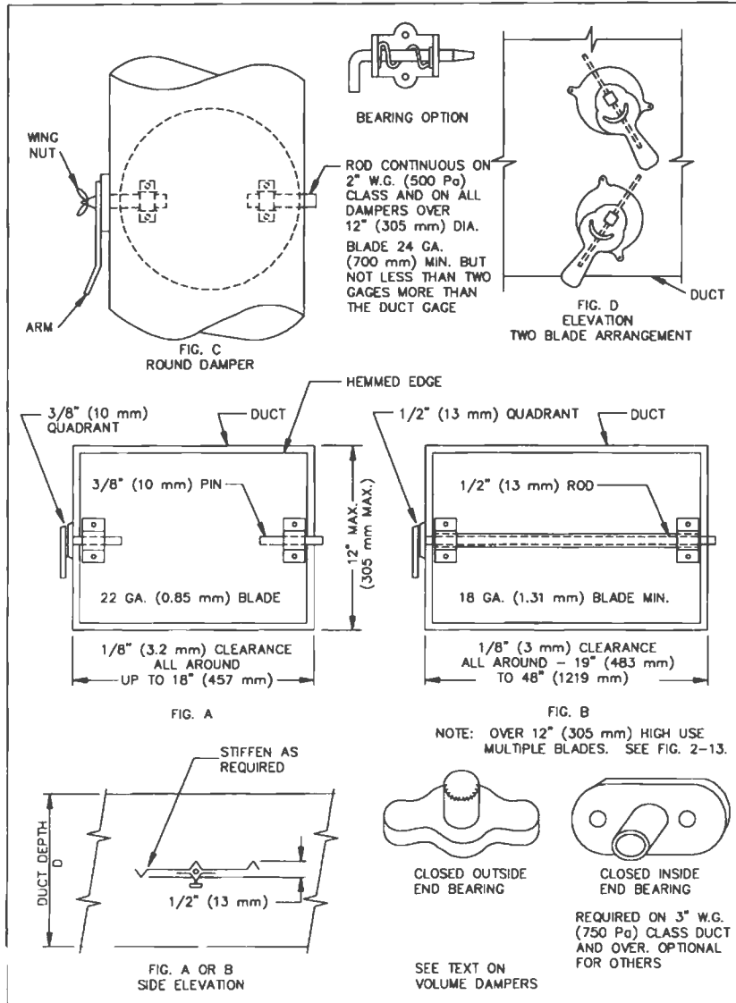
FIG. 2-12 VOLUME DAMPERS - SINGLE BLADE TYPE
