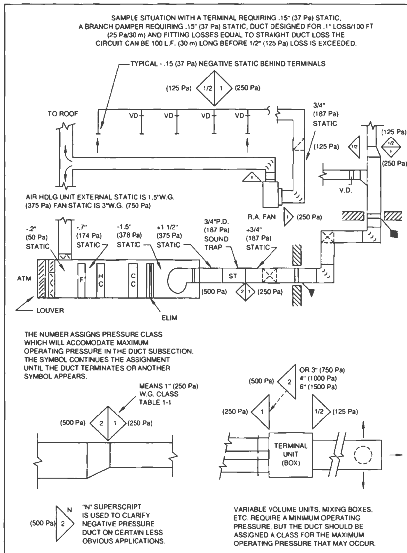
FIG. 1-1 DUCT PRESSURE CLASS DESIGNATION
