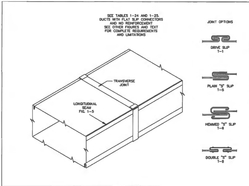
FIG. 1-7 UNREINFORCED DUCT
