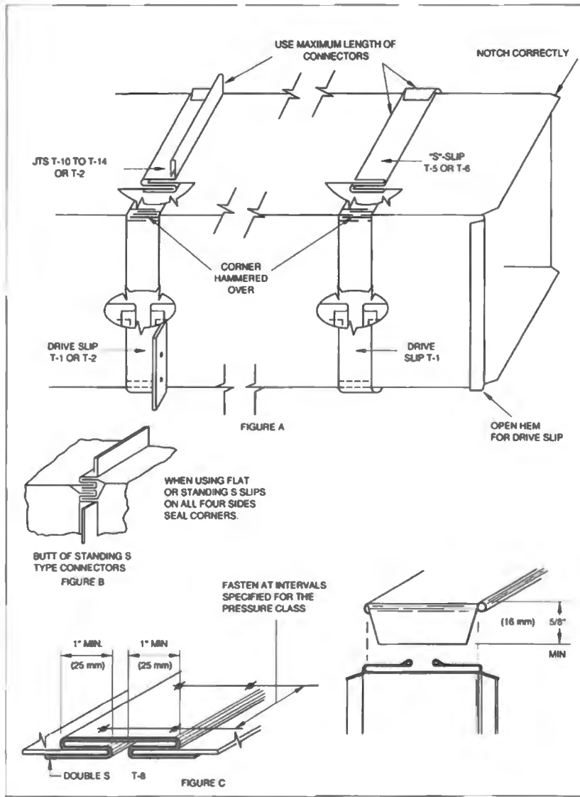
FIG. 1-13 CORNER CLOSURES - SLIPS AND DRIVES
