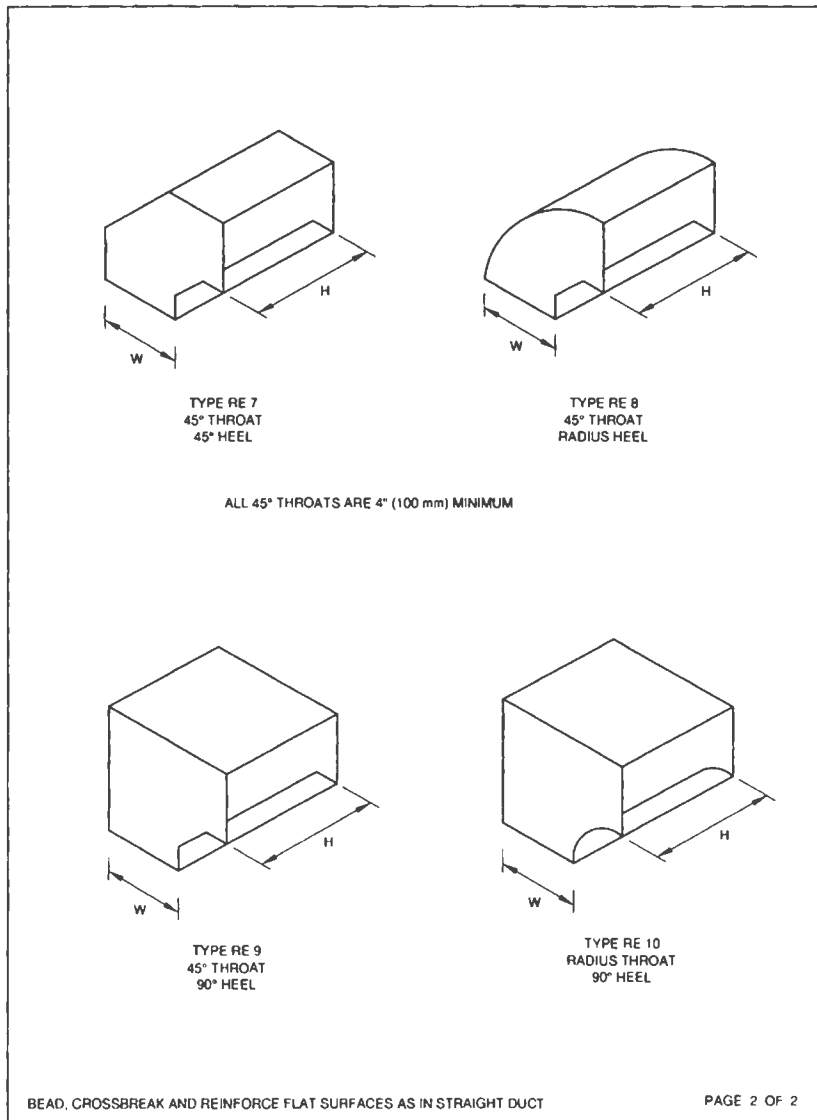
FIG. 2-2 RECTANGULAR ELBOWS
