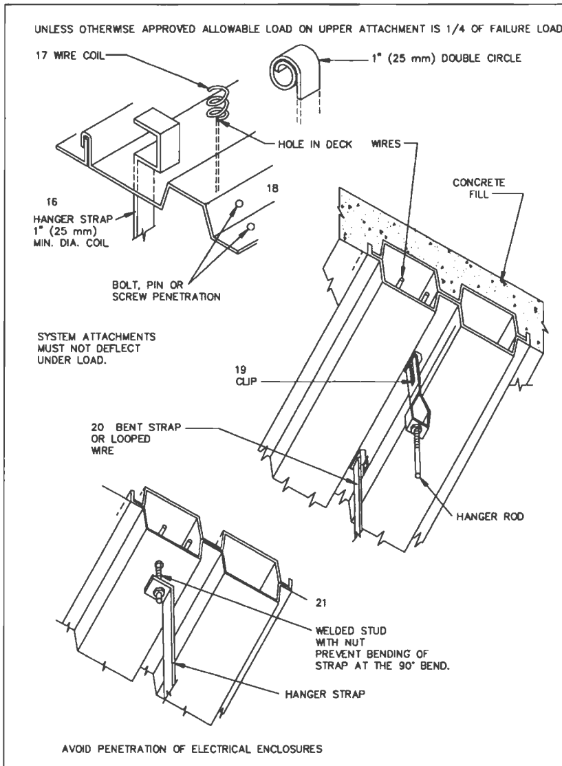
FIG. 4-3 UPPER ATTACHMENTS - TYPICAL
