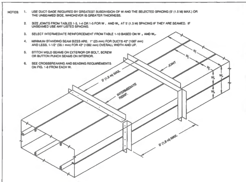
FIG. 1-6 INSIDE STANDING SEAM - LONGITUDINAL - 2" W.G. (500 Pa) MAXIMUM
