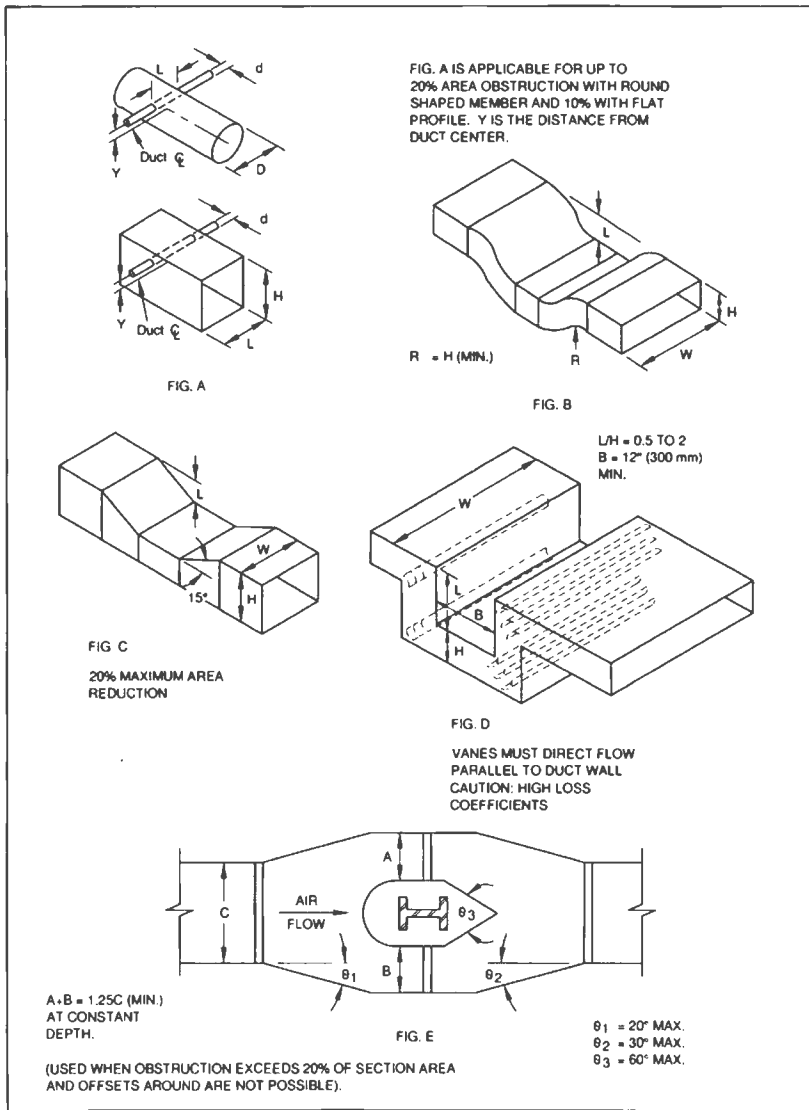
FIG. 2-8 OBSTRUCTIONS
