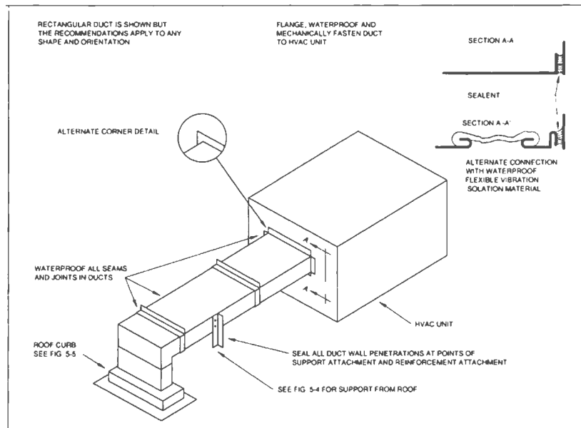
FIG. 5-3 ROOFTOP DUCT INSTALLATION
