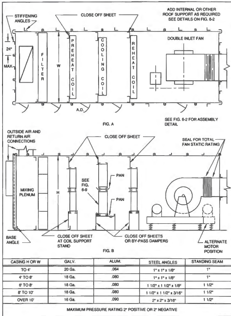
FIG. 6-1 BUILT-UP STANDING SEAM CASING
