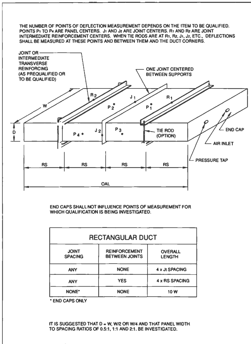
FIG. 7-2 TEST DUCT CONFIGURATION
