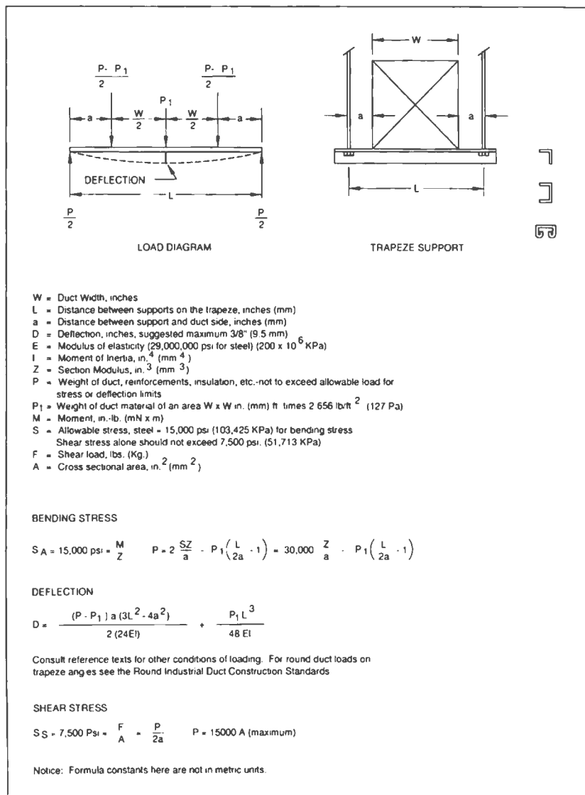
FIG. 4-5 TRAPEZE LOAD DIAGRAM
