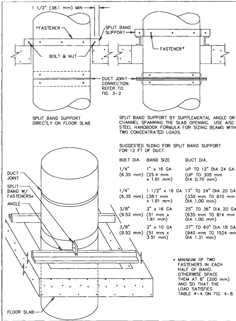
FIG. 4-9 RISER SUPPORT - FROM FLOOR
