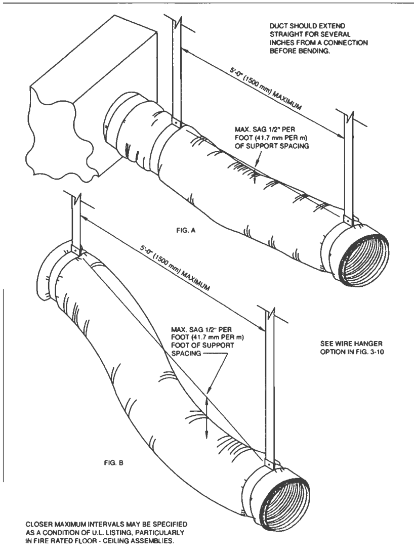
FIG. 3-9 FLEXIBLE DUCT SUPPORTS
