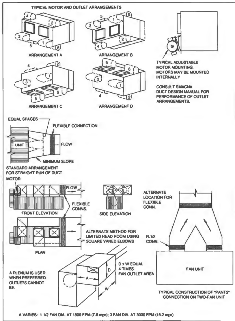
TYPICAL HVAC UNIT CONNECTIONS
