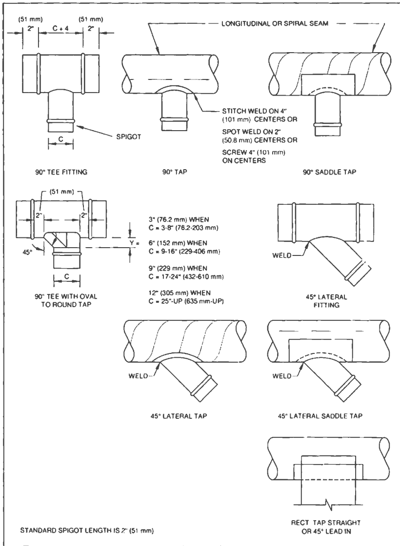
FIG. 3-4 90° TEES AND LATERALS
