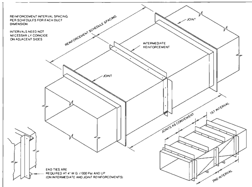
FIG. 1-10 DUCT REINFORCED ON ALL SIDES
