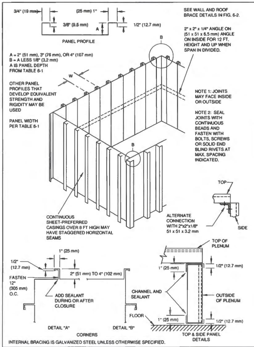
FIG. 6-3 ALTERNATE CASING CONSTRUCTION
