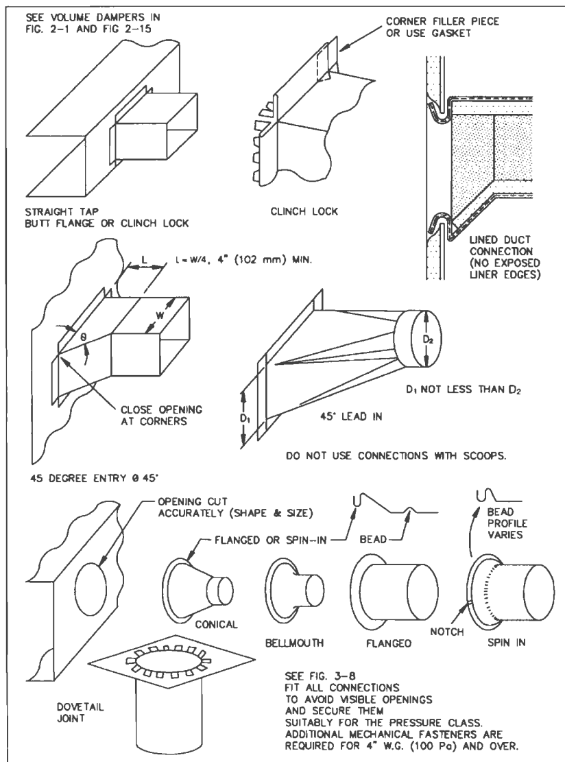
FIG. 2-6 BRANCH CONNECTIONS
