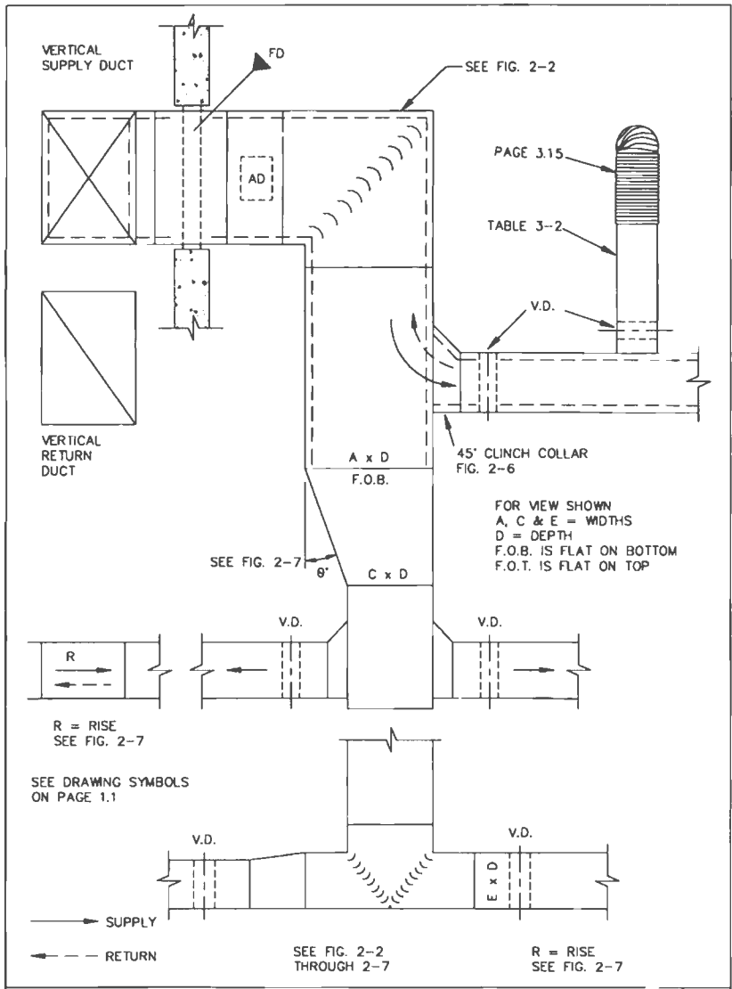
FIG. 2-1 TYPICAL SUPPLY OR RETURN DUCT
