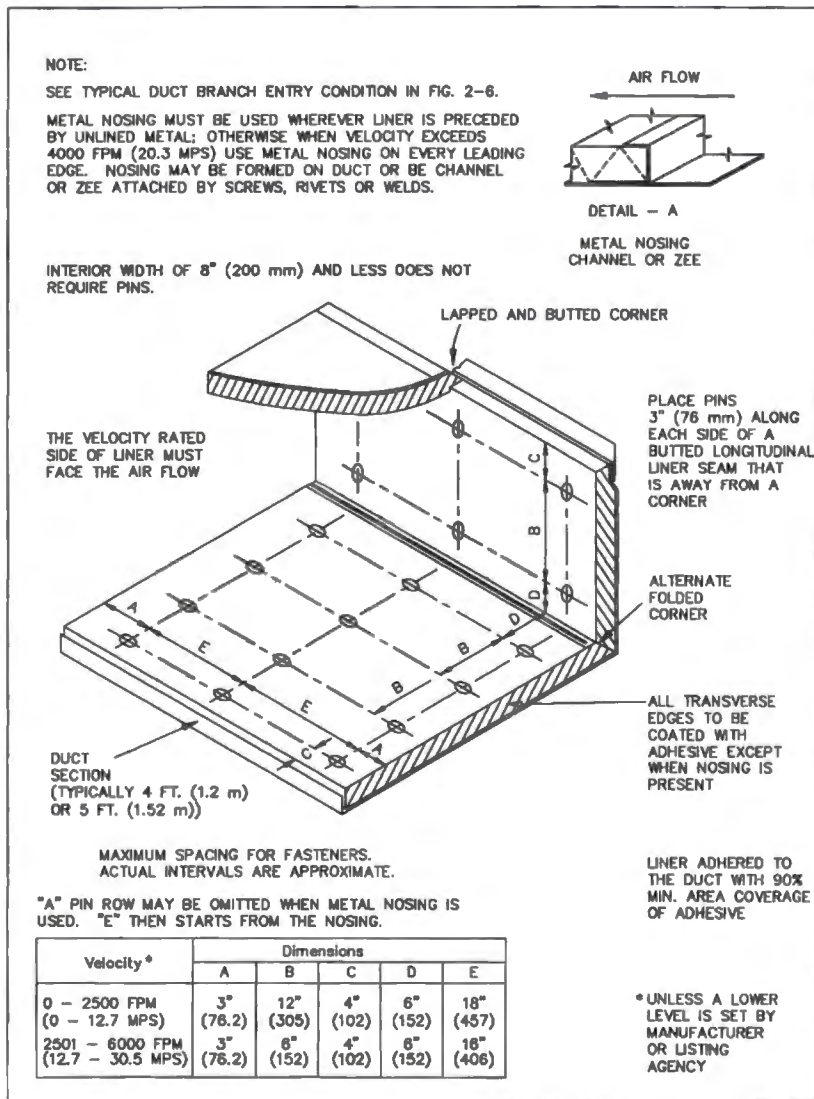
FIG. 2-19 FLEXIBLE DUCT LINER INSTALLATION
