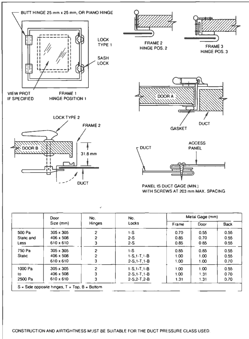
FIG. 2-10M DUCT ACCESS DOORS AND PANELS
