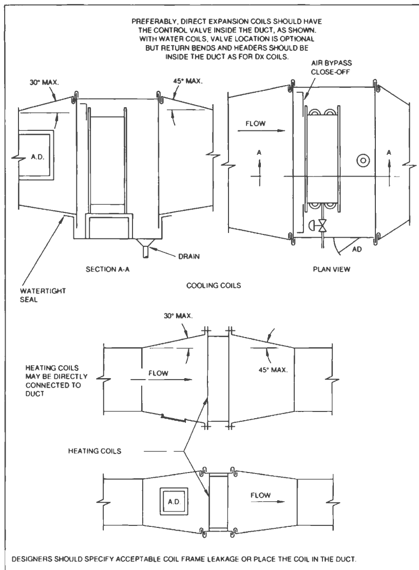
FIG. 2-9 REMOTE HEATING AND COOLING COIL INSTALLATIONS
