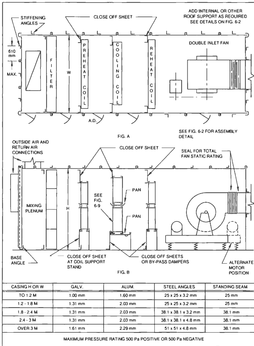
FIG. 6-1M BUILT-UP STANDING SEAM CASING
