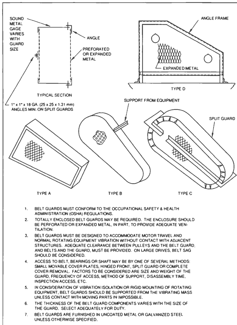
TYPICAL BELT GUARDS
