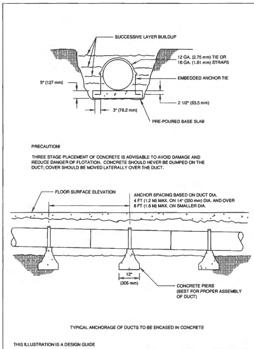
FIG. 3-12 ANCHORS FOR DUCT ENCASEMENT
