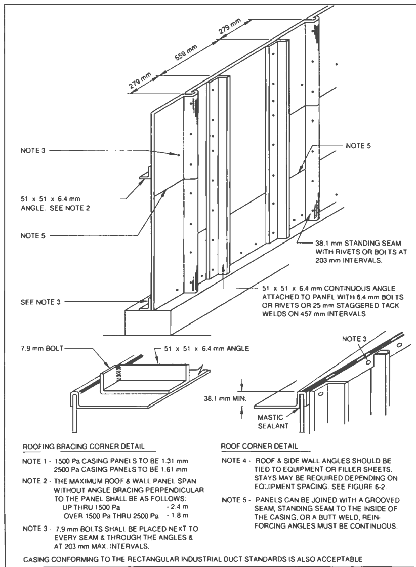
FIG. 6-5M OVER 500 Pa PRESSURE APPARATUS CASING
