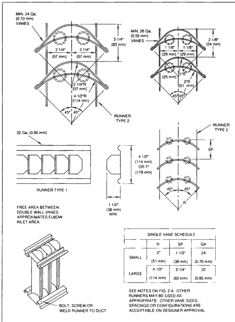
FIG. 2-3 VANES & VANE RUNNERS
