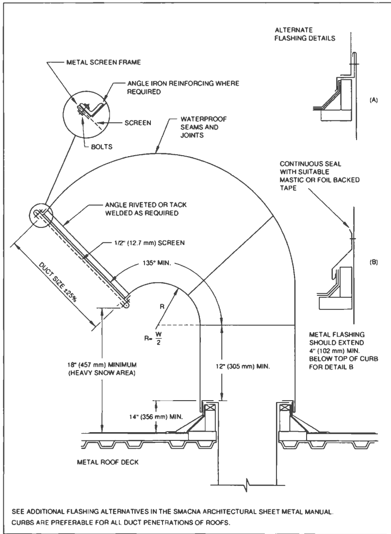
FIG. 5-5 RECTANGULAR GOOSENECK
