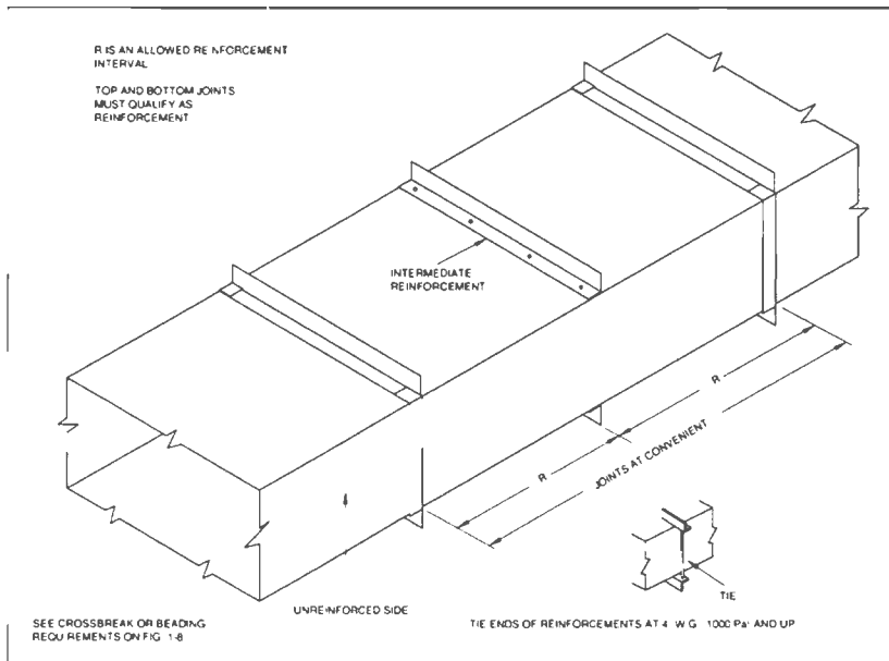
FIG. 1-9 DUCT REINFORCED ON TWO SIDES
