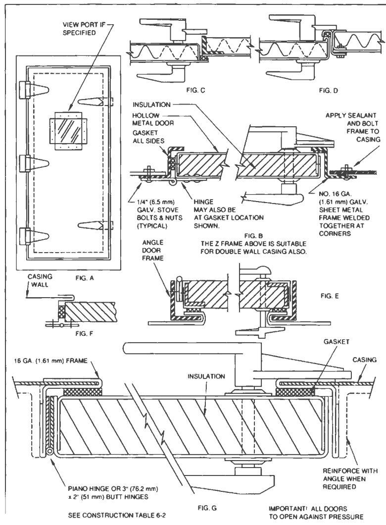
FIG. 6-11 CASING ACCESS DOORS - 2" W.G. (500 Pa)
