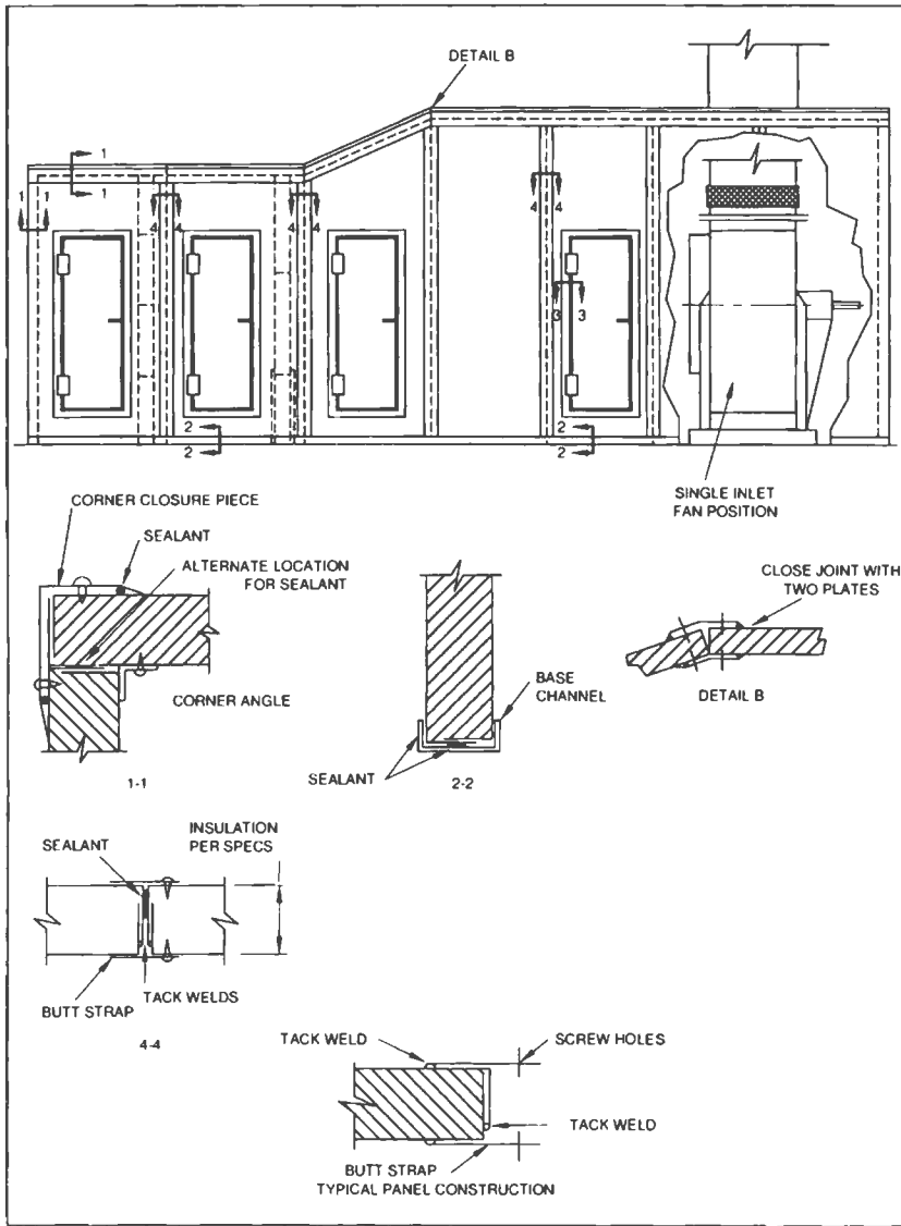
FIG. 6-7 DOUBLE WALL CASING
