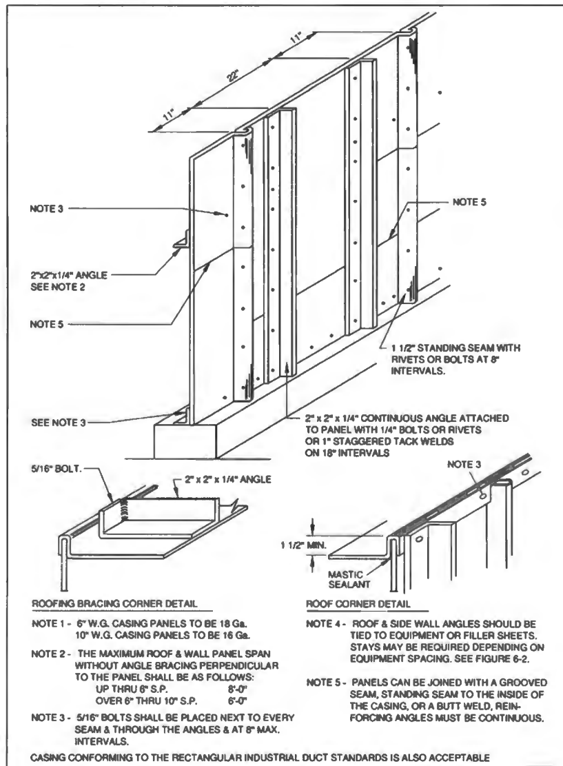
FIG. 6-5 OVER 2" W.G. PRESSURE APPARATUS CASING
