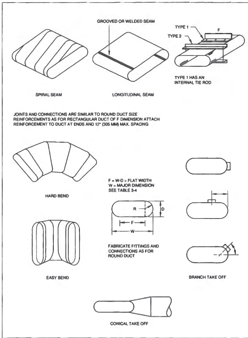
FIG. 3-6 FLAT OVAL DUCTS
