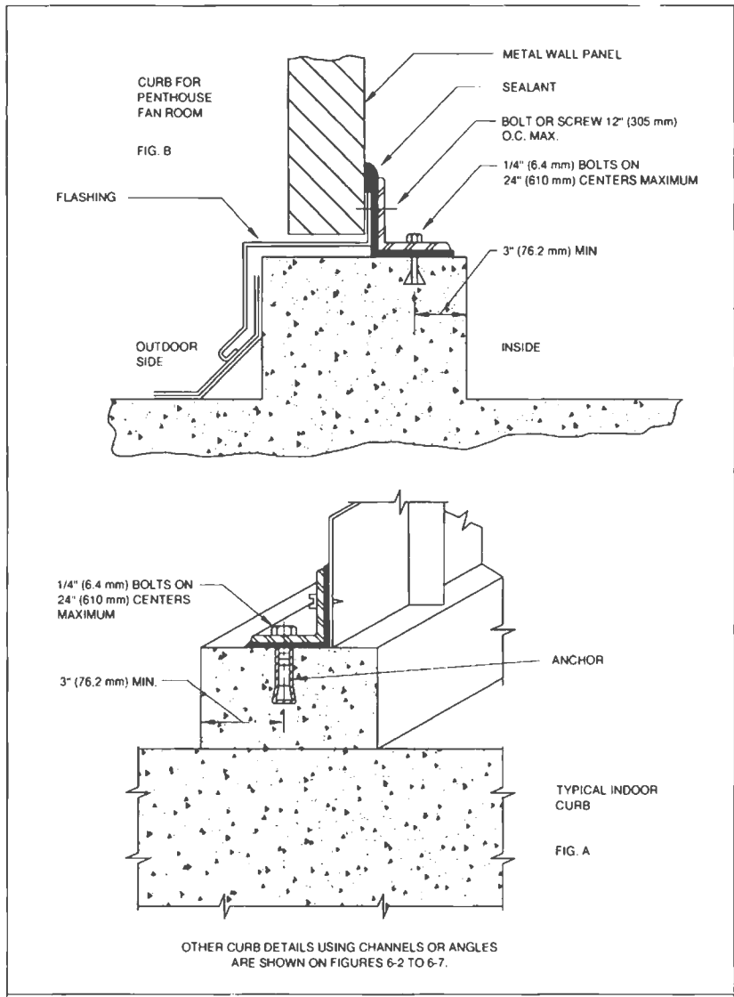
FIG. 6-8 CURB DETAIL
