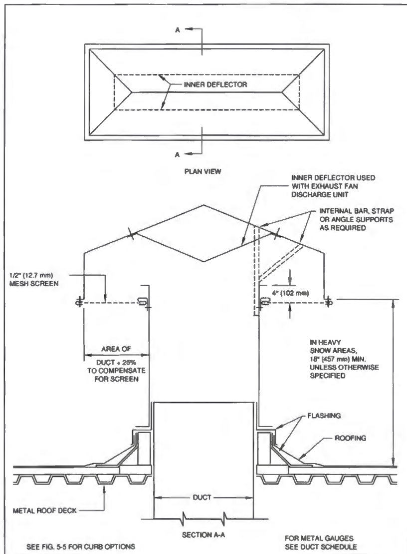
FIG. 5-7 LARGE INTAKE OR EXHAUST VENTILATORS
