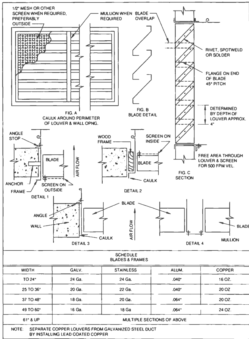
FIG. 5-1 LOUVERS AND SCREENS
