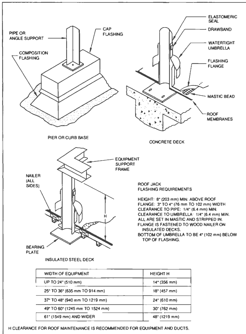
FIG. 5-4 EQUIPMENT AND DUCT SUPPORT FLASHING
