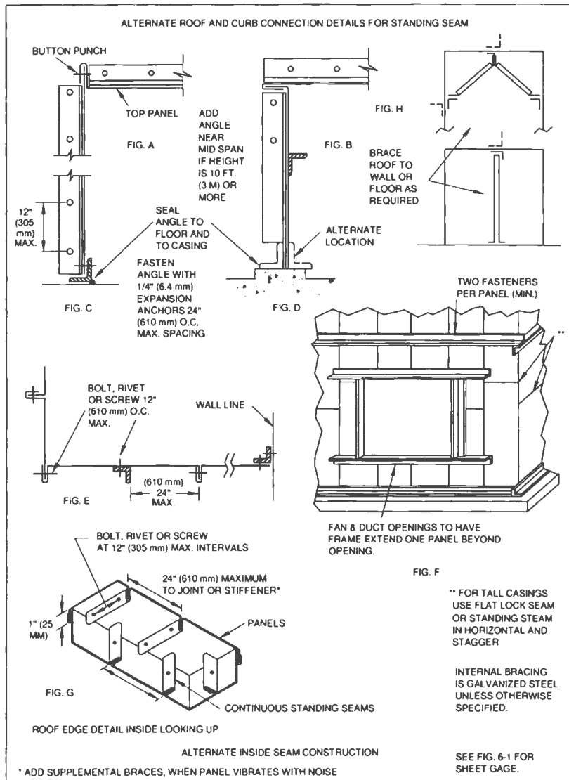
FIG. 6-2 STANDING SEAM CASINGS
