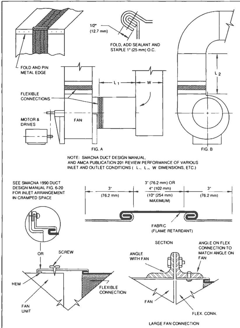
FIG. 2-17 FLEXIBLE CONNECTIONS AT FAN
