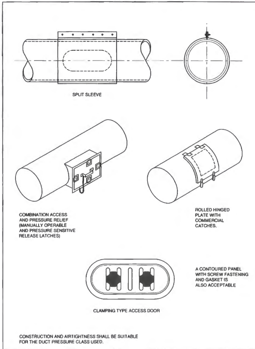
FIG. 2-11 ACCESS DOORS - ROUND DUCT
