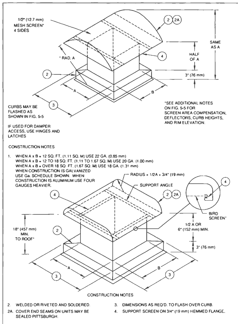
FIG. 5-6 INTAKE OR EXHAUST VENTILATORS
