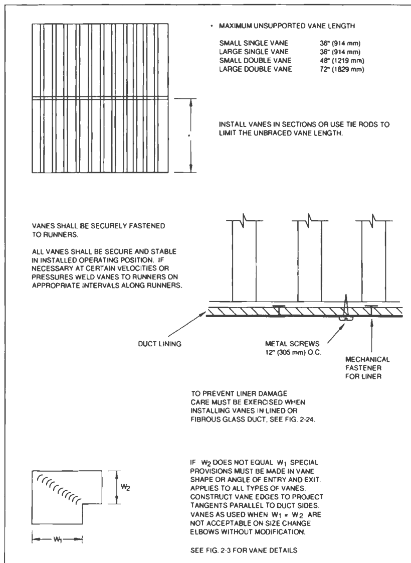
FIG. 2-4 VANE SUPPORT IN ELBOWS
