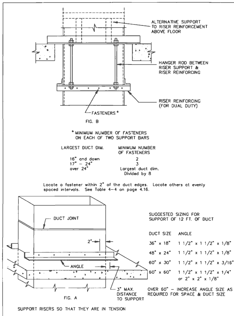
FIG. 4-7 RISER SUPPORTS - FROM FLOOR
