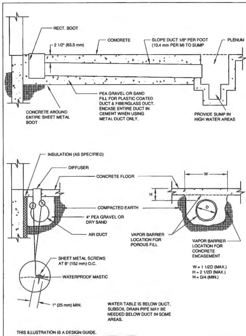
FIG. 3-11 TYPICAL UNDERSLAB DUCT
