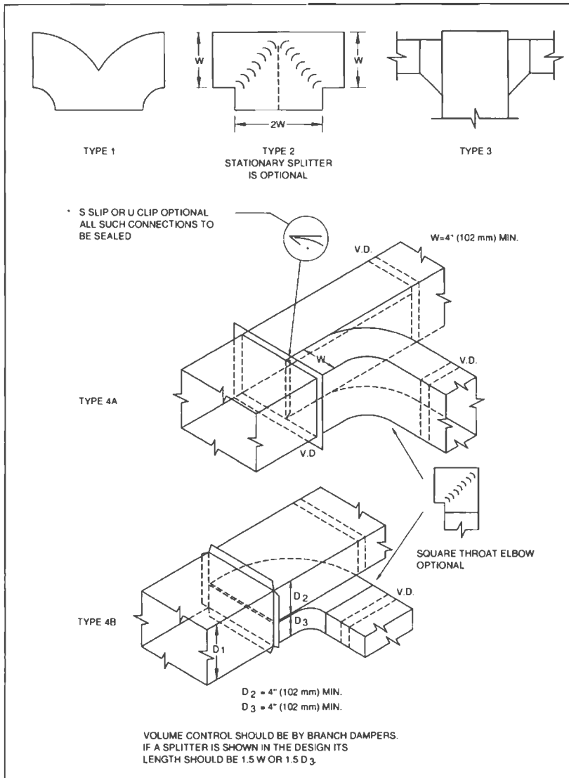
FIG. 2-5 DIVIDED FLOW BRANCHES
