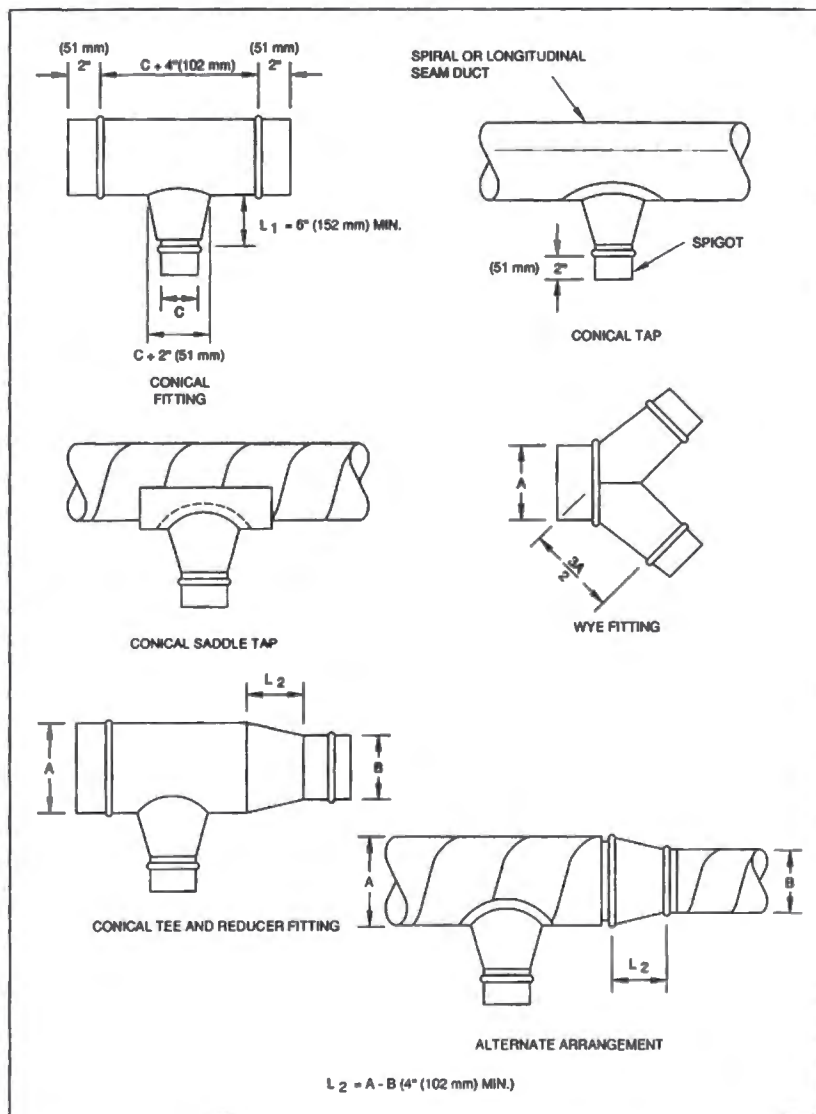
FIG. 3-5 CONICAL TEES
