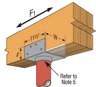
Typical LCC25-3.5 Installation connecting a 3-ply LVL and a 3½" diameter (O.D.) steel column
