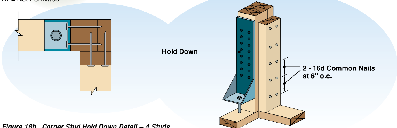
Figure 18b. Corner Stud Hold Down Detail – 4 Studs
