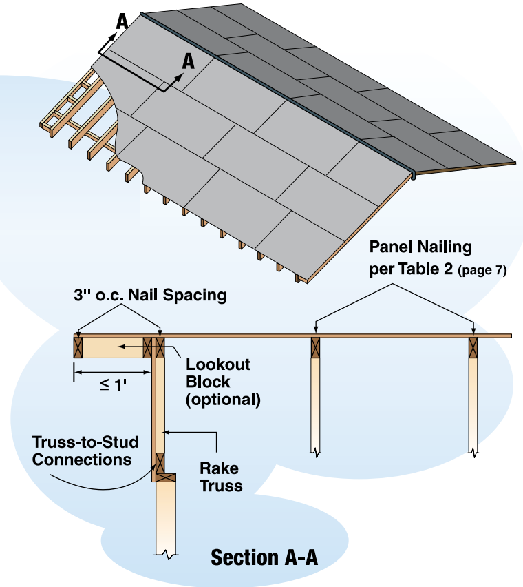
Figure 16. Rake Truss
