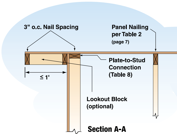
Figure 15. Full-Height Gable Endwall Stud
