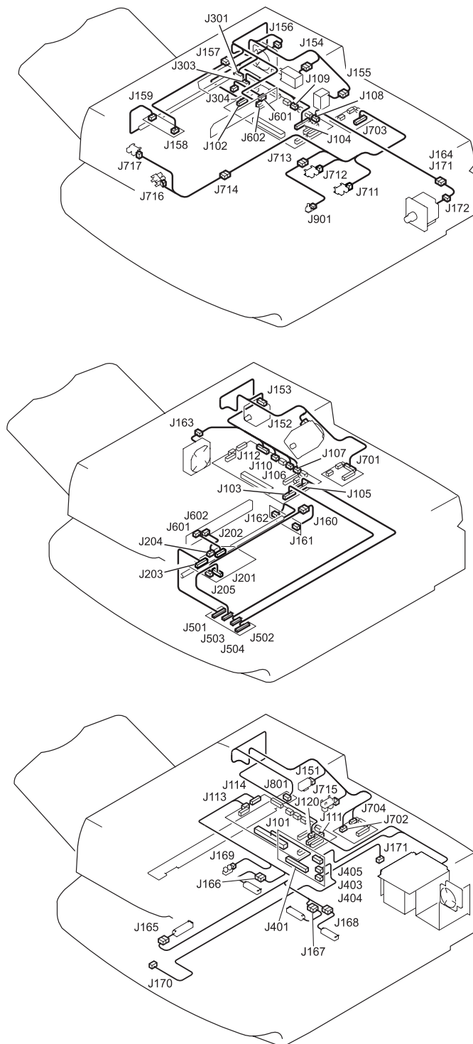
Figure 229. Connector locations
