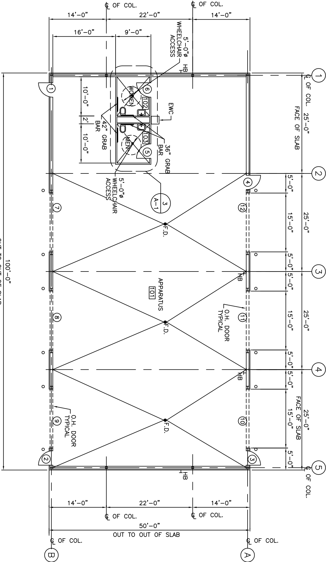
OUT TO OUT OF SLAB FLOOR PLAN SCALE: 1/8" = 1'-0"
